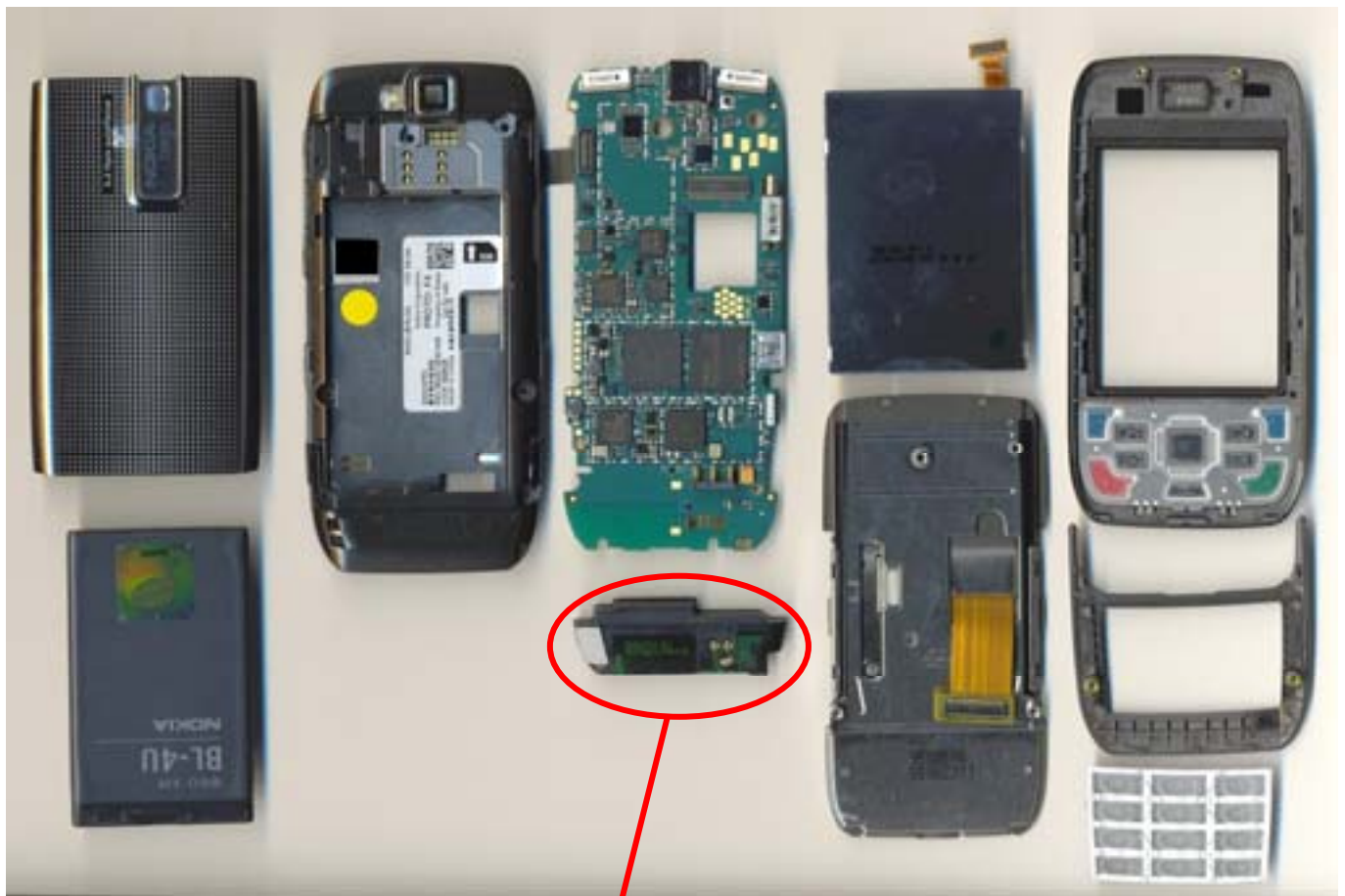
GSM/ WCDMA ANTENNA
