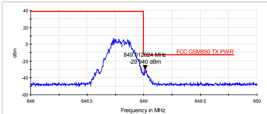
EGPRS, channel 251 / 848.8 MHz (Peak detector, RBW: 3 kHz)
