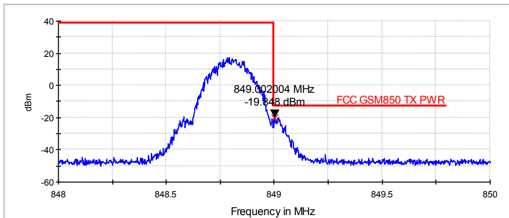
GSM, channel 251 / 848.8 MHz (Peak detector, RBW: 3 kHz)
