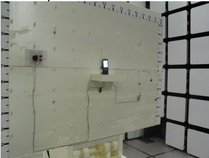
Picture 2 Spurious radiated emission measurement
