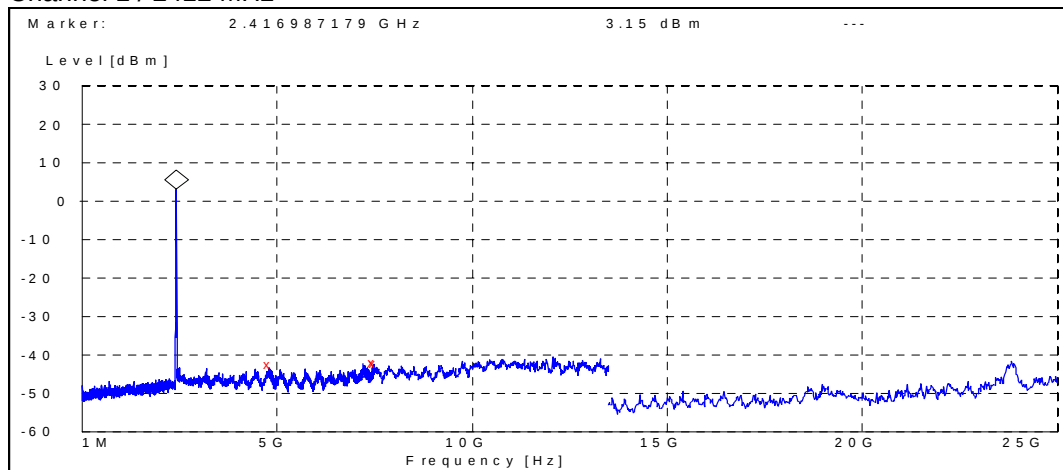
Channel 1 / 2412 MHz
