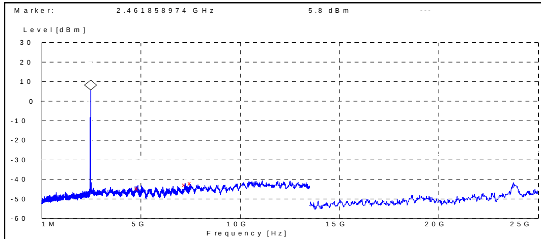
Channel 11 / 2462 MHz
