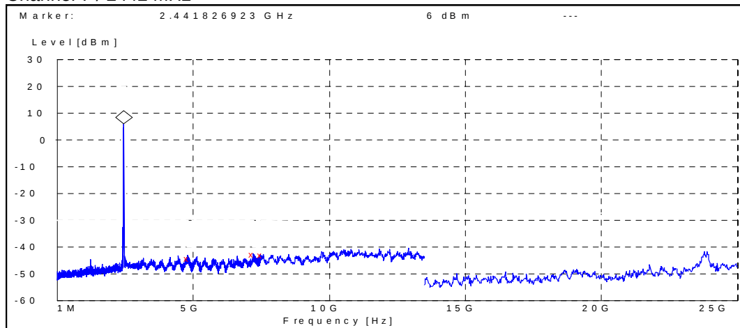
Channel 7 / 2442 MHz
