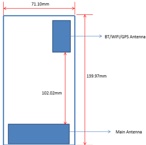
Phone Dimension and Distance Between Main antenna and BT/WiFi/GPS
