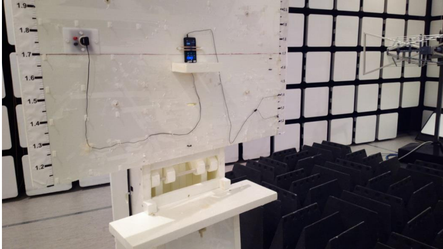
Picture 2. FCC Part 15B Radiated emissions
