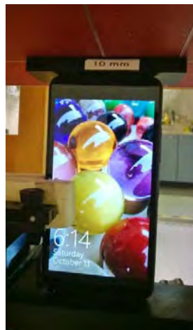
Photo of the device positioned for WR mode measurement – top edge facing phantom. The spacer was removed before the start of the measurements.
