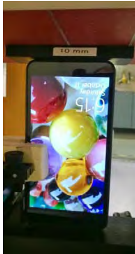
Photo of the device positioned for WR mode measurement – bottom edge facing phantom. The spacer was removed before the start of the measurements.
