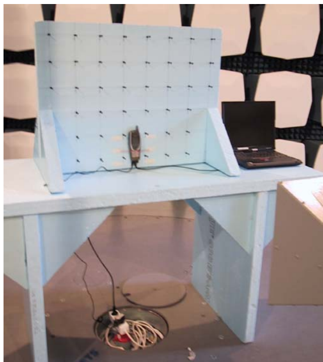
Picture 2: Radiated emission test setup.
