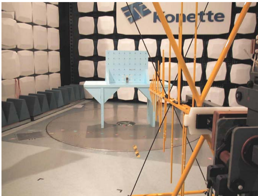
Picture 2: Radiated emission test setup for below 1 GHz frequencies
