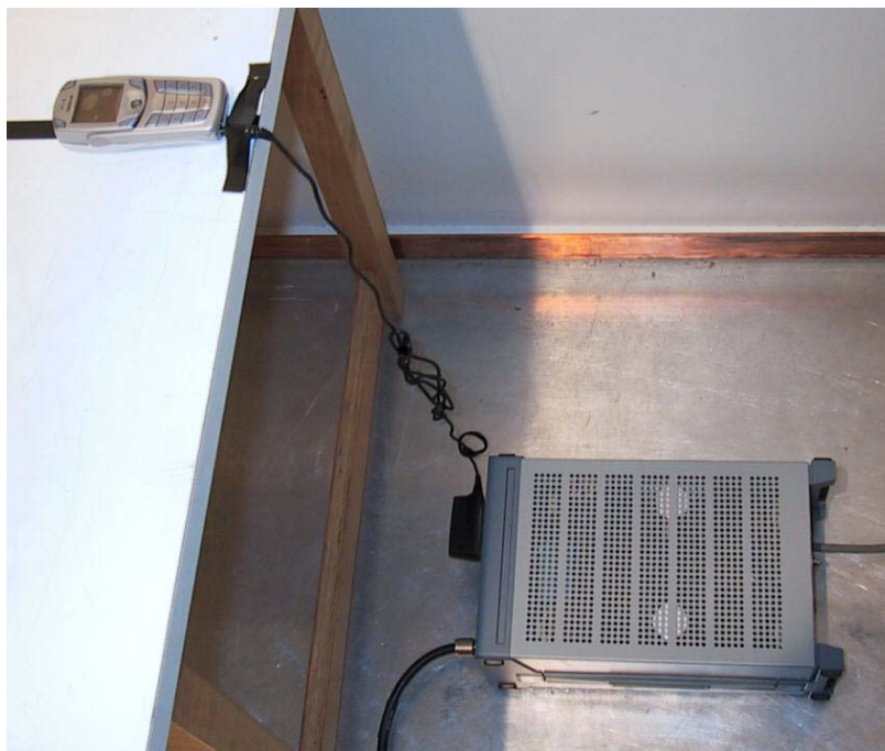
Picture 2: AC-power line conducted emissions test setup
