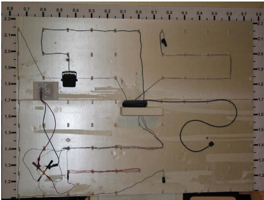
Picture 1 Spurious radiated emission measurement
