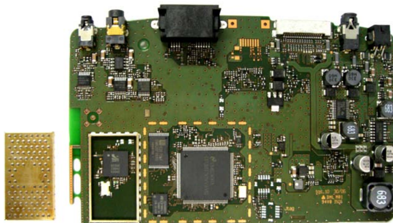
Top view of PWB without shielding
