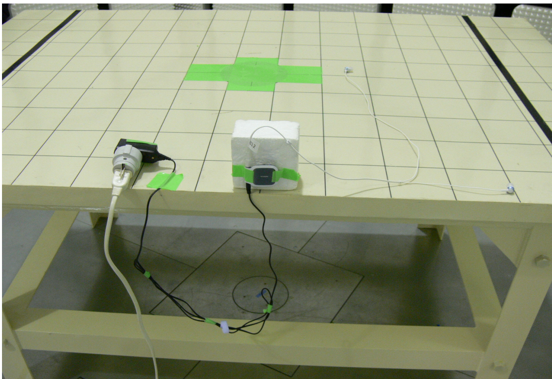
Photograph 3: Set-up for Radiated Emission, EUT Configuration Y-Axis
