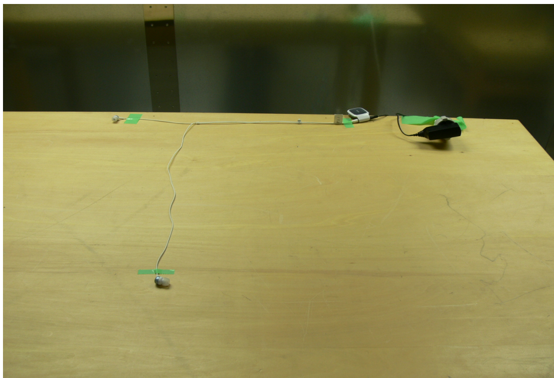
Photograph 5: Set-up for AC Mains Conducted Emission of Transmitter, Front View
