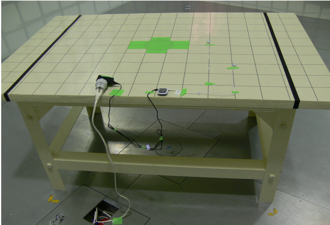
Photograph 2: Set-up for Radiated Emission, EUT Configuration X-Axis
