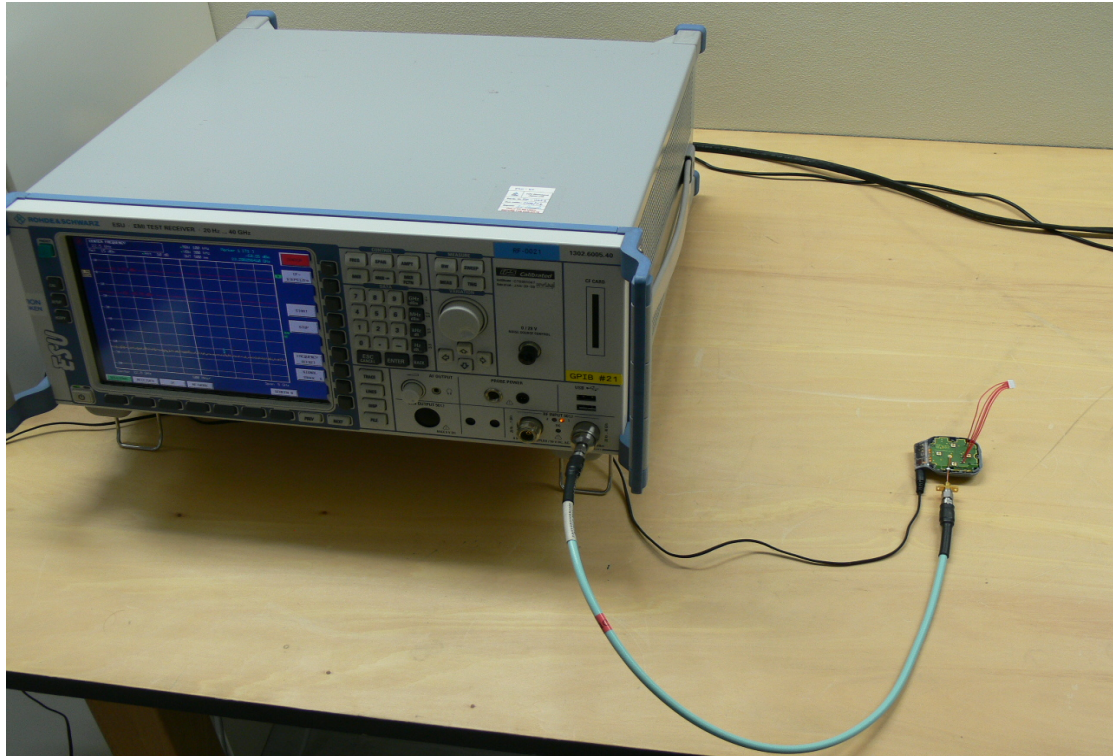
Photograph 1: Set-up for Conducted Emissions at Antenna Port
