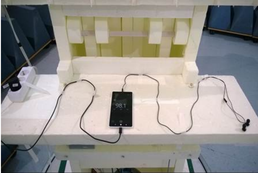
Picture 3. FCC Part 15B Radiated emissions
