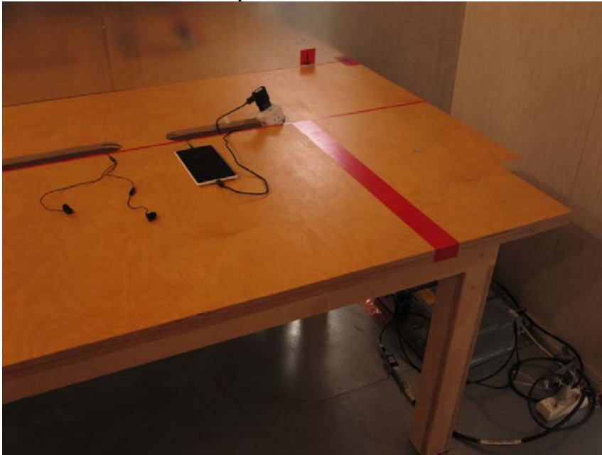
Picture 4. FCC Part 15C AC powerline conducted emissions
