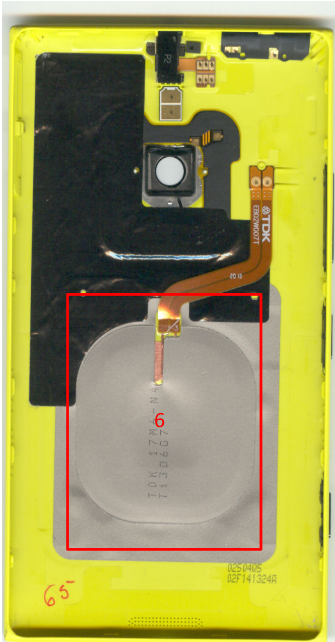
7) Wireless charging (WLC) back cover.
