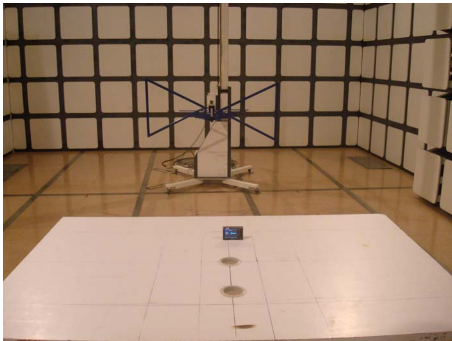
(2) Radiated Emission Test Setup Photo
