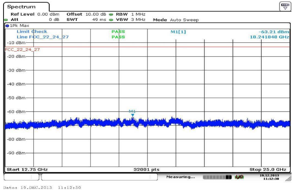
Plot 3: Channel 1412 (12.75 GHz – 25 GHz)
