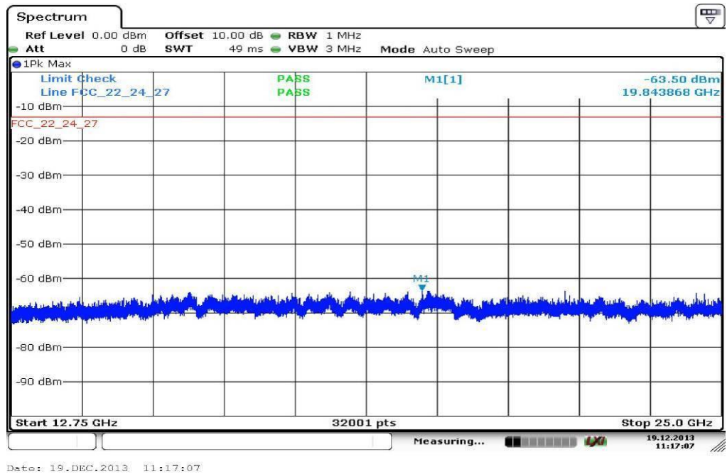
Plot 3: Channel 661 (12.75 GHz - 25 GHz)
