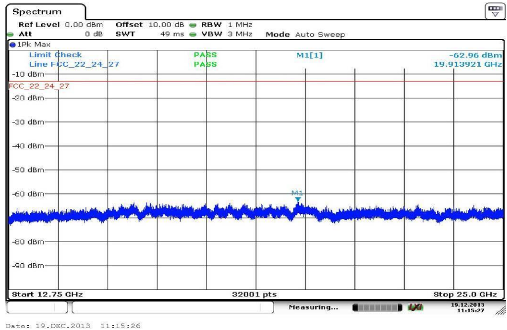
Plot 3: Channel 9400 (12.75 GHz - 25 GHz)
