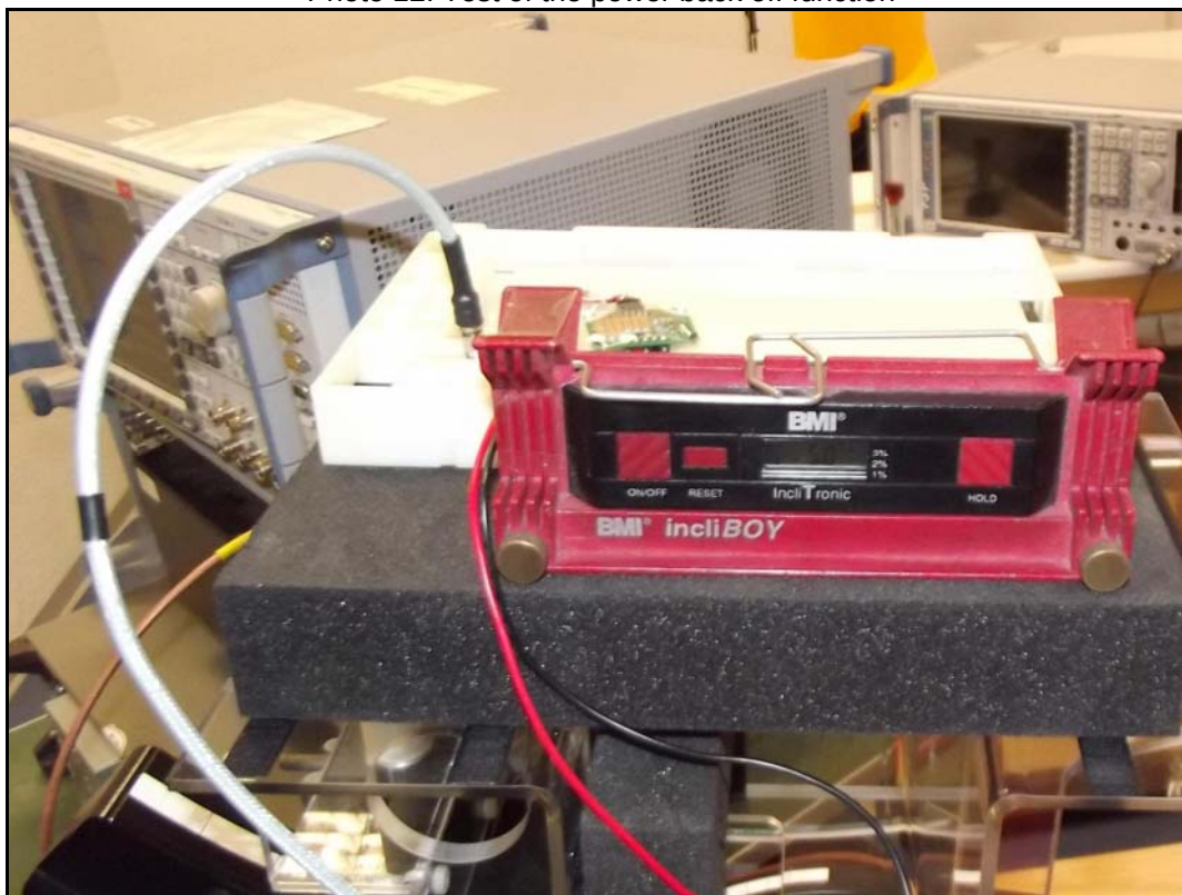
Photo 12: Test of the power back off function
