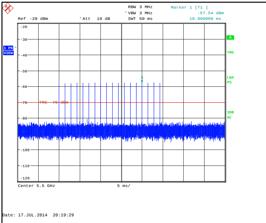
Type 0 Radar
