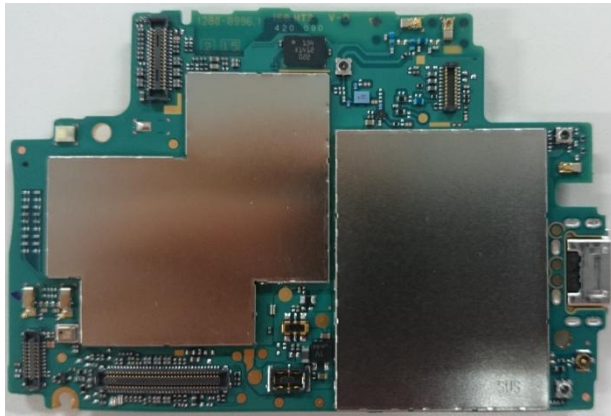
Internal PWB with Shield cases (Rear-side)
