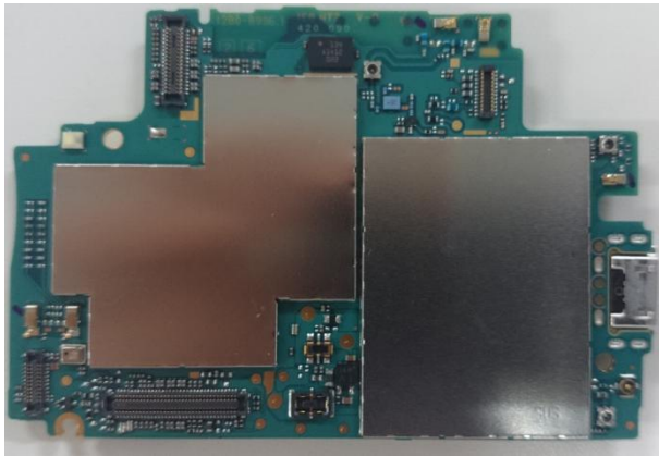
Internal PWB with Shield cases (Rear-side)
