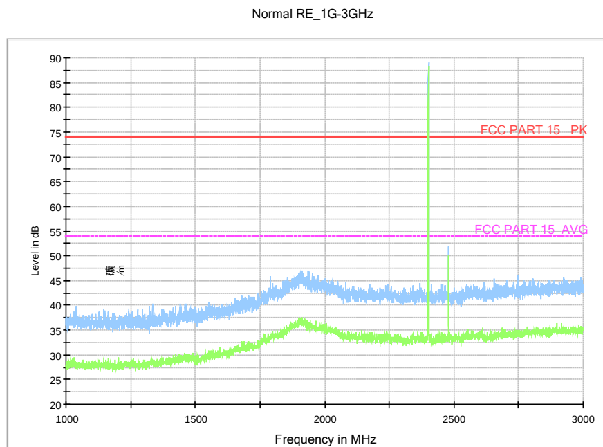
Fig.68. Radiated emission: \pi/4 DQPSK, Channel 0, 1 GHz - 3 GHz
