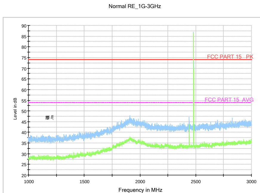
Fig.73. Radiated emission: \pi/4 DQPSK, Channel 78, 1 GHz - 3 GHz
