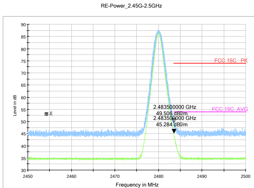
Fig.86. Radiated emission (Power): 8DPSK, high channel
