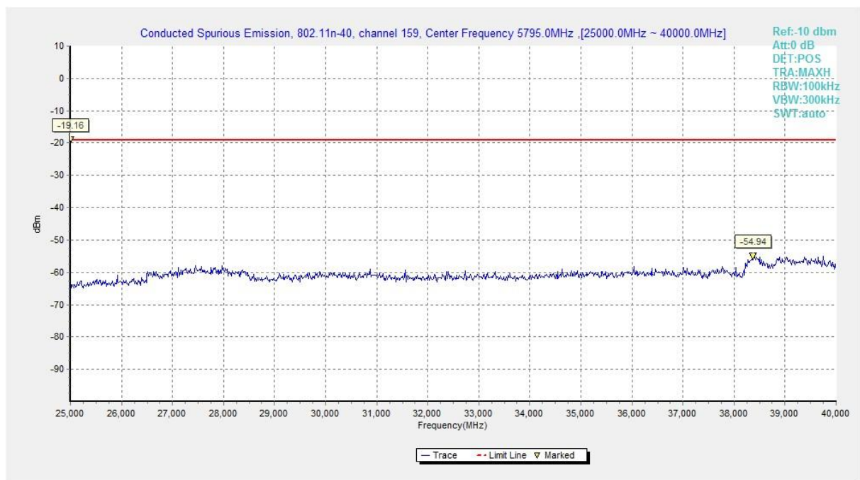
Fig. 48 Conducted Spurious Emission (802.11n-HT40, Ch159, 25 GHz-40 GHz)
