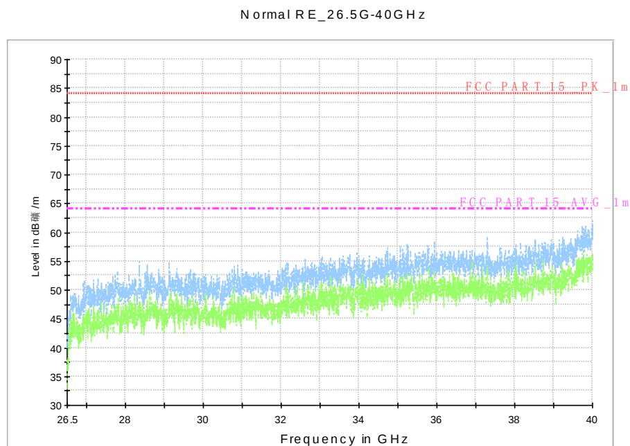
Fig. 82 Radiated Spurious Emission (802.11n-HT40, Ch151, 26.5 GHz - 40 GHz)
