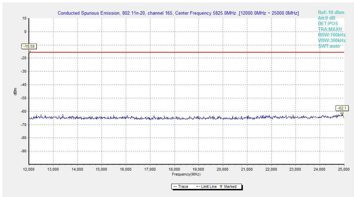
Fig. 39 Conducted Spurious Emission (802.11n-HT20, Ch165, 12 GHz-25 GHz)
