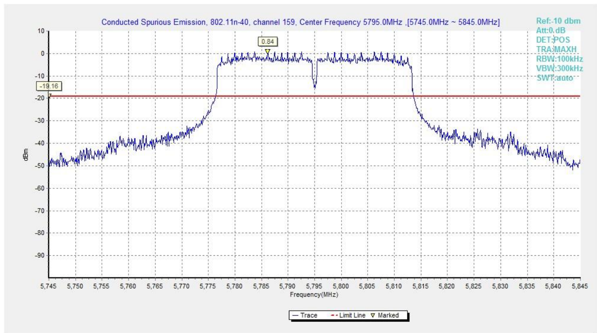
Fig. 45 Conducted Spurious Emission (802.11n-HT40, Ch159, Center Frequency)
