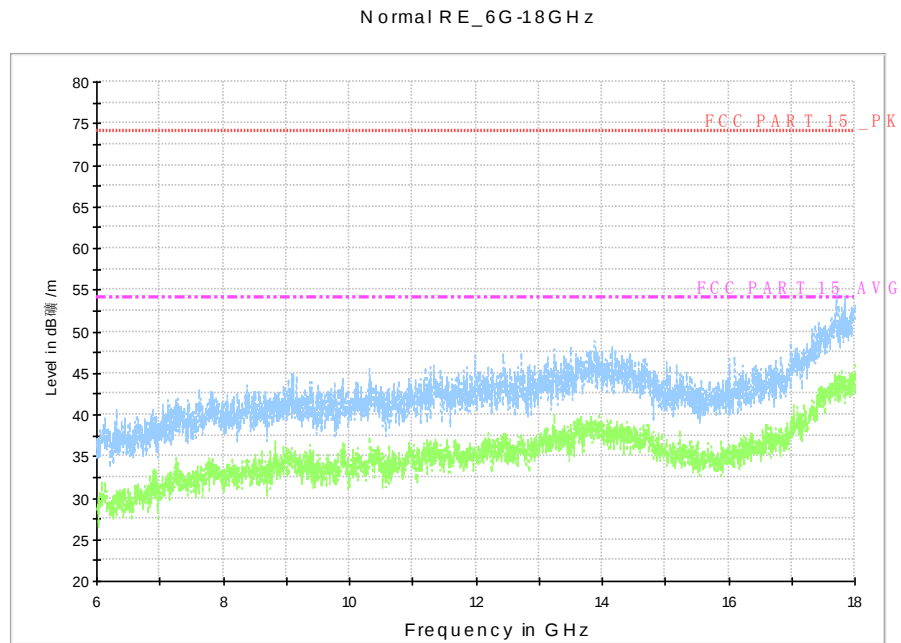
Fig. 69 Radiated Spurious Emission (802.11n-HT20, Ch157, 6 GHz-18 GHz)
