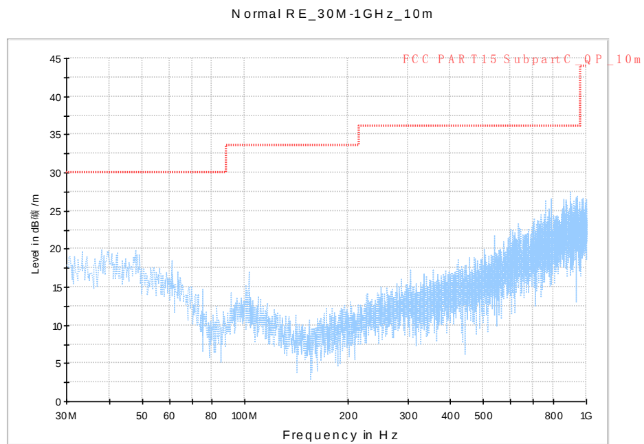
Fig. 83 Radiated Spurious Emission (802.11ac-HT80, Ch155, 30 MHz-1 GHz)
