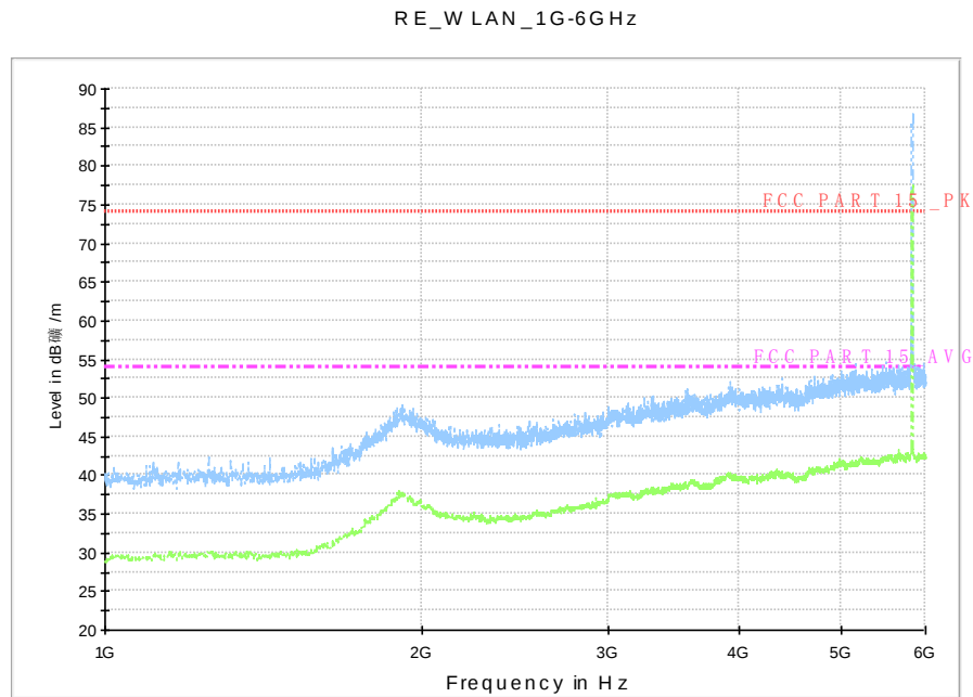
Fig. 71 Radiated Spurious Emission (802.11n-HT20, Ch165, 1 GHz-6 GHz)
