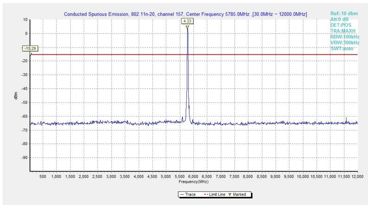
Fig. 34 Conducted Spurious Emission (802.11n-HT20, Ch157, 30 MHz-12 GHz)
