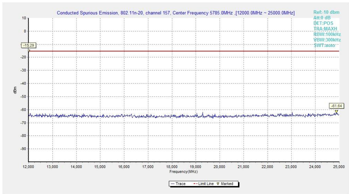
Fig. 35 Conducted Spurious Emission (802.11n-HT20, Ch157, 12 GHz-25 GHz)
