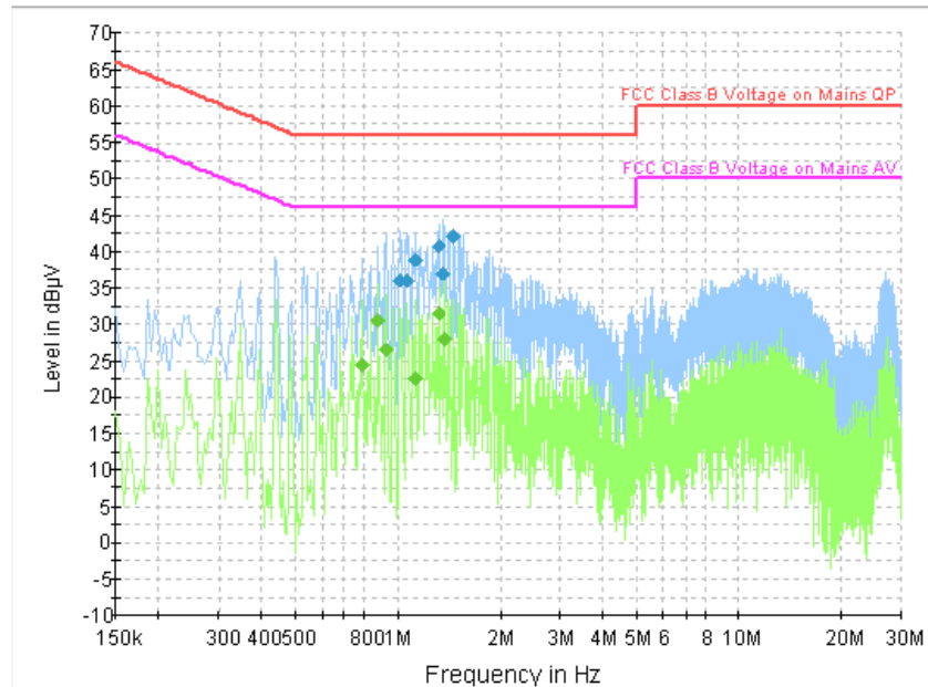
Fig. 88 AC Powerline Conducted Emission-802.11a
