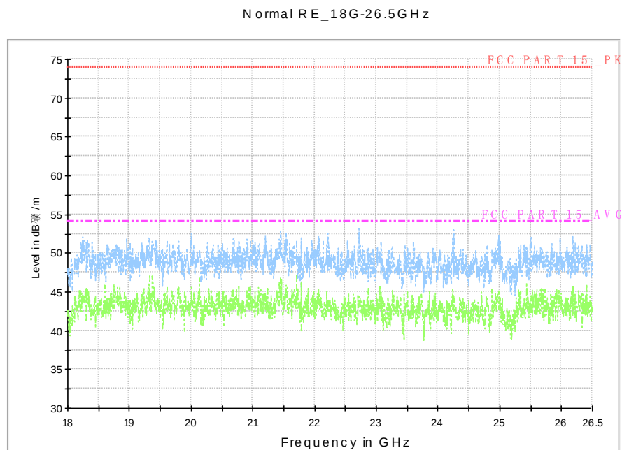
Fig. 81 Radiated Spurious Emission (802.11n-HT40, Ch151, 18 GHz-26.5 GHz)
