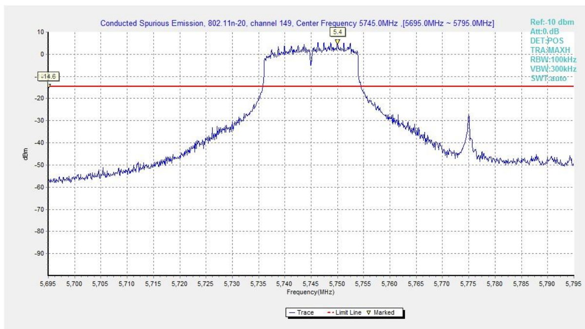
Fig. 29 Conducted Spurious Emission (802.11n-HT20, Ch149, Center Frequency)
