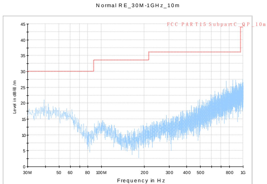
Fig. 53 Radiated Spurious Emission (802.11a, Ch149, 30 MHz-1 GHz)
