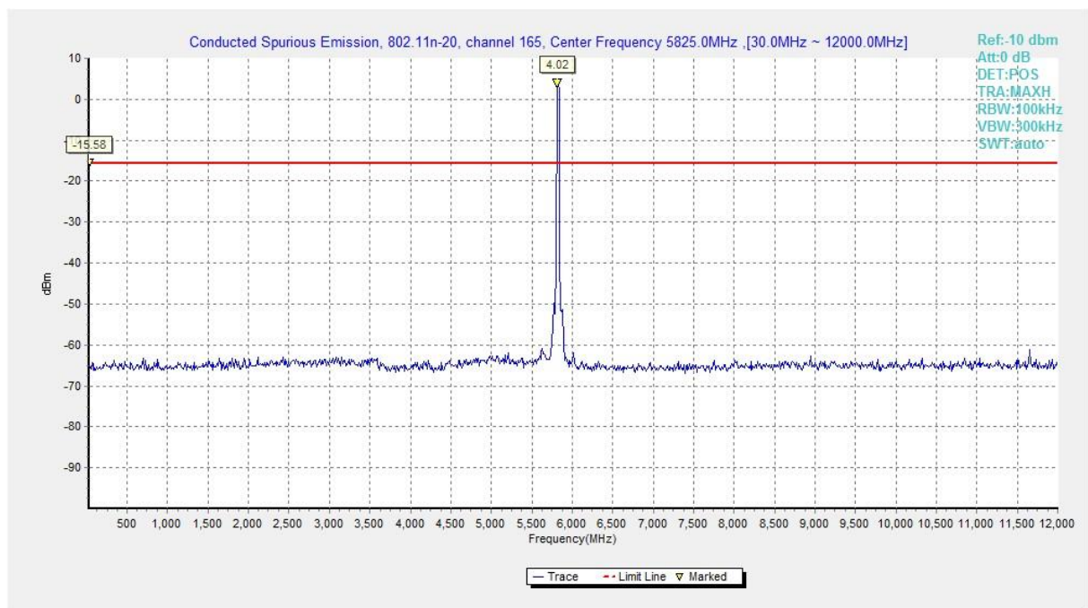
Fig. 38 Conducted Spurious Emission (802.11n-HT20, Ch165, 30 MHz-12 GHz)
