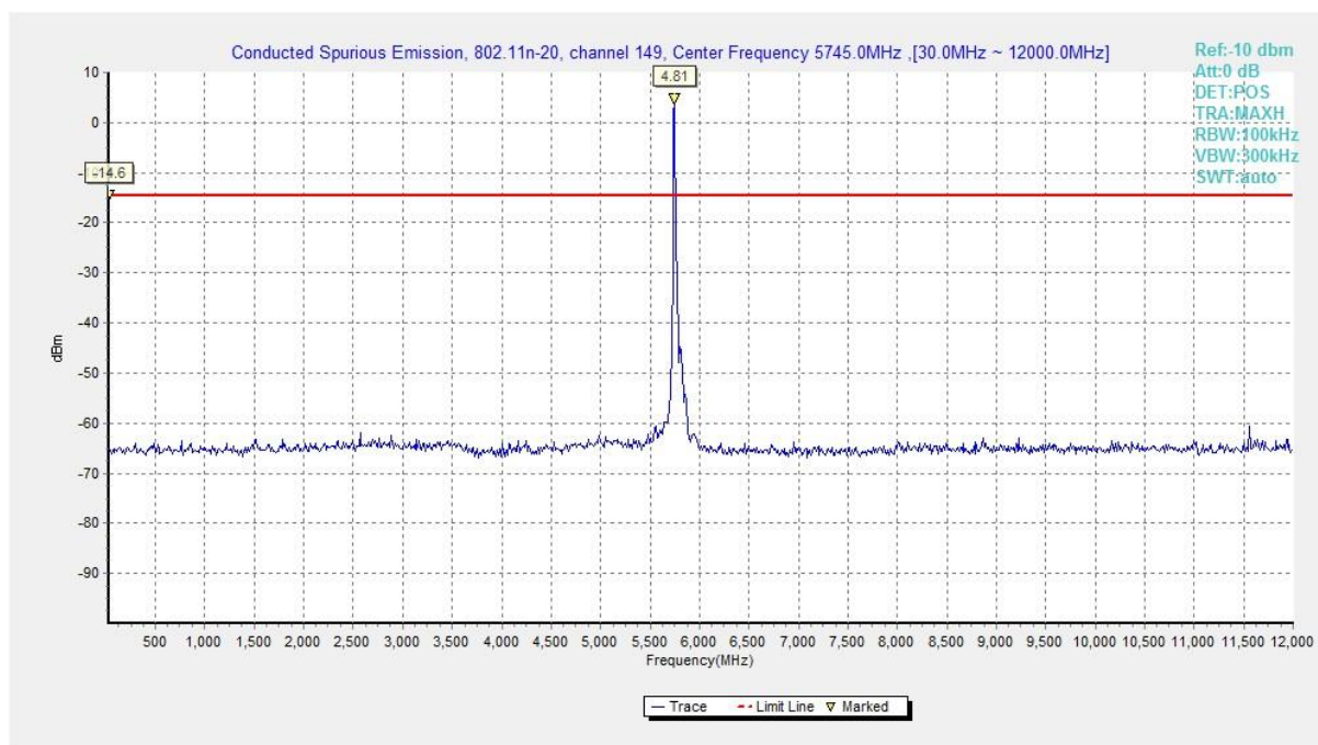
Fig. 30 Conducted Spurious Emission (802.11n-HT20, Ch149, 30 MHz-12 GHz)
