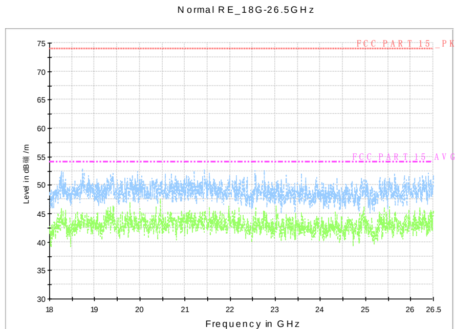
Fig. 86 Radiated Spurious Emission (802.11ac-HT80, Ch155, 18 GHz-26.5 GHz)
