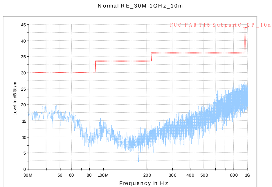
Fig. 75 Radiated Spurious Emission (802.11n-HT40, Ch151, 30 MHz-1 GHz)
