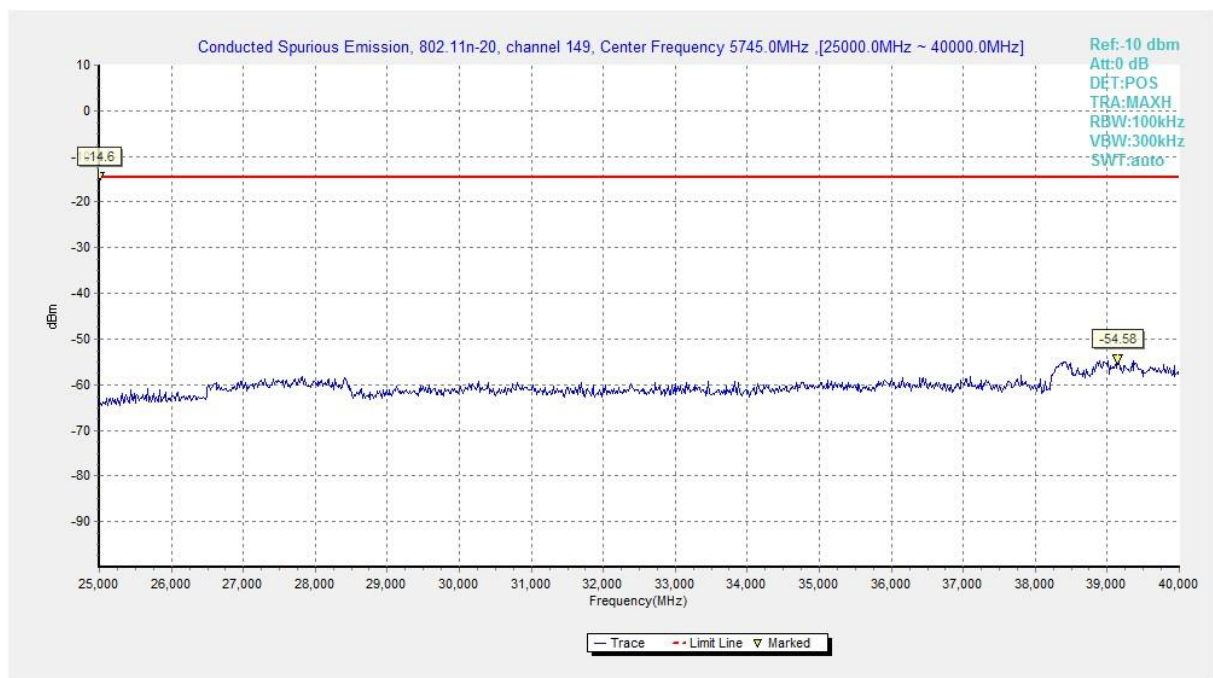
Fig. 32 Conducted Spurious Emission (802.11n-HT20, Ch149, 25 GHz-40 GHz)
