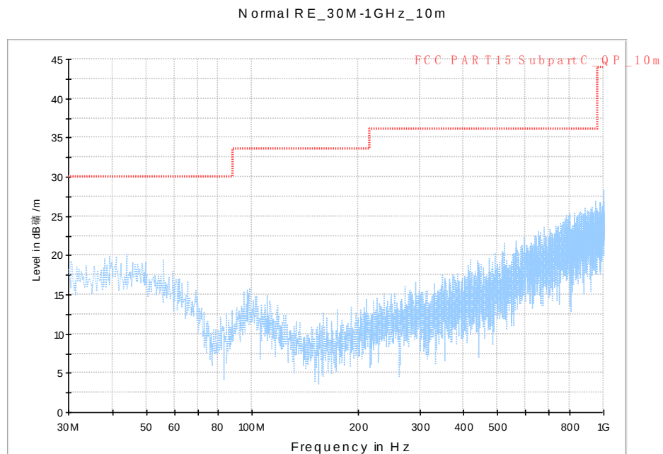
Fig. 70 Radiated Spurious Emission (802.11n-HT20, Ch165, 30 MHz-1 GHz)
