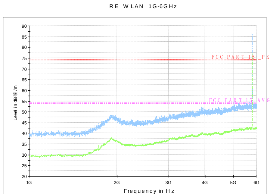
Fig. 68 Radiated Spurious Emission (802.11n-HT20, Ch157, 1 GHz-6 GHz)
