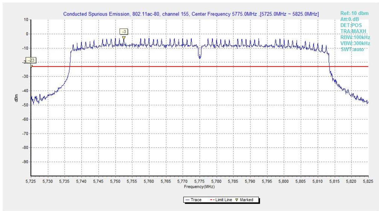
Fig. 49 Conducted Spurious Emission (802.11ac-HT80, Ch155, Center Frequency)
