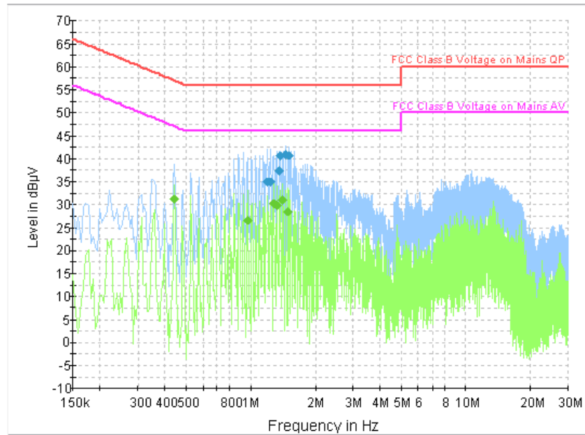
Fig. 89 AC Powerline Conducted Emission-Idle
