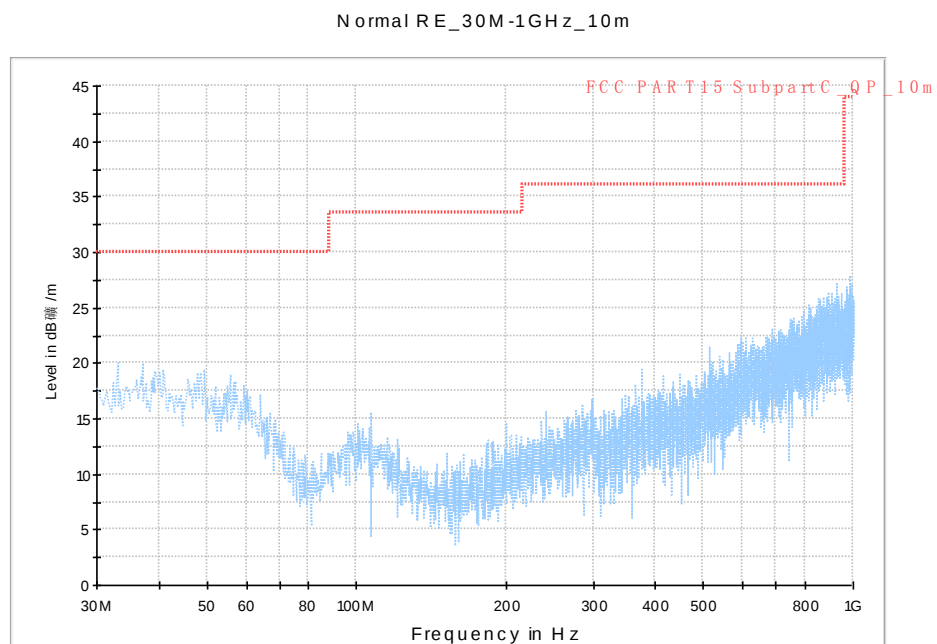
Fig. 56 Radiated Spurious Emission (802.11a, Ch157, 30 MHz-1 GHz)
