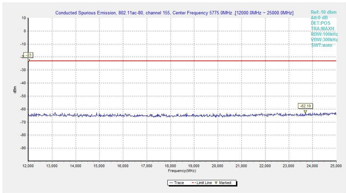
Fig. 51 Conducted Spurious Emission (802.11ac-HT80, Ch155, 12 GHz-25 GHz)
