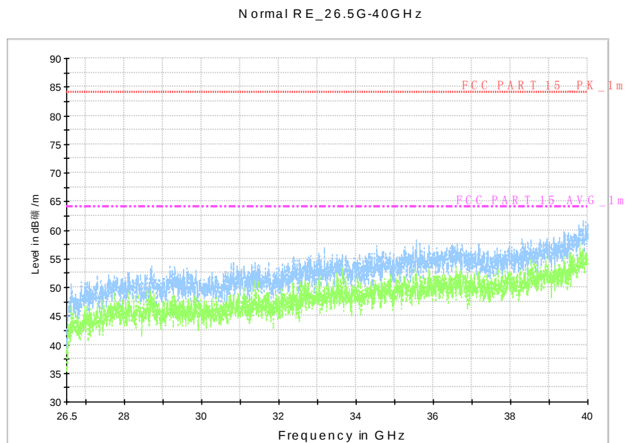
Fig. 63 Radiated Spurious Emission (802.11a, Ch157, 26.5 GHz - 40 GHz)
