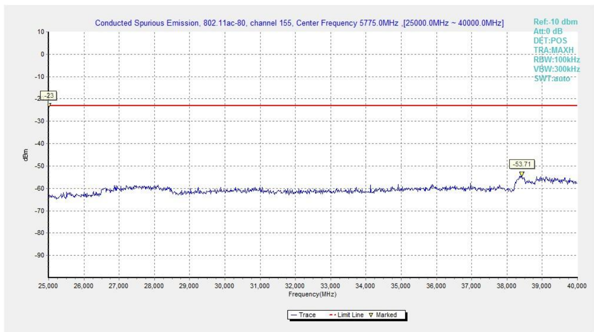
Fig. 52 Conducted Spurious Emission (802.11ac-HT80, Ch155, 25 GHz-40 GHz)
