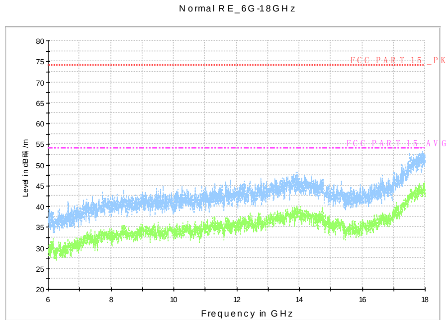
Fig. 77 Radiated Spurious Emission (802.11n-HT40, Ch151, 6 GHz-18 GHz)
