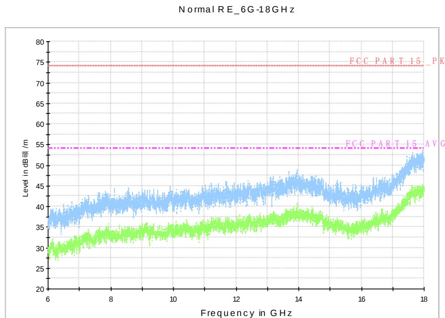
Fig. 66 Radiated Spurious Emission (802.11n-HT20, Ch149, 6 GHz-18 GHz)
