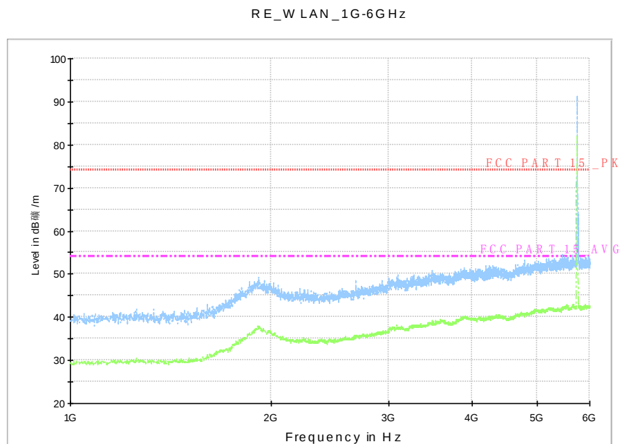
Fig. 54 Radiated Spurious Emission (802.11a, Ch149, 1 GHz-6 GHz)
