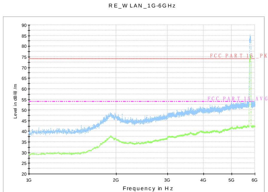
Fig. 84 Radiated Spurious Emission (802.11ac-HT80, Ch155, 1 GHz-6 GHz)
