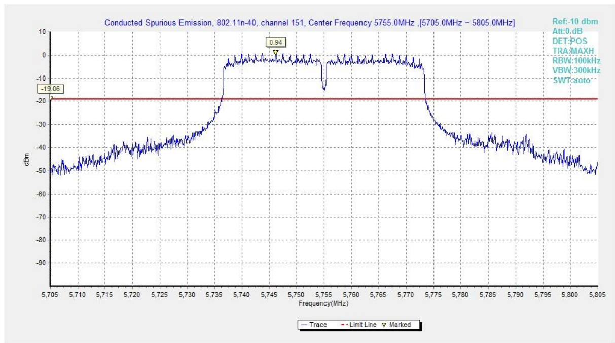
Fig. 41 Conducted Spurious Emission (802.11n-HT40, Ch151, Center Frequency)
