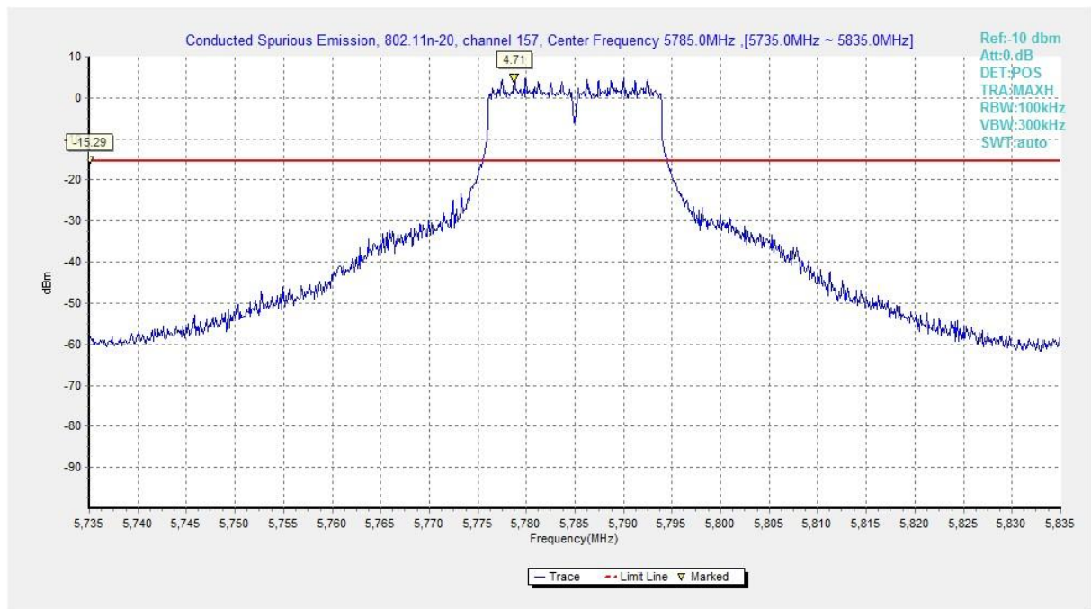
Fig. 33 Conducted Spurious Emission (802.11n-HT20, Ch157, Center Frequency)
