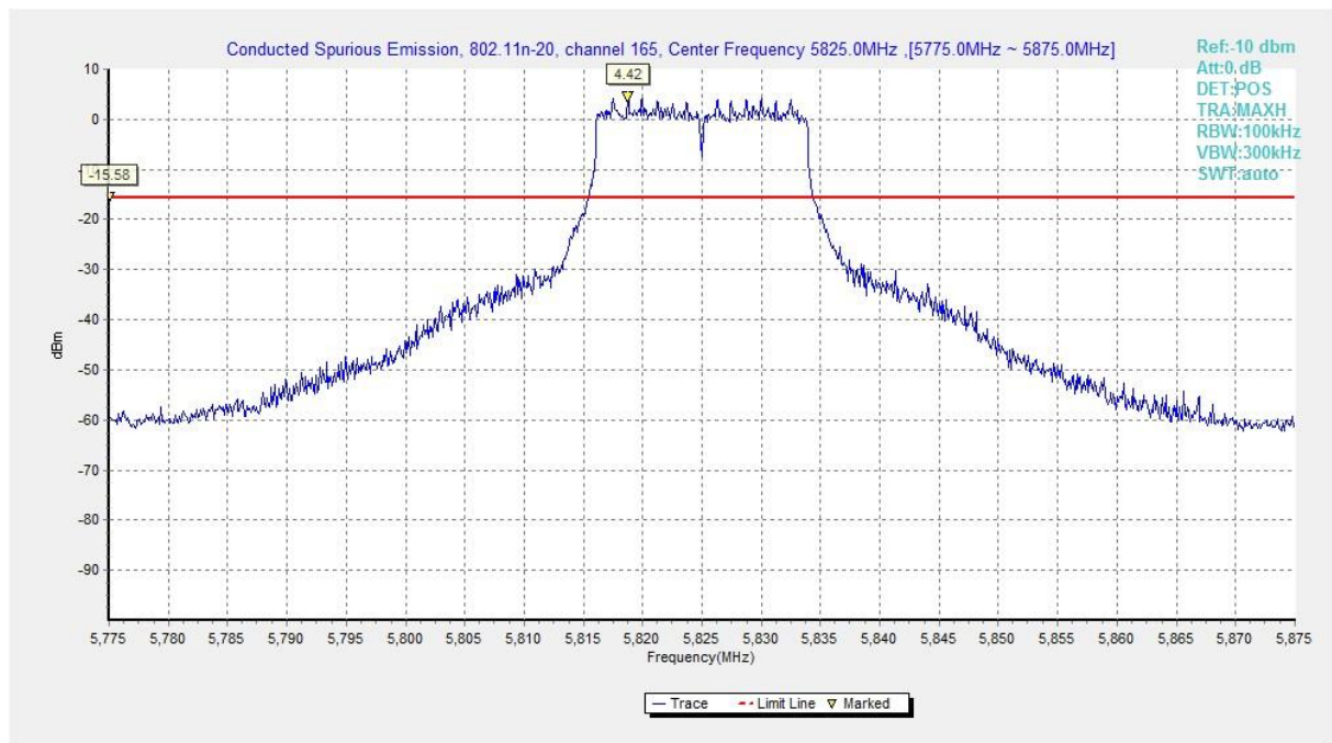
Fig. 37 Conducted Spurious Emission (802.11n-HT20, Ch165, Center Frequency)
