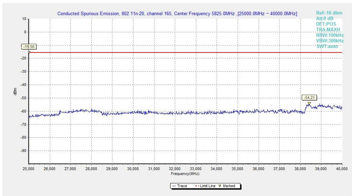
Fig. 40 Conducted Spurious Emission (802.11n-HT20, Ch165, 25 GHz-40 GHz)
