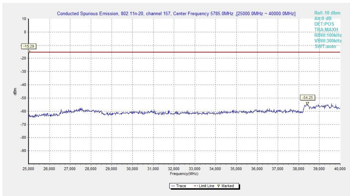
Fig. 36 Conducted Spurious Emission (802.11n-HT20, Ch157, 25 GHz-40 GHz)
