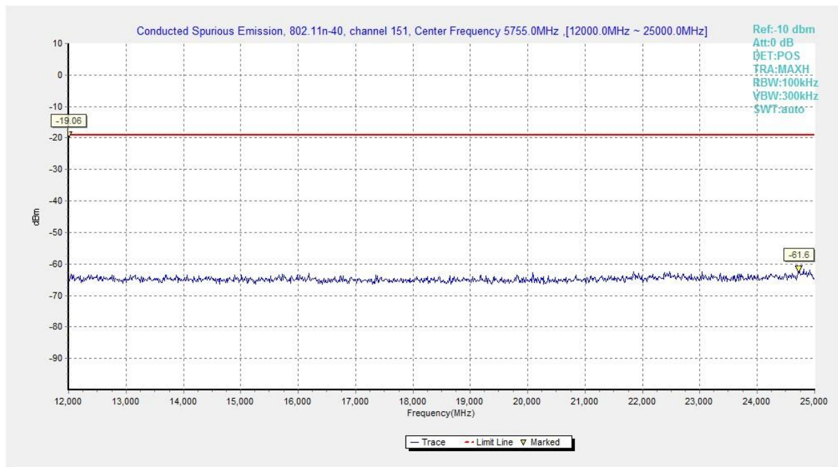
Fig. 43 Conducted Spurious Emission (802.11n-HT40, Ch151, 12 GHz-25 GHz)
