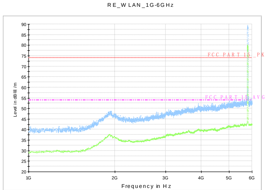
Fig. 79 Radiated Spurious Emission (802.11n-HT40, Ch159 1 GHz-6 GHz)
