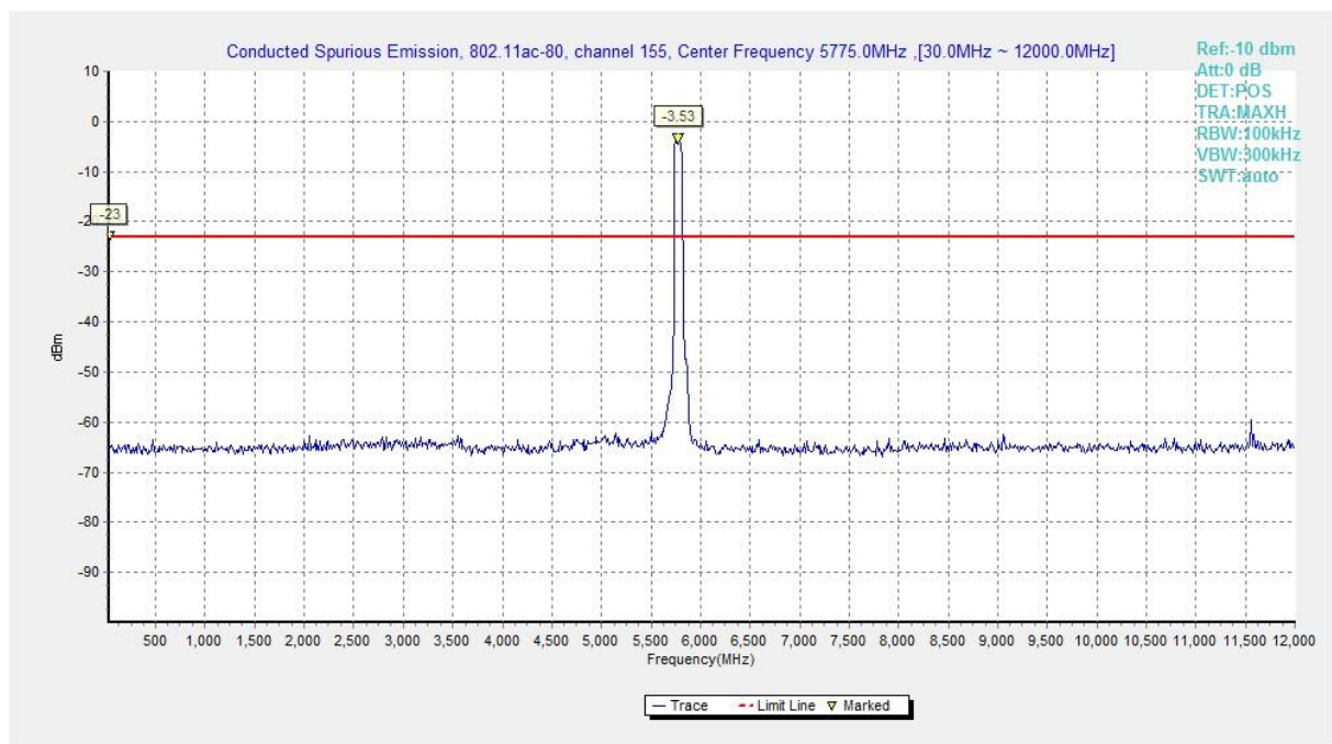
Fig. 50 Conducted Spurious Emission (802.11ac-HT80, Ch155, 30 MHz-12 GHz)
