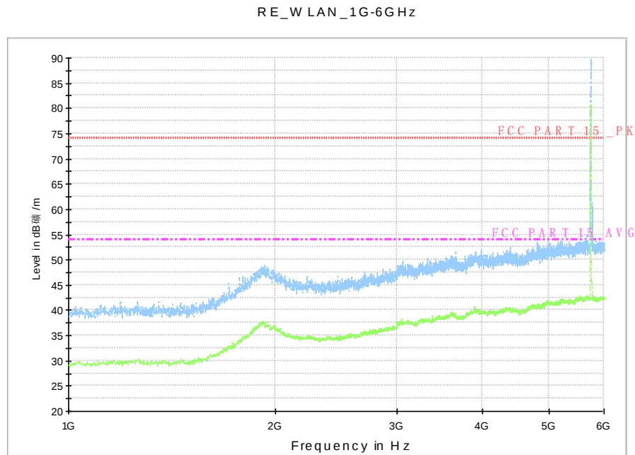
Fig. 65 Radiated Spurious Emission (802.11n-HT20, Ch149, 1 GHz-6 GHz)
