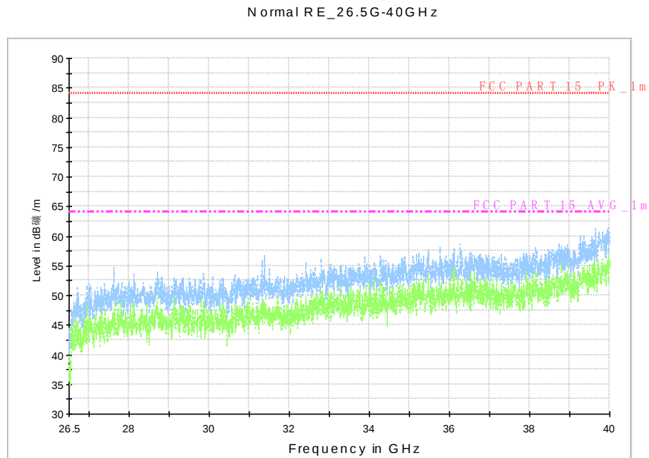
Fig. 87 Radiated Spurious Emission (802.11ac-HT80, Ch155, 26.5 GHz - 40 GHz)
