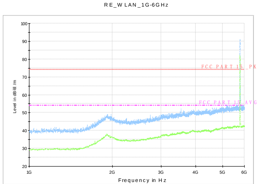
Fig. 57 Radiated Spurious Emission (802.11a, Ch157, 1 GHz-6 GHz)
