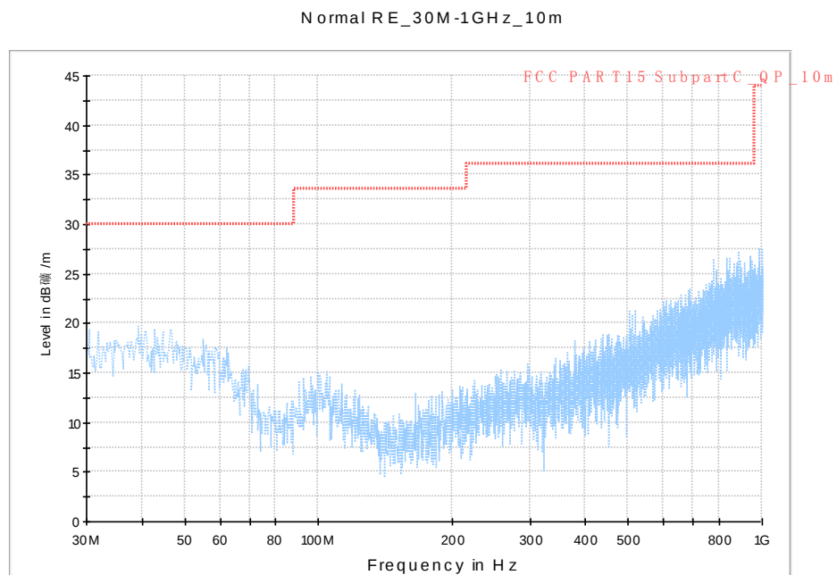
Fig. 59 Radiated Spurious Emission (802.11a, Ch165, 30 MHz-1 GHz)
