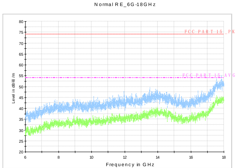
Fig. 85 Radiated Spurious Emission (802.11ac-HT80, Ch155, 6 GHz-18 GHz)
