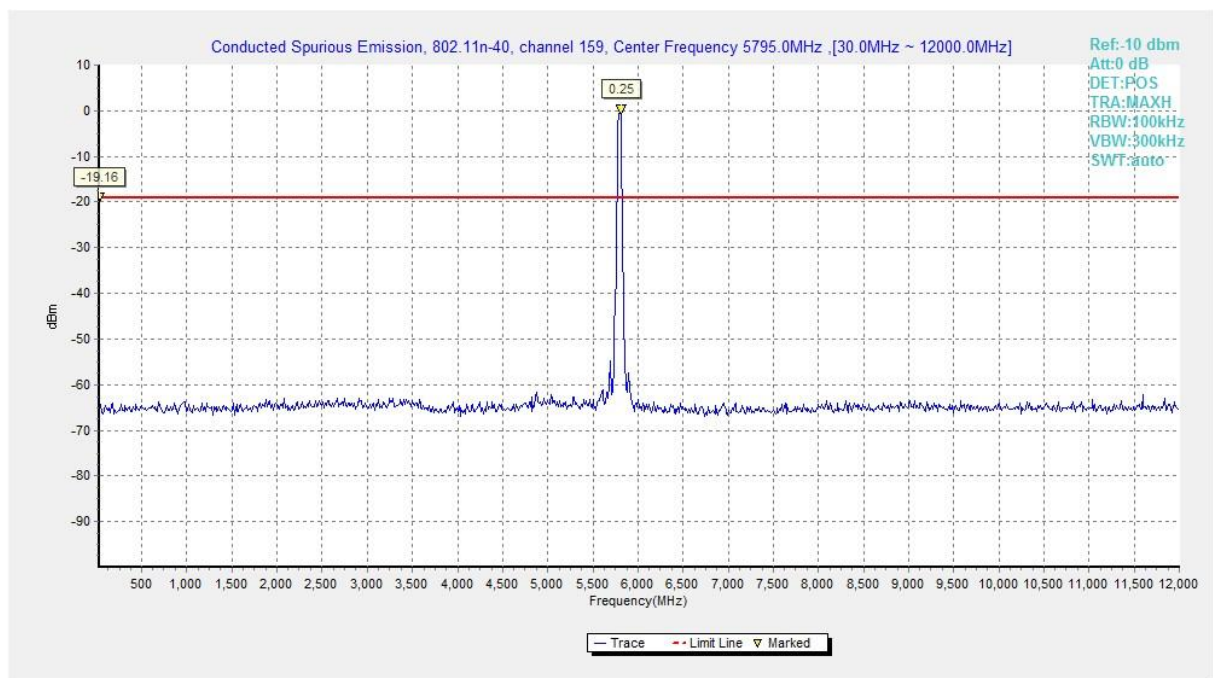
Fig. 46 Conducted Spurious Emission (802.11n-HT40, Ch159, 30 MHz-12 GHz)
