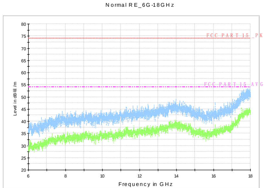
Fig. 55 Radiated Spurious Emission (802.11a, Ch149, 6 GHz-18 GHz)
