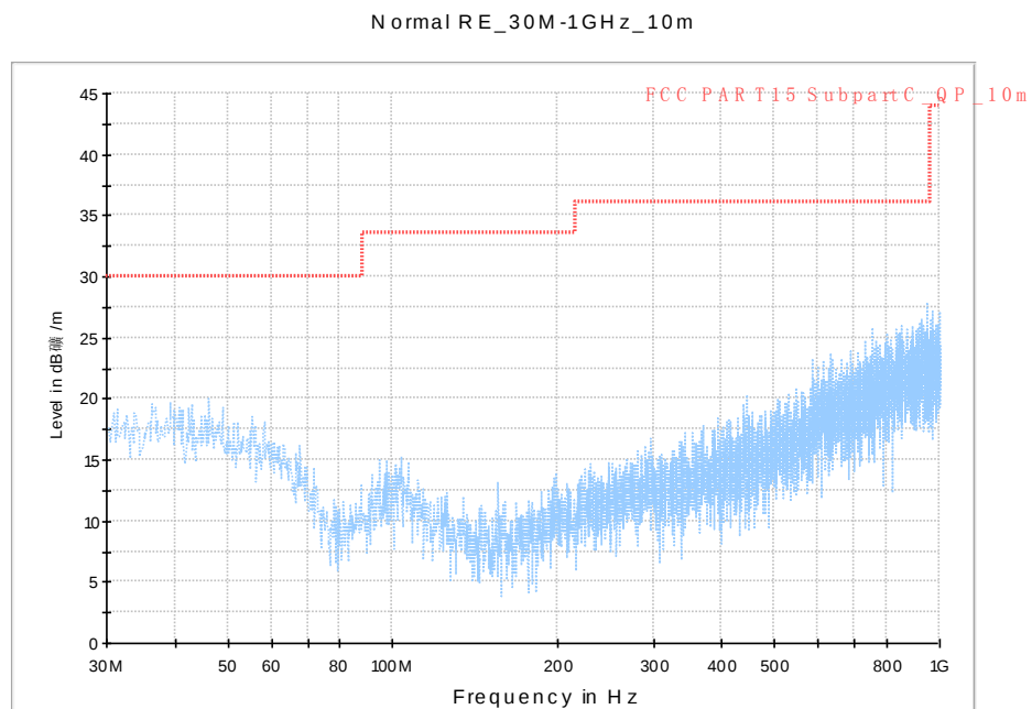
Fig. 67 Radiated Spurious Emission (802.11n-HT20, Ch157, 30 MHz-1 GHz)
