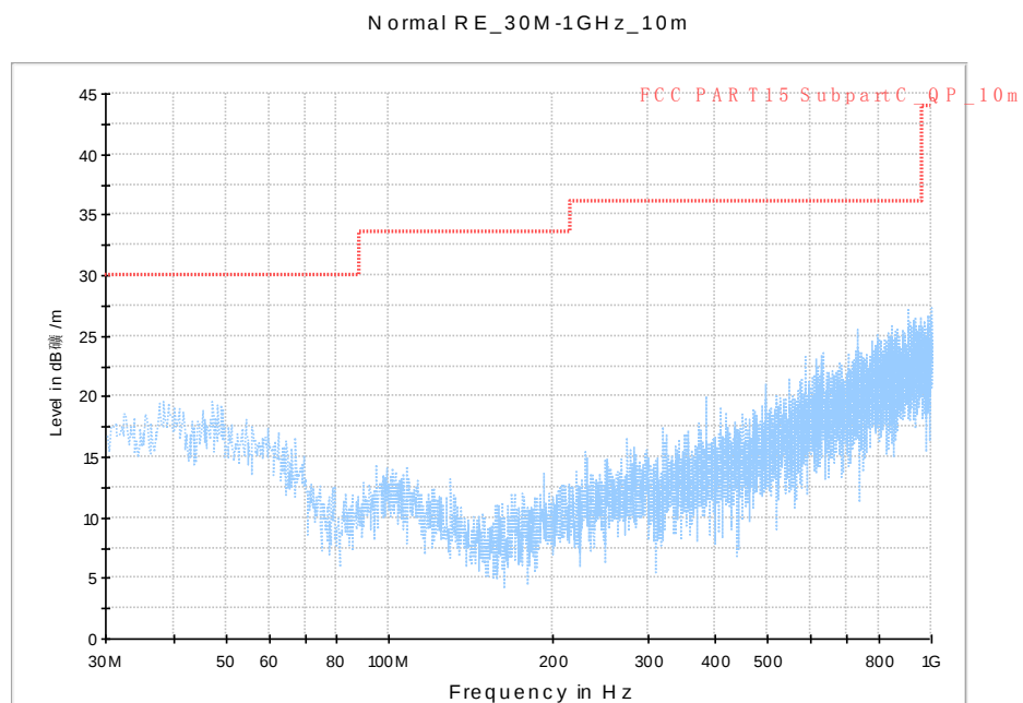
Fig. 64 Radiated Spurious Emission (802.11n-HT20, Ch149, 30 MHz-1 GHz)
