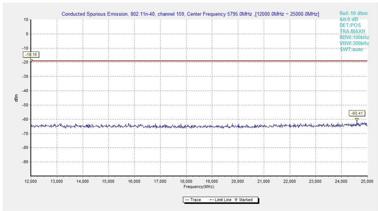
Fig. 47 Conducted Spurious Emission (802.11n-HT40, Ch159, 12 GHz-25 GHz)
