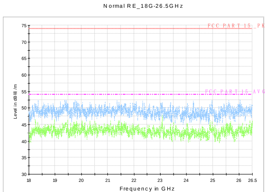
Fig. 73 Radiated Spurious Emission (802.11n-HT20, Ch157, 18 GHz-26.5 GHz)
