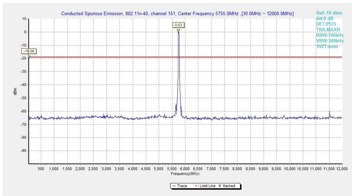
Fig. 42 Conducted Spurious Emission (802.11n-HT40, Ch151, 30 MHz-12 GHz)
