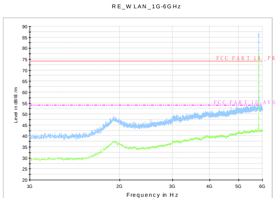
Fig. 60 Radiated Spurious Emission (802.11a, Ch165, 1 GHz-6 GHz)
