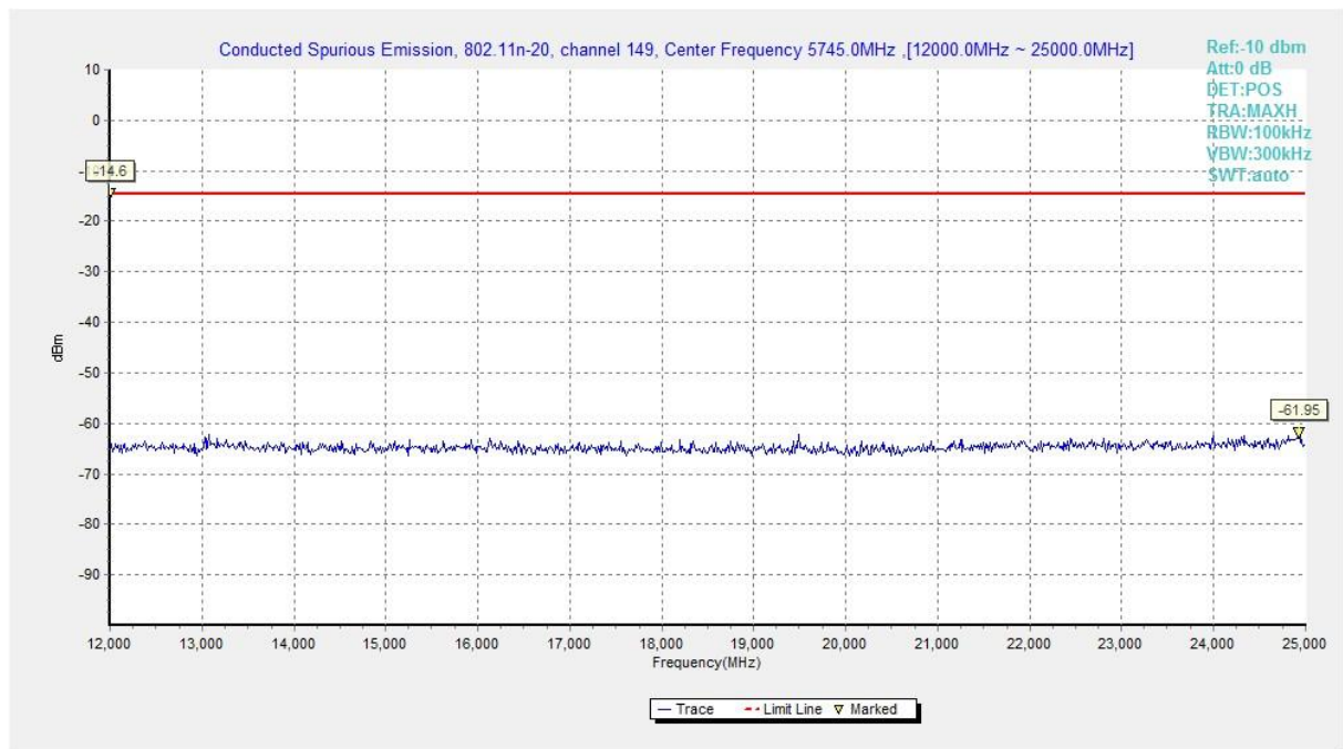
Fig. 31 Conducted Spurious Emission (802.11n-HT20, Ch149, 12 GHz-25 GHz)
