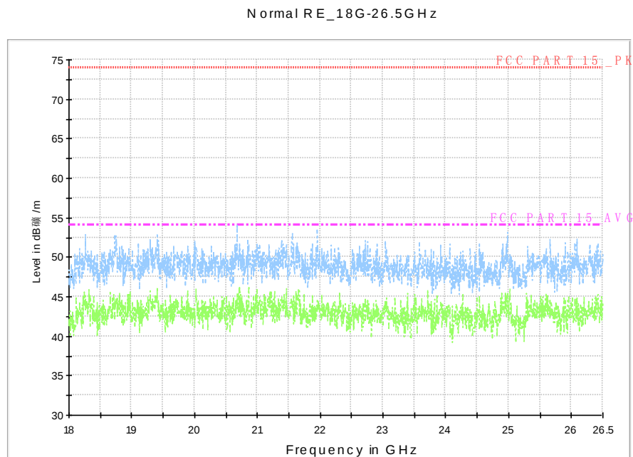
Fig. 62 Radiated Spurious Emission (802.11a, Ch157, 18 GHz-26.5 GHz)
