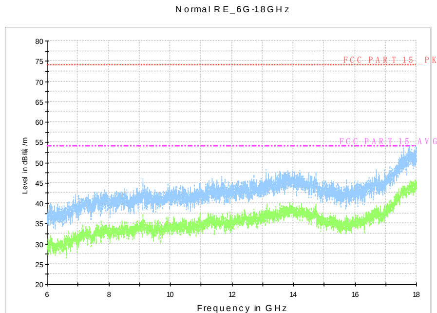
Fig. 80 Radiated Spurious Emission (802.11n-HT40, Ch159, 6 GHz-18 GHz)
