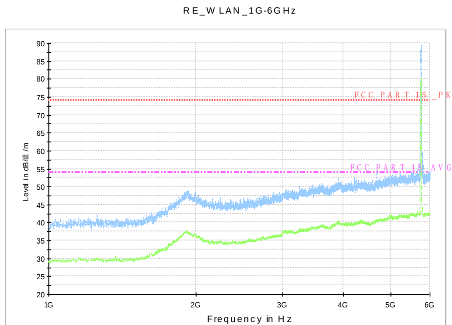
Fig. 76 Radiated Spurious Emission (802.11n-HT40, Ch151, 1 GHz-6 GHz)
