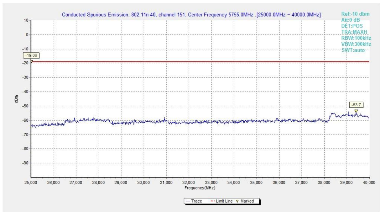
Fig. 44 Conducted Spurious Emission (802.11n-HT40, Ch151, 25 GHz-40 GHz)
