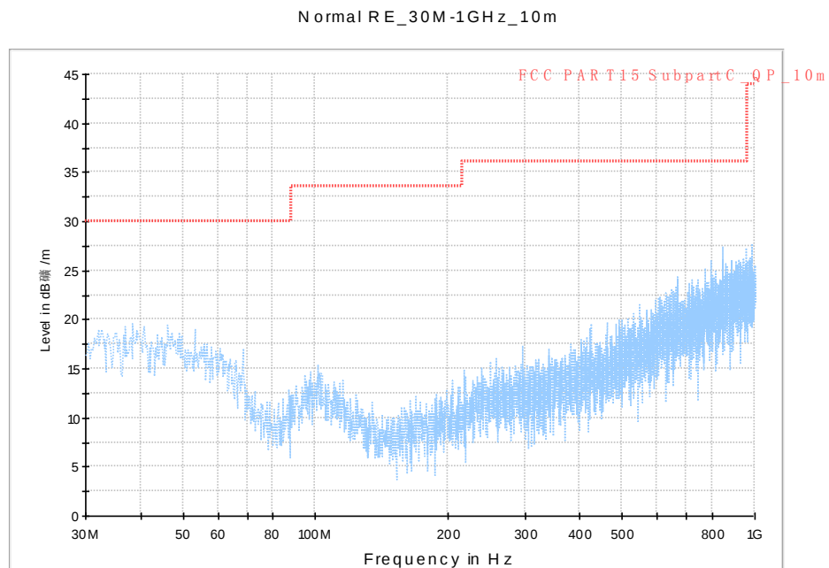
Fig. 78 Radiated Spurious Emission (802.11n-HT40, Ch159, 30 MHz-1 GHz)
