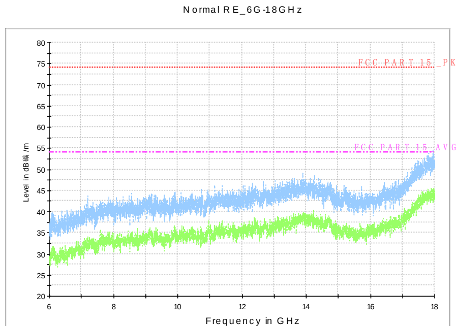
Fig. 72 Radiated Spurious Emission (802.11n-HT20, Ch165, 6 GHz-18 GHz)
