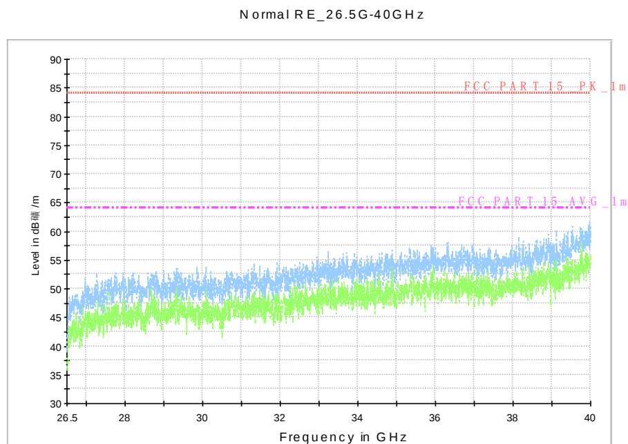
Fig. 74 Radiated Spurious Emission (802.11n-HT20, Ch157, 26.5 GHz - 40 GHz)
