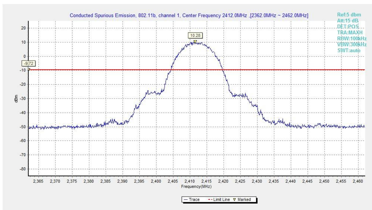
Fig.A.6.1.1 Conducted Spurious Emission (802.11b, Ch1, Center Frequency)
