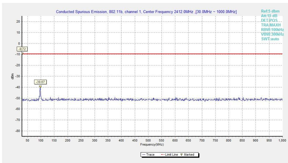
Fig.A.6.1.2 Conducted Spurious Emission (802.11b, Ch1, 30 MHz-1 GHz)
