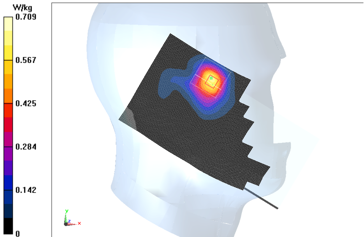
Fig.22 2450 MHz CH1
