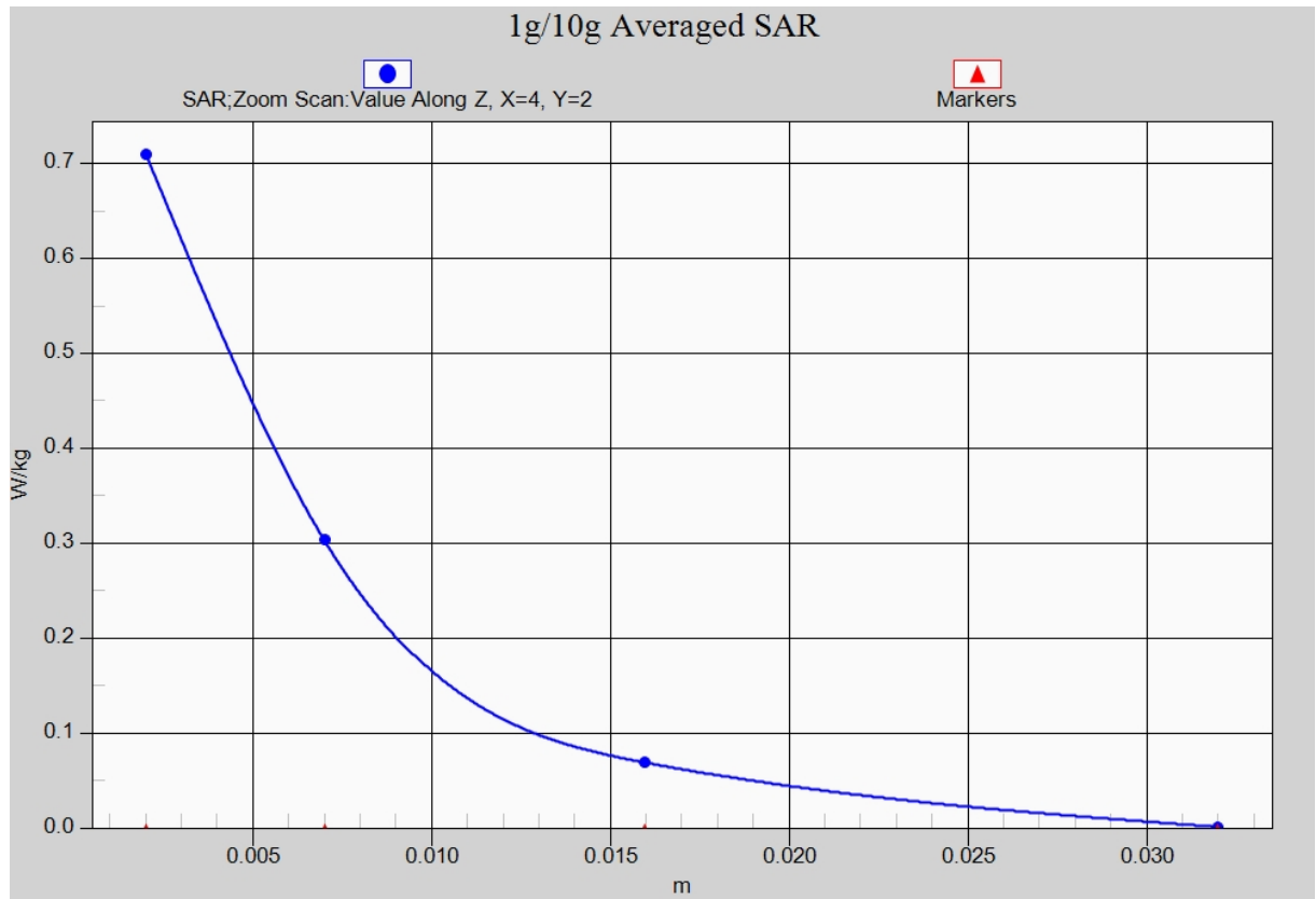
Fig. 22-1 Z-Scan at power reference point (2450 MHz CH1)
