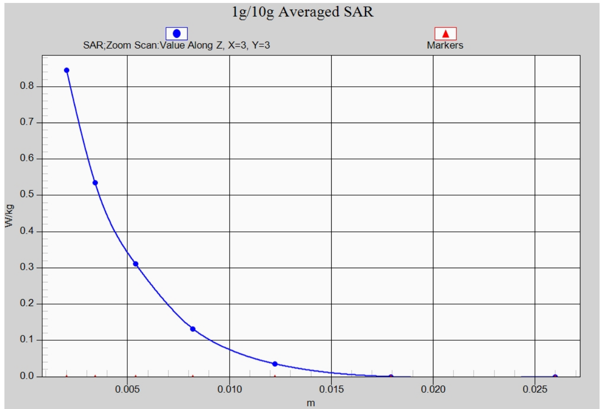
Fig. 25-1 Z-Scan at power reference point (5GHz CH52)
