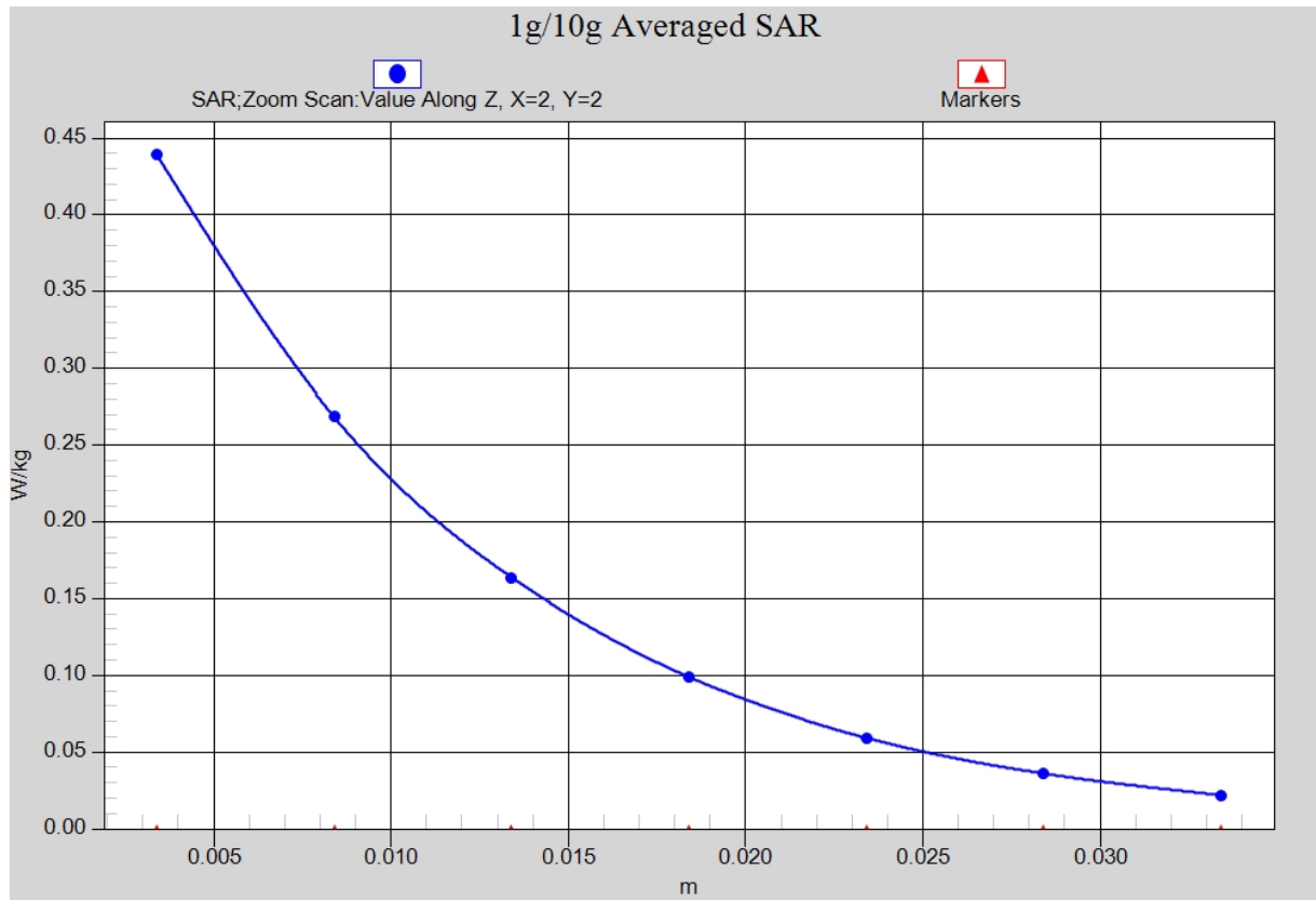
Fig. 15-1 Z-Scan at power reference point (LTE Band2 CH18900)
