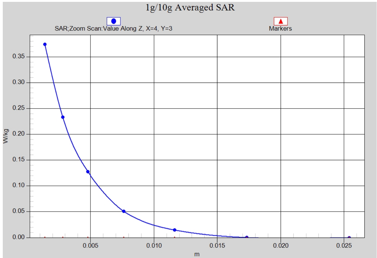
Fig. 24-1 Z-Scan at power reference point (5GHz CH48)
