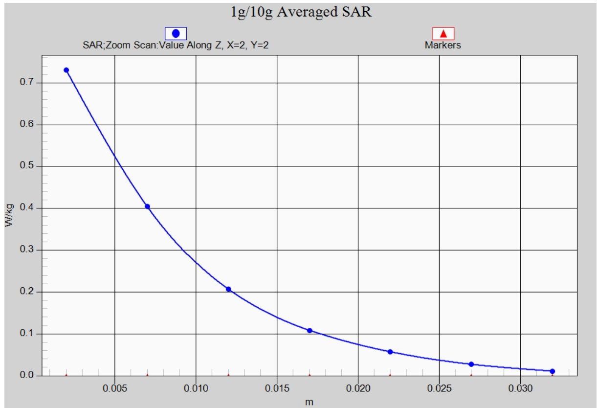
Fig. 23-1 Z-Scan at power reference point (2450 MHz CH6)
