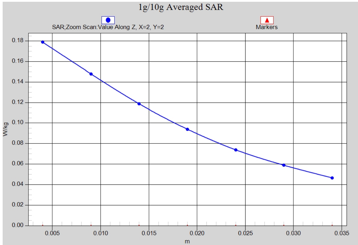
Fig. 21-1 Z-Scan at power reference point (LTE Band17 CH23780)
