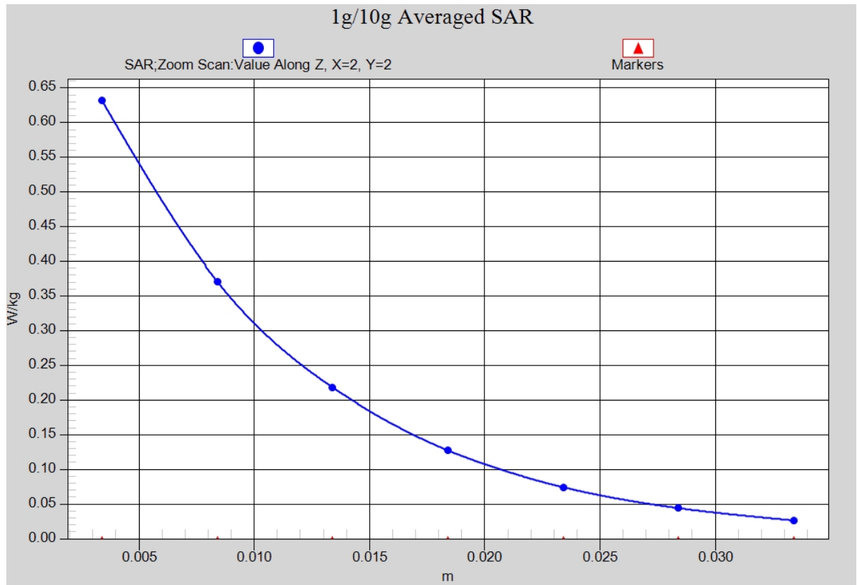
Fig. 16-1 Z-Scan at power reference point (LTE Band2 CH18700)
