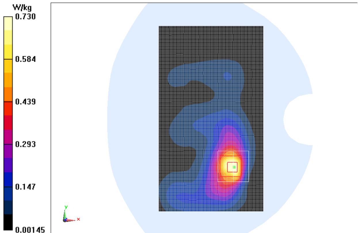
Fig.23 2450 MHz CH6
