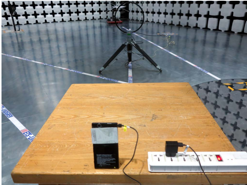
Picture C-1: Field Strength Measurements (Below 30MHz)
