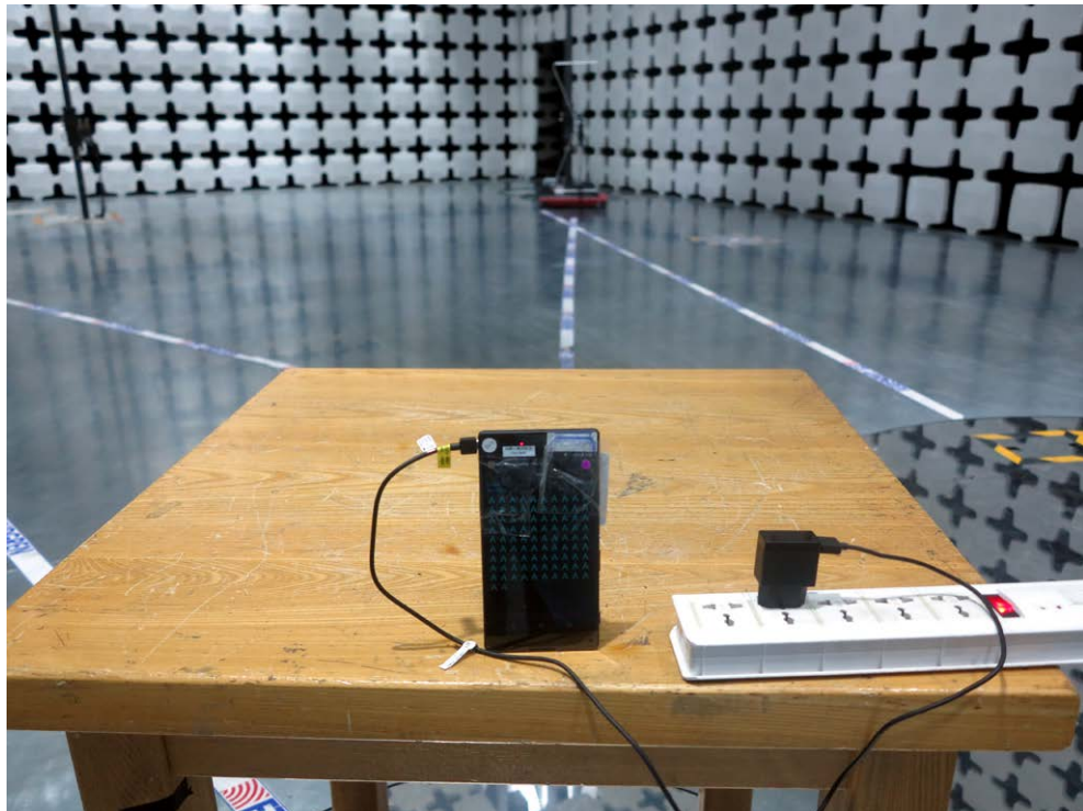
Picture C-2: Field Strength Measurements (Above 30MHz)
