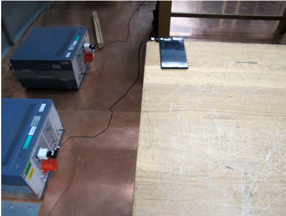
Picture C-3: Conducted Emissions Measurements
