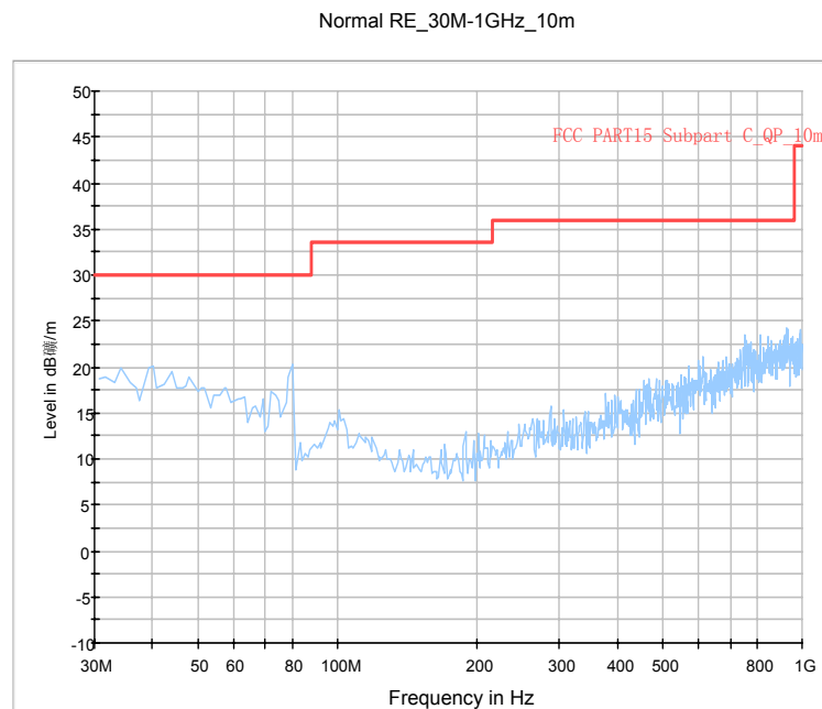
Fig.74. Radiated emission: \pi/4 DQPSK, Channel 39, 30 MHz - 1 GHz
