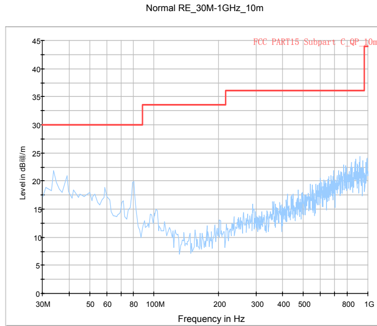
Fig.83. Radiated emission: 8DPSK, Channel 0, 30 MHz - 1 GHz
