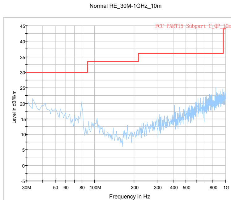
Fig.77. Radiated emission: \pi/4 DQPSK, Channel 78, 30 MHz - 1 GHz
