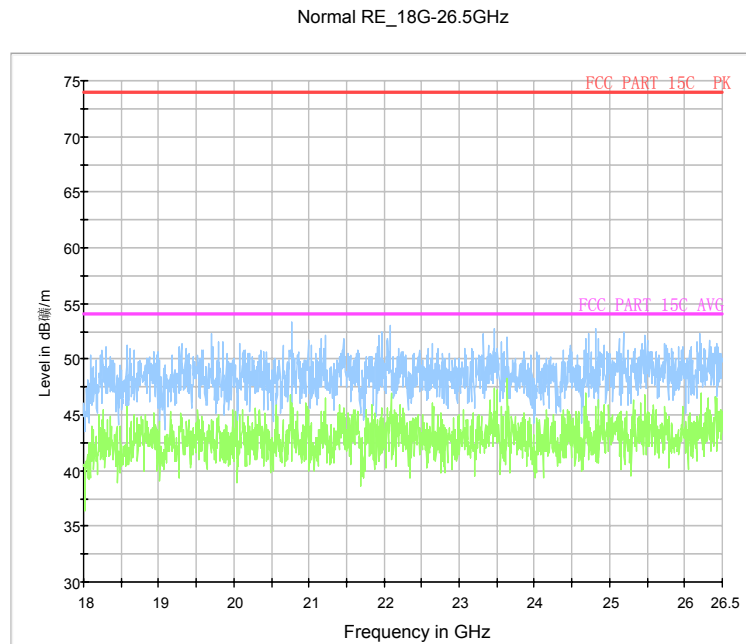
Fig.70. Radiated emission: GFSK, 18 GHz - 26 GHz
