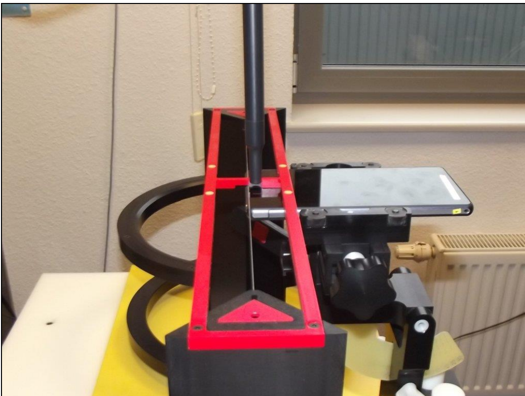
Photo 6: Test position
