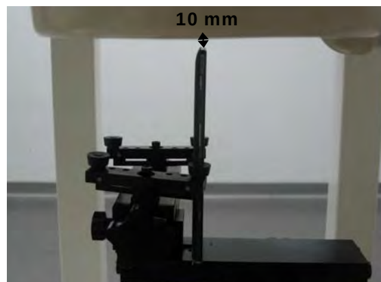
Fig.13 EUT bottom to flat phantom
