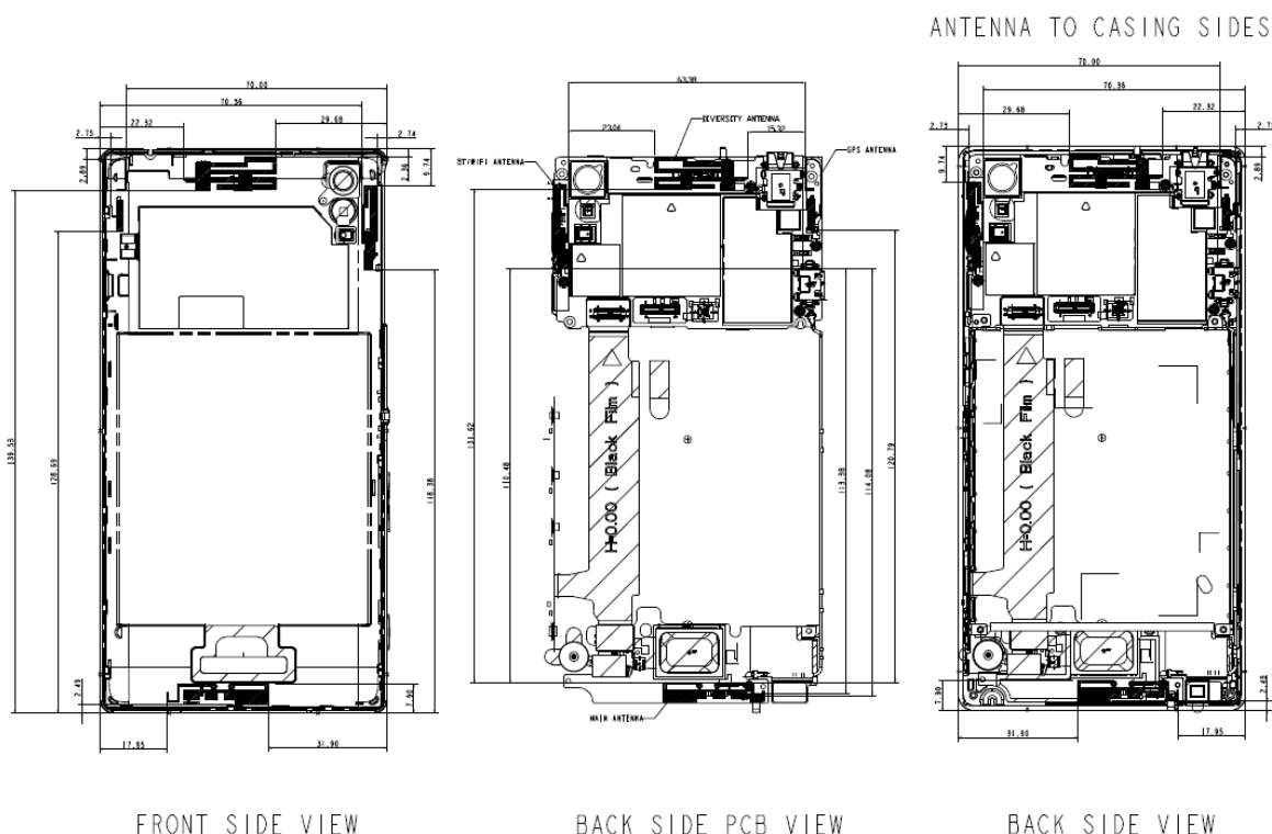
Fig.23 Antenna position of EUT - End of Report -
