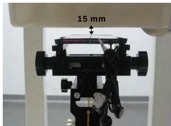
Fig.8 EUT front side with headset (MH410C) to flat phantom
