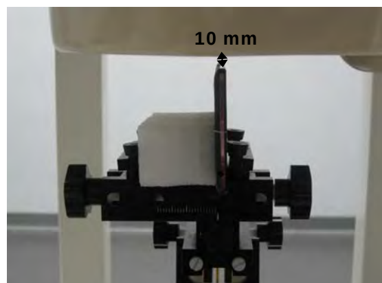
Fig.15 EUT right to flat phantom
