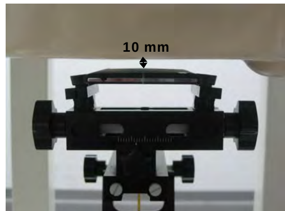
Fig.12 EUT back to flat phantom
