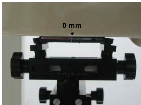
Fig.17 EUT front to flat phantom
