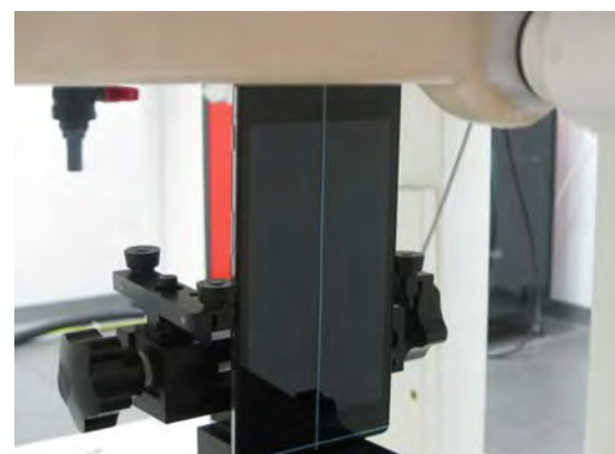
Fig.19 EUT bottom to flat phantom
