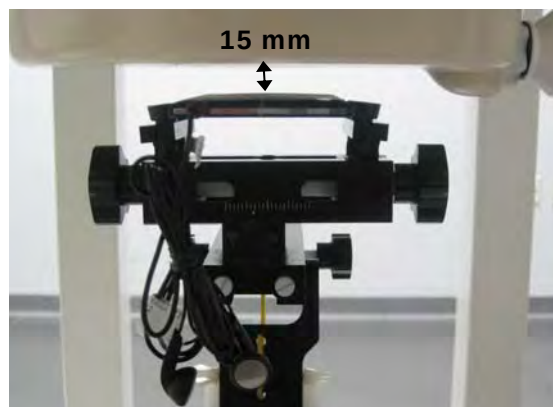
Fig.10 EUT back side with headset (MH410C) to flat phantom
