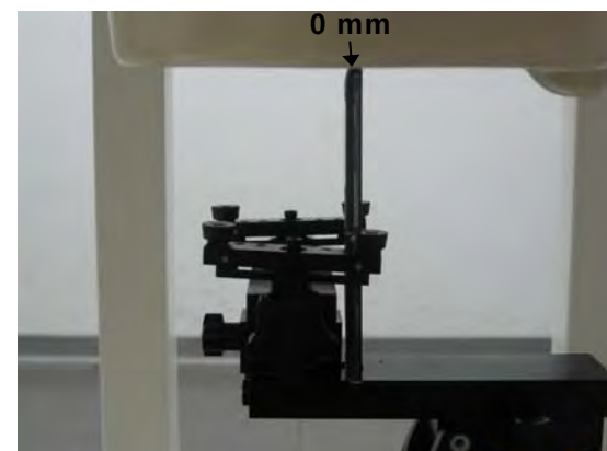
Fig.19 EUT bottom to flat phantom
