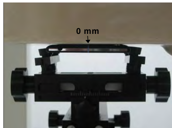
Fig.18 EUT back to flat phantom
