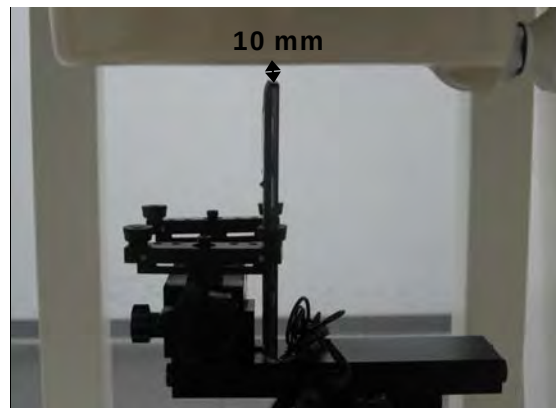
Fig.14 EUT bottom with headset (MH410C) to flat phantom
