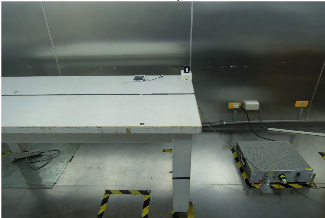
AC Power-line Conducted Emission Set up Photo (Adapter Model number: EP880)
