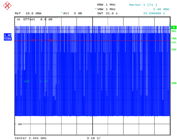
Fig.100. Time of occupancy (Dwell Time): Channel 39, \pi/4 DQPSK -DH1
