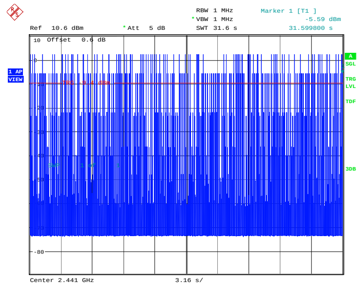
Fig.96. Time of occupancy (Dwell Time): Channel 39, GFSK-DH3
