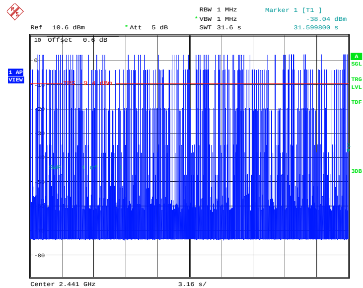
Fig.110. Time of occupancy (Dwell Time): Channel 39, 8DPSK -DH5
