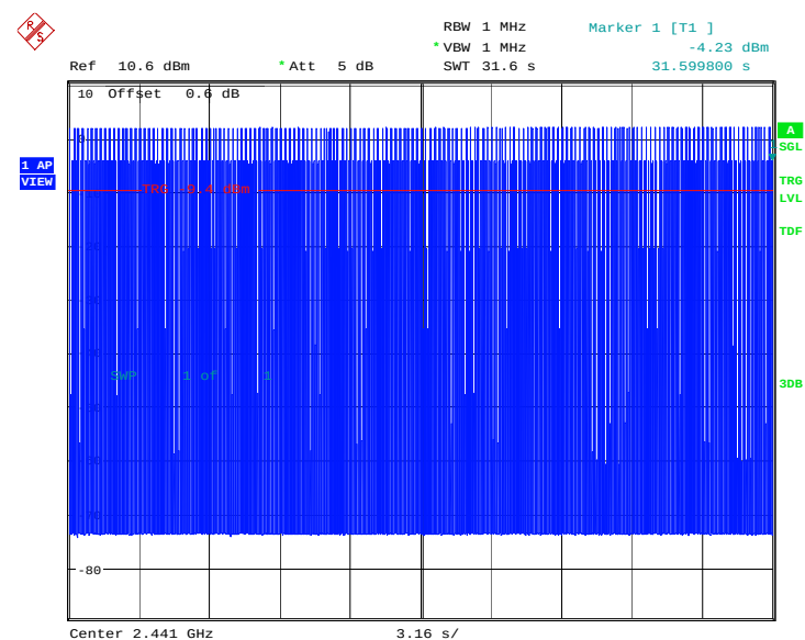
Fig.106. Time of occupancy (Dwell Time): Channel 39, 8DPSK-DH1
