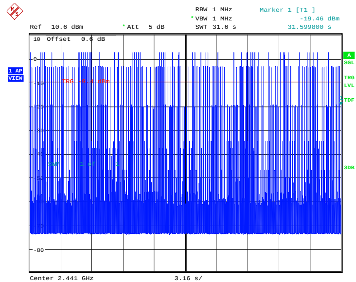
Fig.104. Time of occupancy (Dwell Time): Channel 39, \pi/4 DQPSK -DH5
