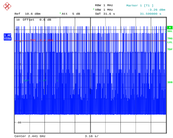
Fig.102. Time of occupancy (Dwell Time): Channel 39, \pi/4 DQPSK -DH3
