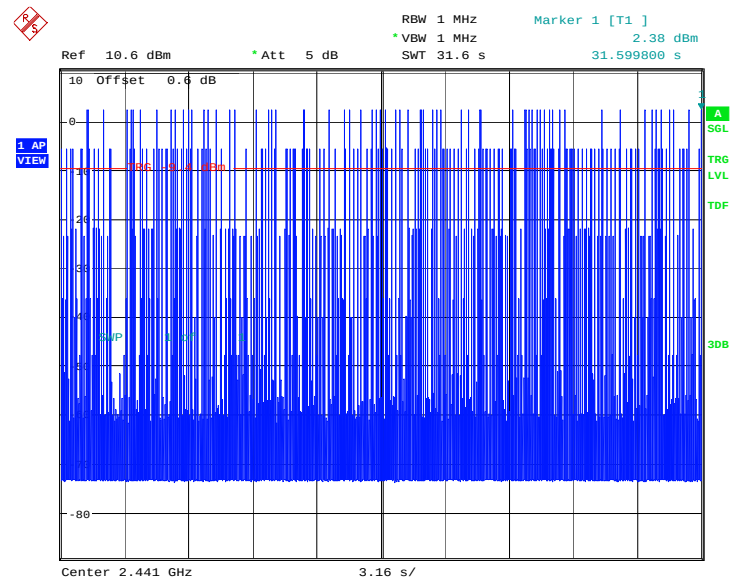
Fig.98. Time of occupancy (Dwell Time): Channel 39, GFSK-DH5
