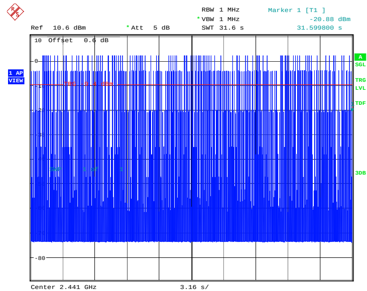
Fig.108. Time of occupancy (Dwell Time): Channel 39, 8DPSK -DH3
