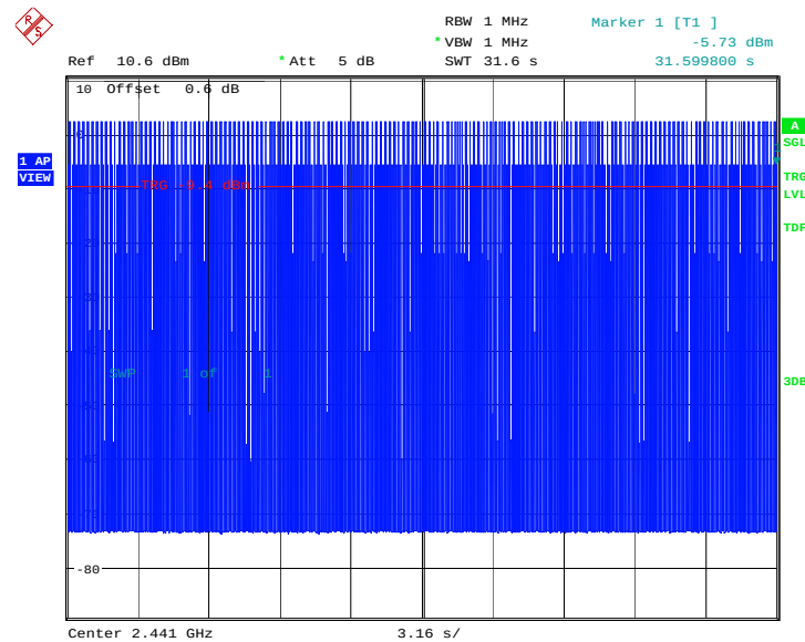
Fig.94. Time of occupancy (Dwell Time): Channel 39, GFSK-DH1
