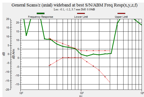
Fig 9.4 GSM1900 Ch512
