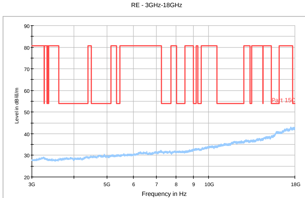
Fig. 53 Radiated Spurious Emission (802.11b, Ch11, 3 GHz-18 GHz)
