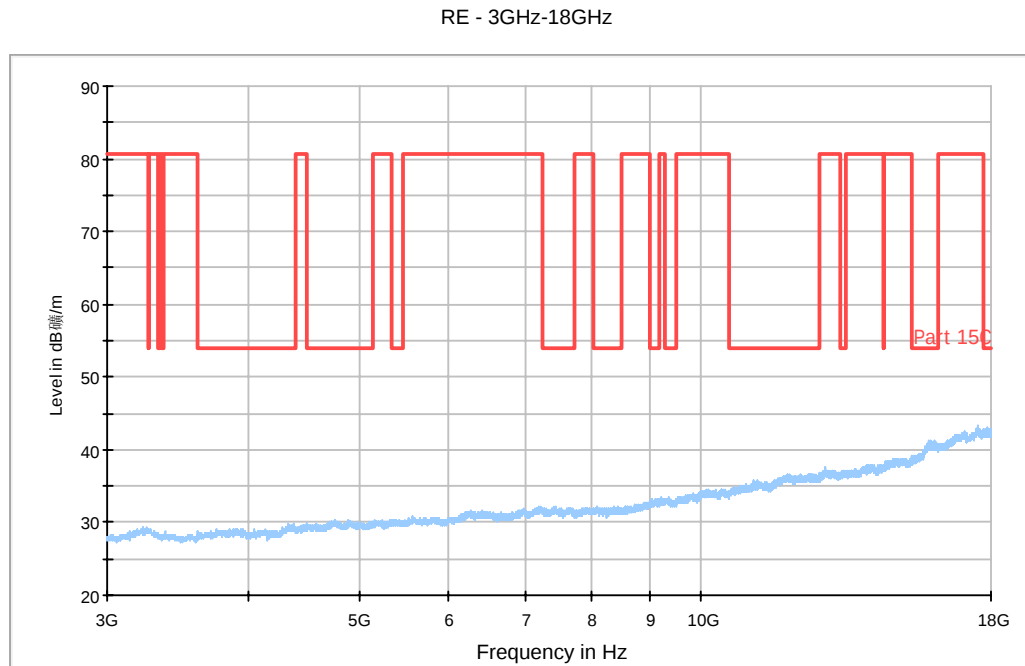
Fig. 71 Radiated Spurious Emission (802.11n-HT20, Ch6, 3 GHz-18 GHz)
