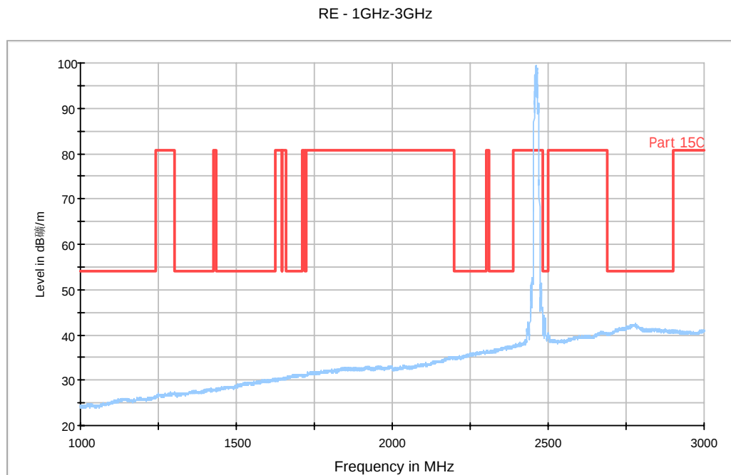
Fig. 52 Radiated Spurious Emission (802.11b, Ch11, 1 GHz-3 GHz)
