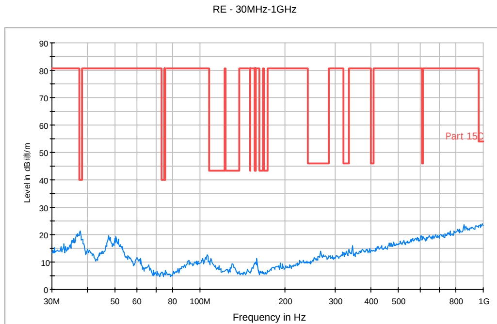
Fig. 66 Radiated Spurious Emission (802.11n-HT20, Ch1, 30 MHz-1 GHz)
