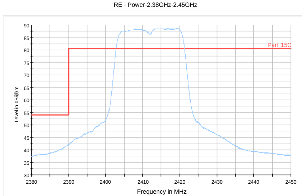
Fig. 65 Radiated Spurious Emission (Power): 802.11n-HT20, ch1, 2.38 GHz - 2.45GHz
