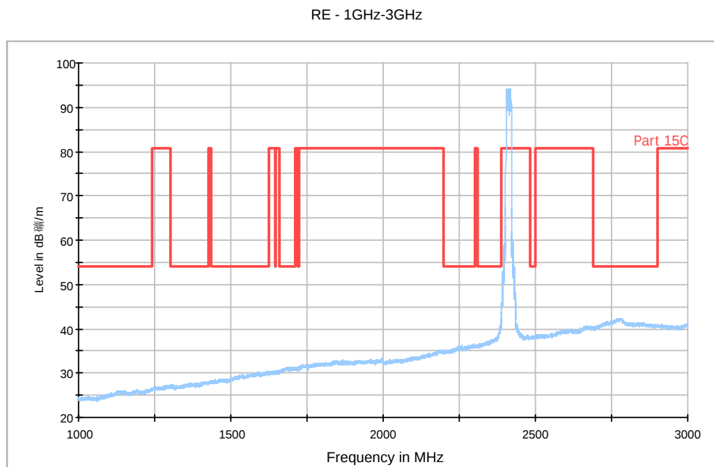
Fig. 56 Radiated Spurious Emission (802.11g, Ch1, 1 GHz-3 GHz)
