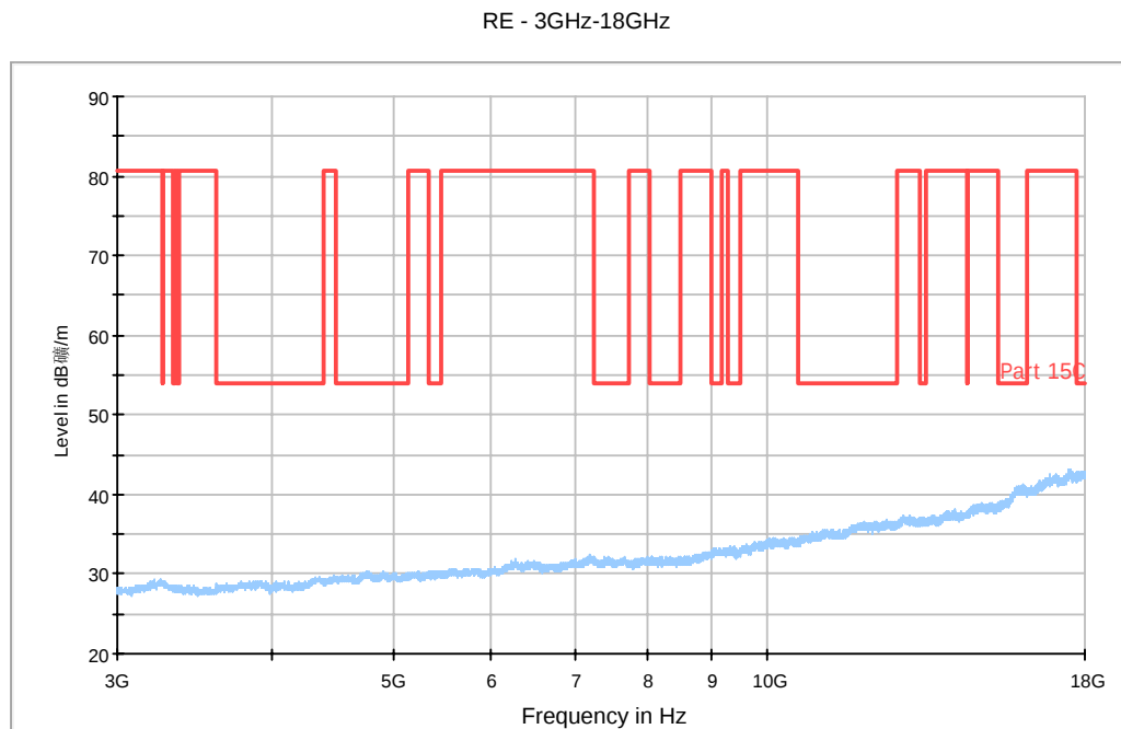
Fig. 75 Radiated Spurious Emission (802.11n-HT20, Ch11, 3 GHz-18 GHz)
