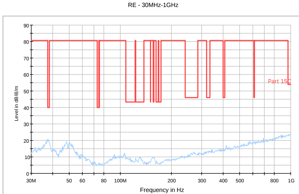
Fig. 55 Radiated Spurious Emission (802.11g, Ch1, 30 MHz-1 GHz)
