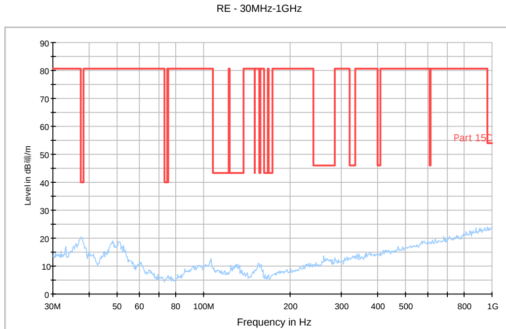
Fig. 51 Radiated Spurious Emission (802.11b, Ch11, 30 MHz-1 GHz)
