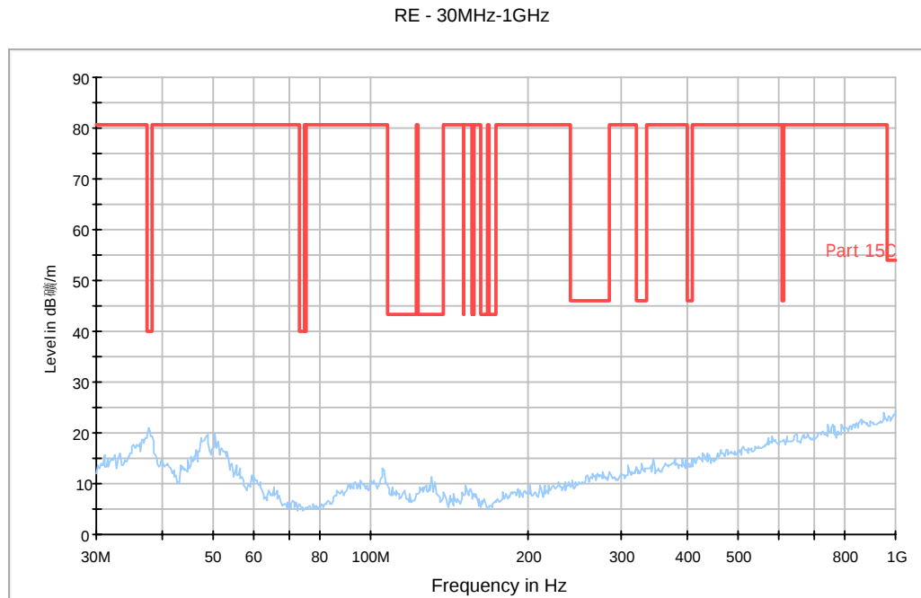
Fig. 69 Radiated Spurious Emission (802.11n-HT20, Ch6, 30 MHz-1 GHz)
