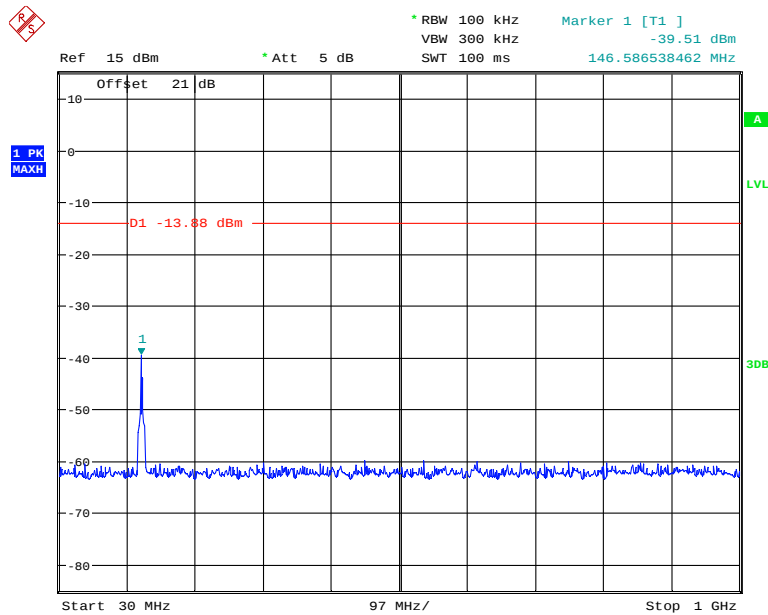
Fig. 22 Conducted Spurious Emission (802.11b, Ch11, Center Frequency)
