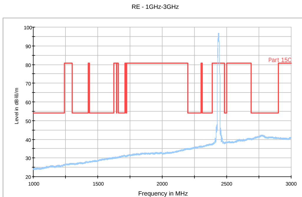
Fig. 48 Radiated Spurious Emission (802.11b, Ch6, 1 GHz-3 GHz)
