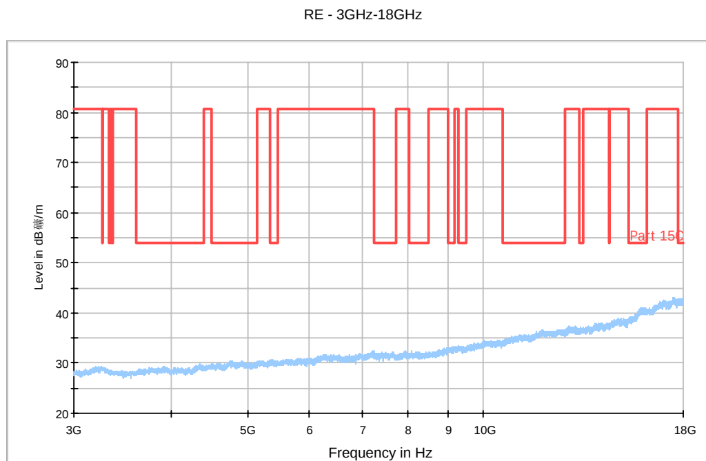
Fig. 68 Radiated Spurious Emission (802.11n-HT20, Ch1, 3 GHz-18 GHz)
