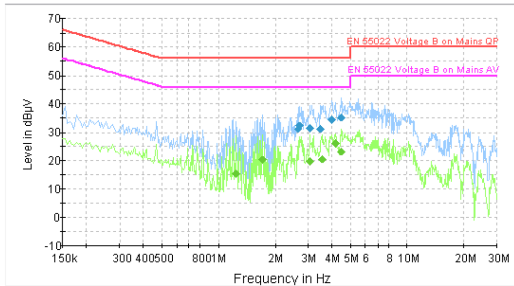
Fig. 87 AC Powerline Conducted Emission
