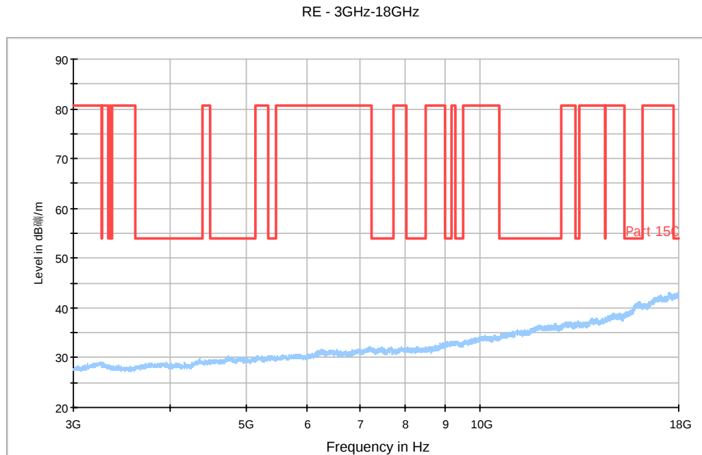
Fig. 60 Radiated Spurious Emission (802.11g, Ch6, 3 GHz-18 GHz)
