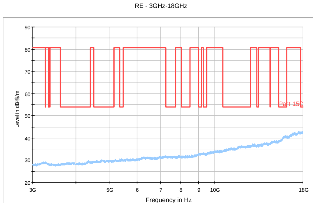
Fig. 46 Radiated Spurious Emission (802.11b, Ch1, 3 GHz-18 GHz)
