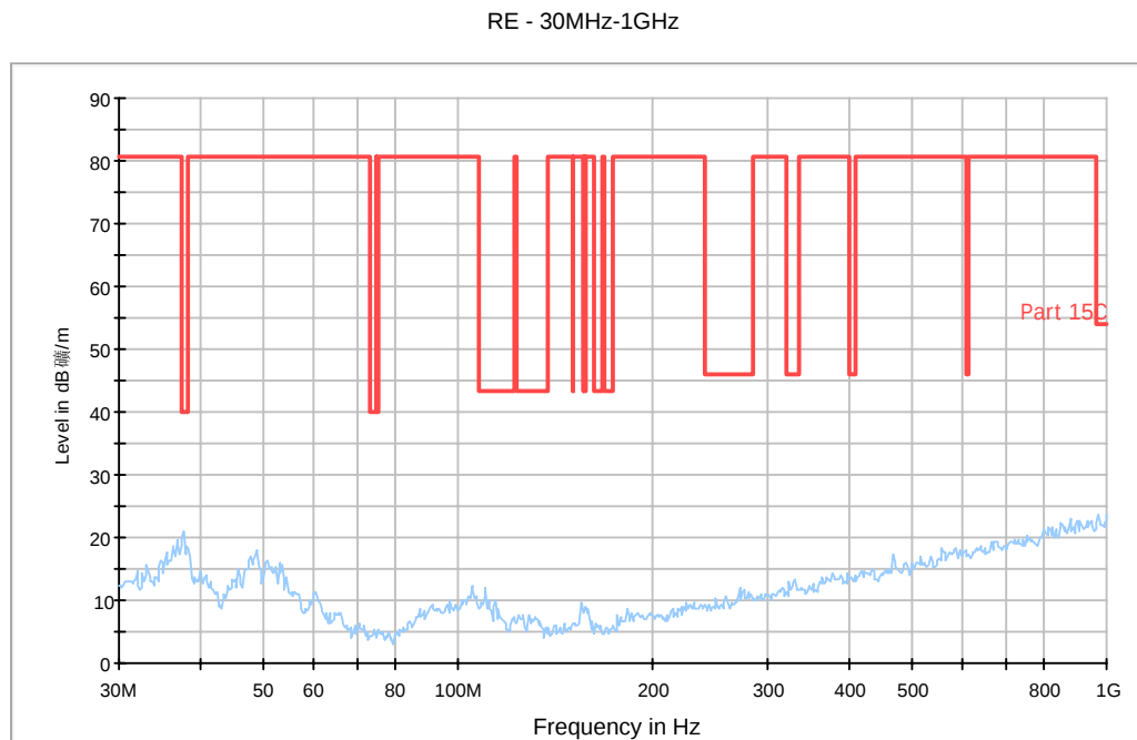
Fig. 44 Radiated Spurious Emission (802.11b, Ch1, 30 MHz-1 GHz)
