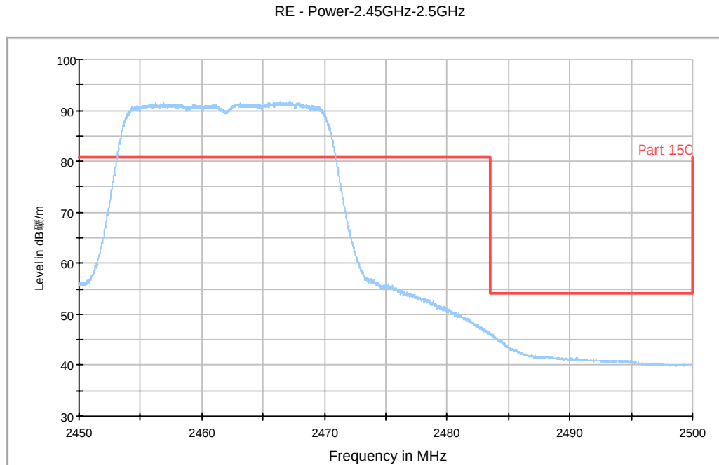
Fig. 61 Radiated Spurious Emission (Power): 802.11g, ch11, 2.45 GHz - 2.5GHz
