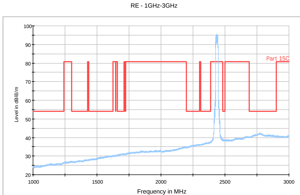
Fig. 70 Radiated Spurious Emission (802.11n-HT20, Ch6, 1 GHz-3 GHz)
