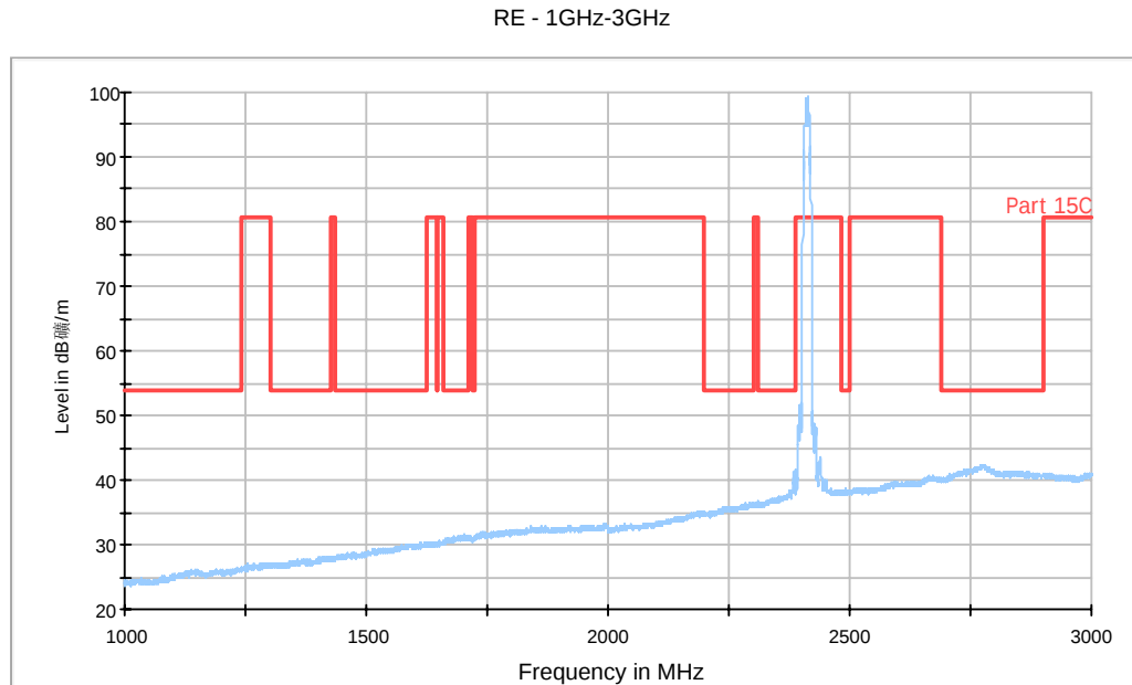
Fig. 45 Radiated Spurious Emission (802.11b, Ch1, 1 GHz-3 GHz)
