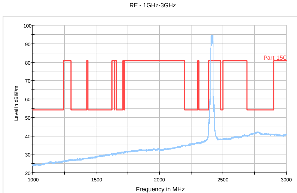
Fig. 67 Radiated Spurious Emission (802.11n-HT20, Ch1, 1 GHz-3 GHz)
