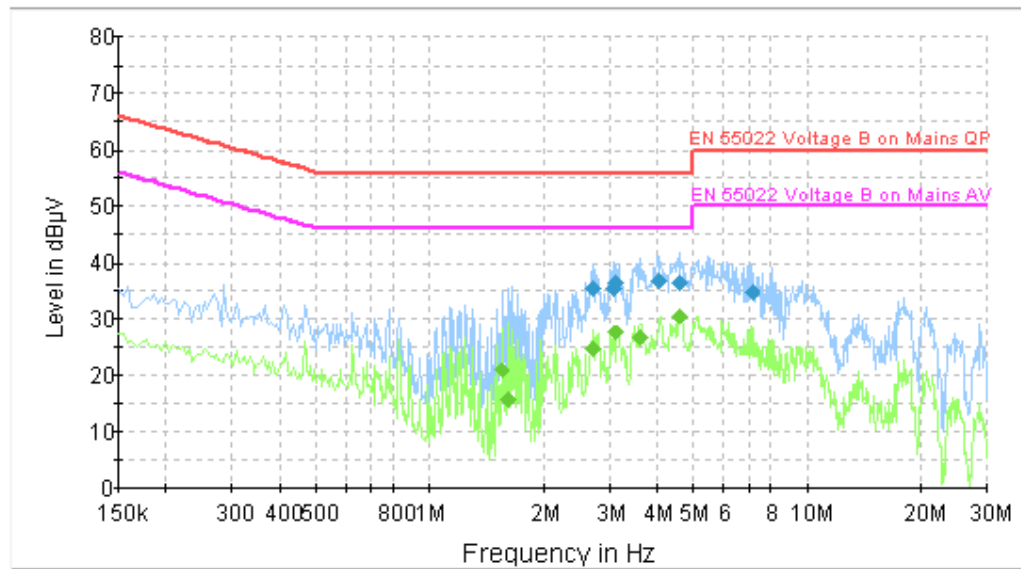
Fig. 86 AC Powerline Conducted Emission
