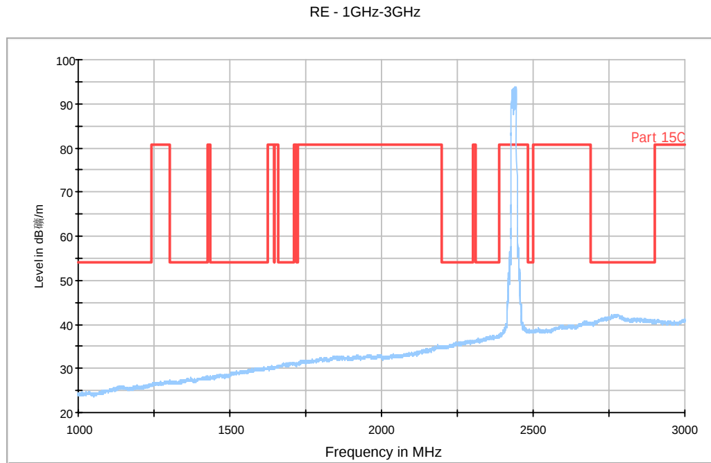
Fig. 59 Radiated Spurious Emission (802.11g, Ch6, 1 GHz-3 GHz)
