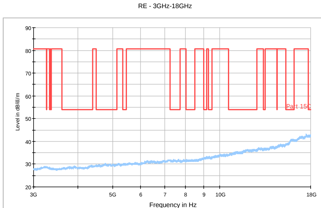
Fig. 64 Radiated Spurious Emission (802.11g, Ch11, 3 GHz-18 GHz)
