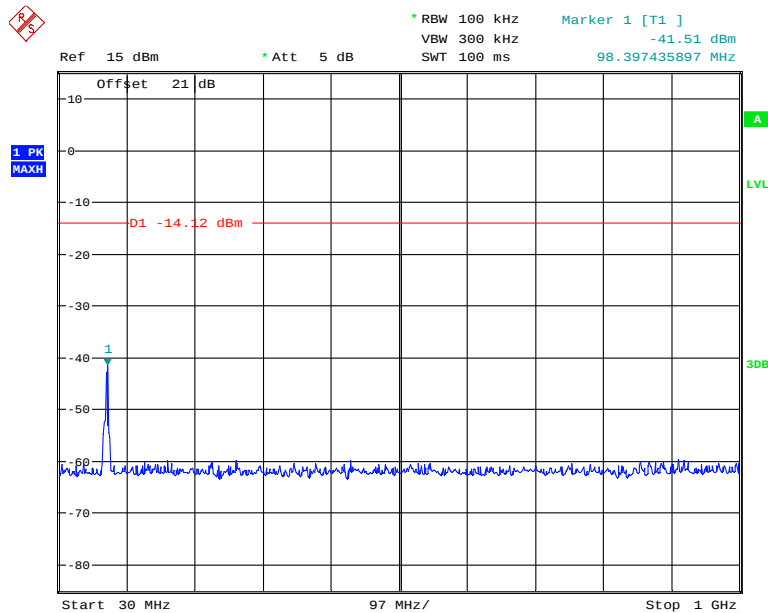
Fig. 16 Conducted Spurious Emission (802.11b, Ch1, Center Frequency)
