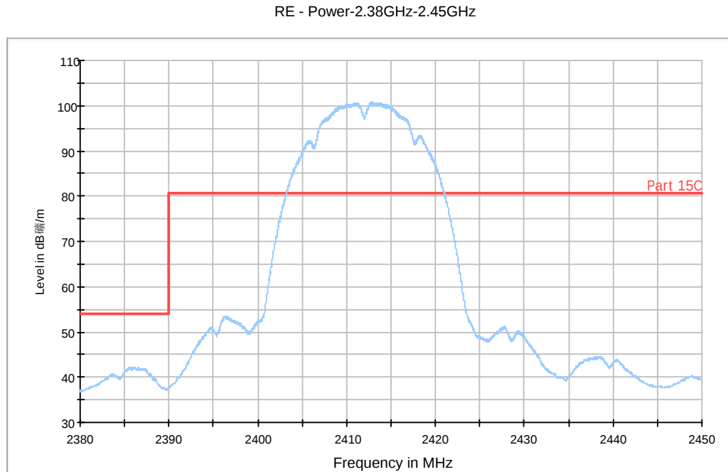
Fig. 43 Radiated Spurious Emission (Power): 802.11b, ch1, 2.38 GHz - 2.45GHz
