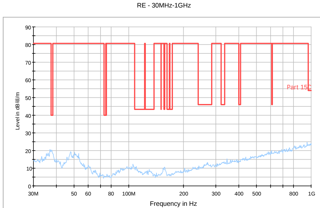
Fig. 73 Radiated Spurious Emission (802.11n-HT20, Ch11, 30 MHz-1 GHz)
