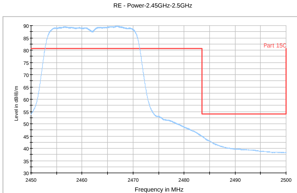
Fig. 72 Radiated Spurious Emission (Power): 802.11n-HT20, ch11, 2.45 GHz - 2.5GHz
