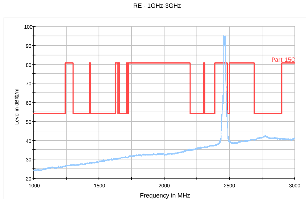
Fig. 74 Radiated Spurious Emission (802.11n-HT20, Ch11, 1 GHz-3 GHz)
