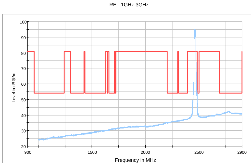
Fig. 63 Radiated Spurious Emission (802.11g, Ch11, 1 GHz-3 GHz)
