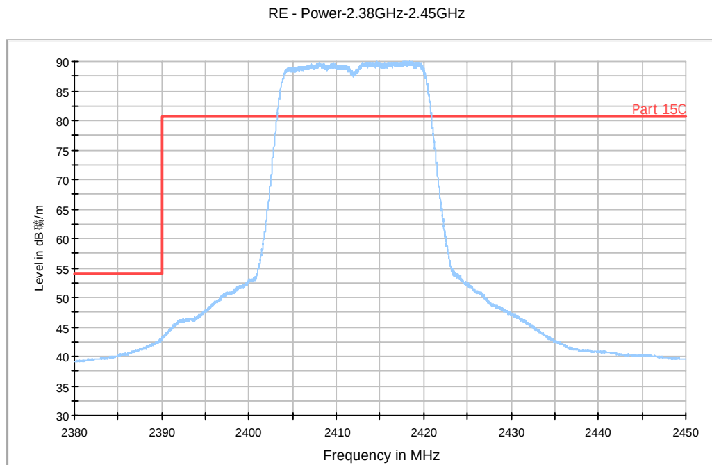
Fig. 54 Radiated Spurious Emission (Power): 802.11g, ch1, 2.38 GHz - 2.45GHz
