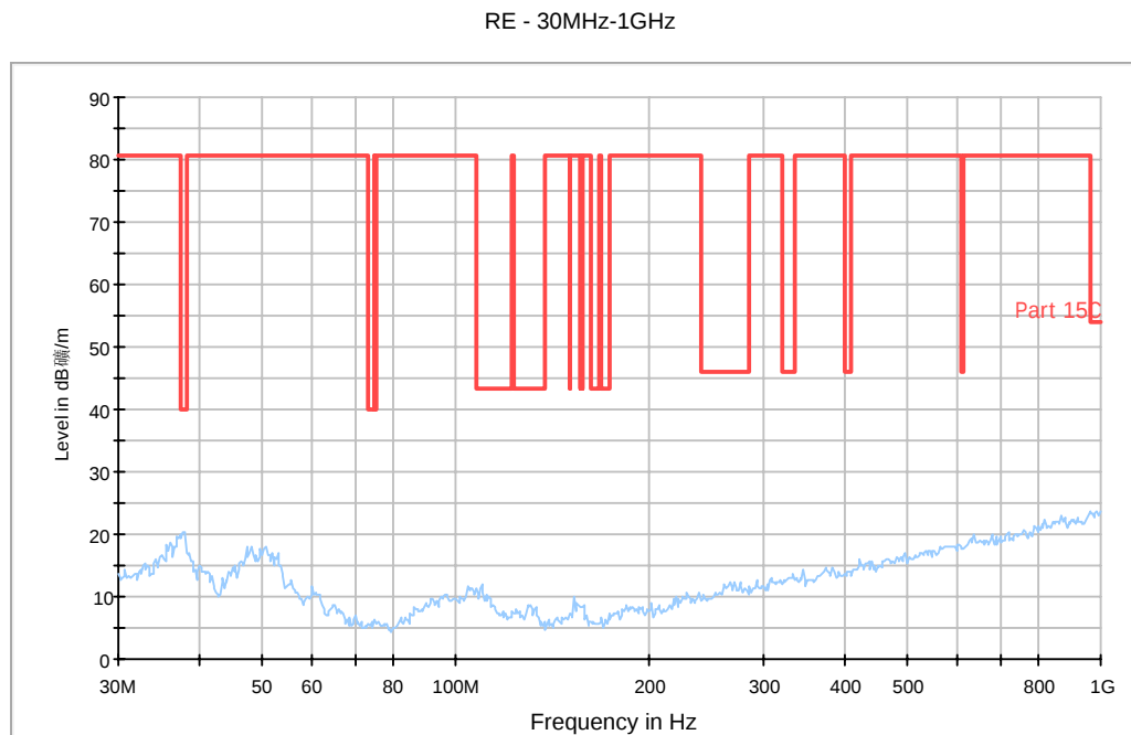
Fig. 47 Radiated Spurious Emission (802.11b, Ch6, 30 MHz-1 GHz)
