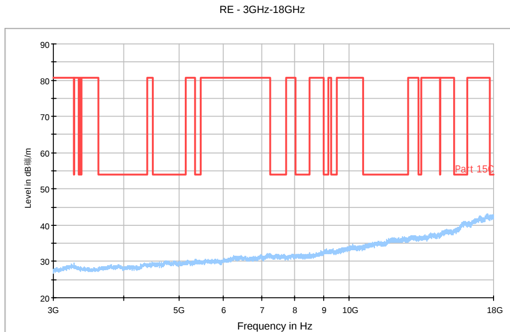
Fig. 57 Radiated Spurious Emission (802.11g, Ch1, 3 GHz-18 GHz)
