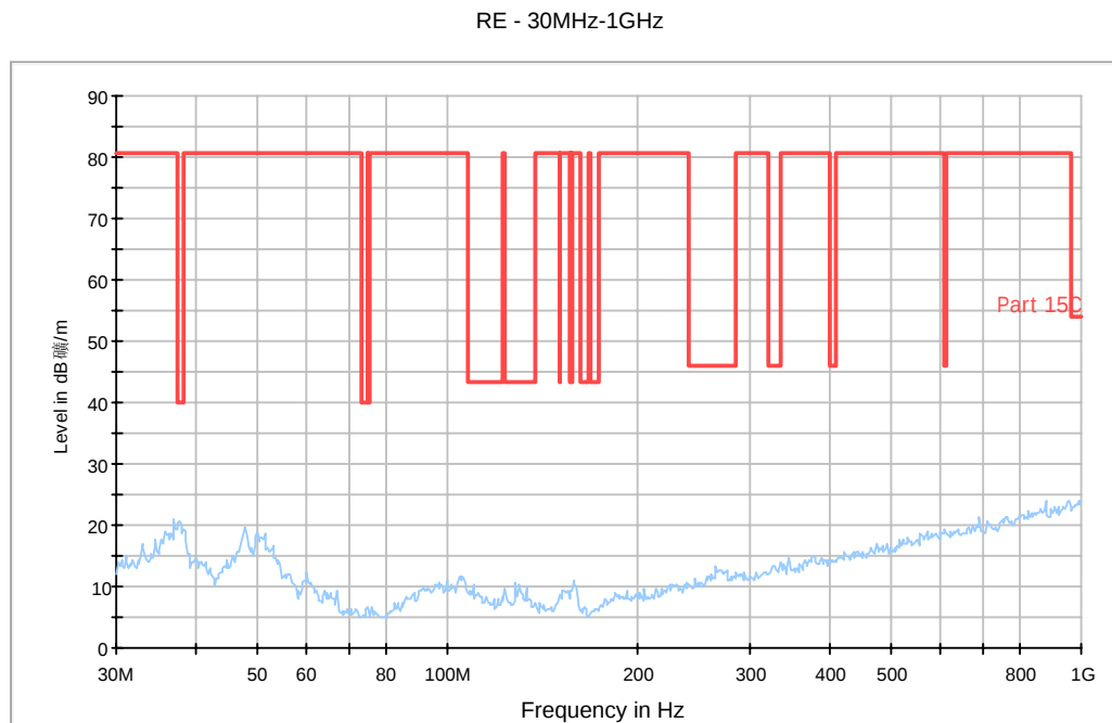
Fig. 62 Radiated Spurious Emission (802.11g, Ch11, 30 MHz-1 GHz)
