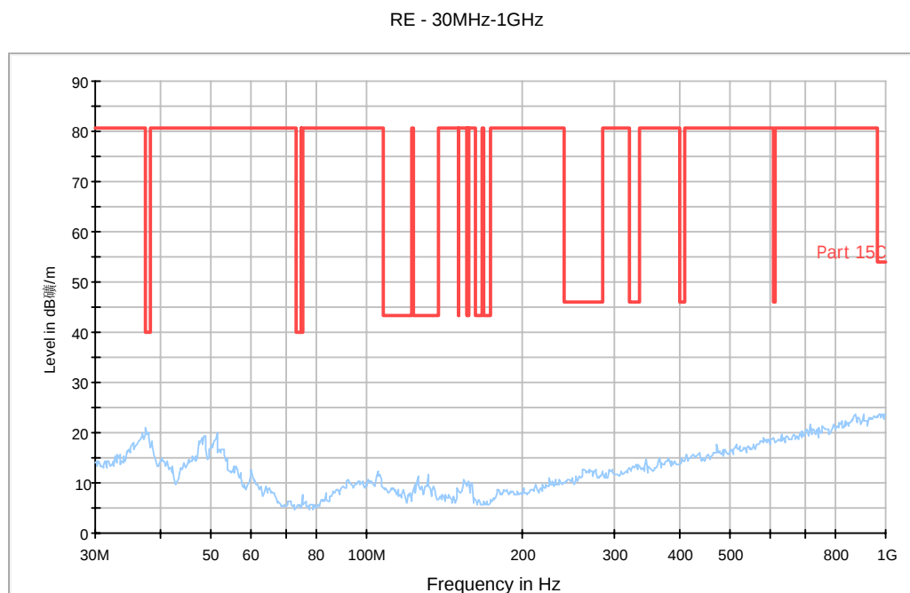
Fig. 58 Radiated Spurious Emission (802.11g, Ch6, 30 MHz-1 GHz)
