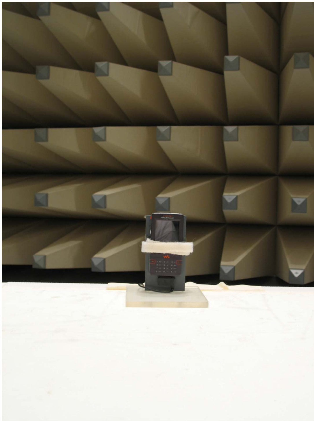
Photo 1 (Radiated Emissions):
