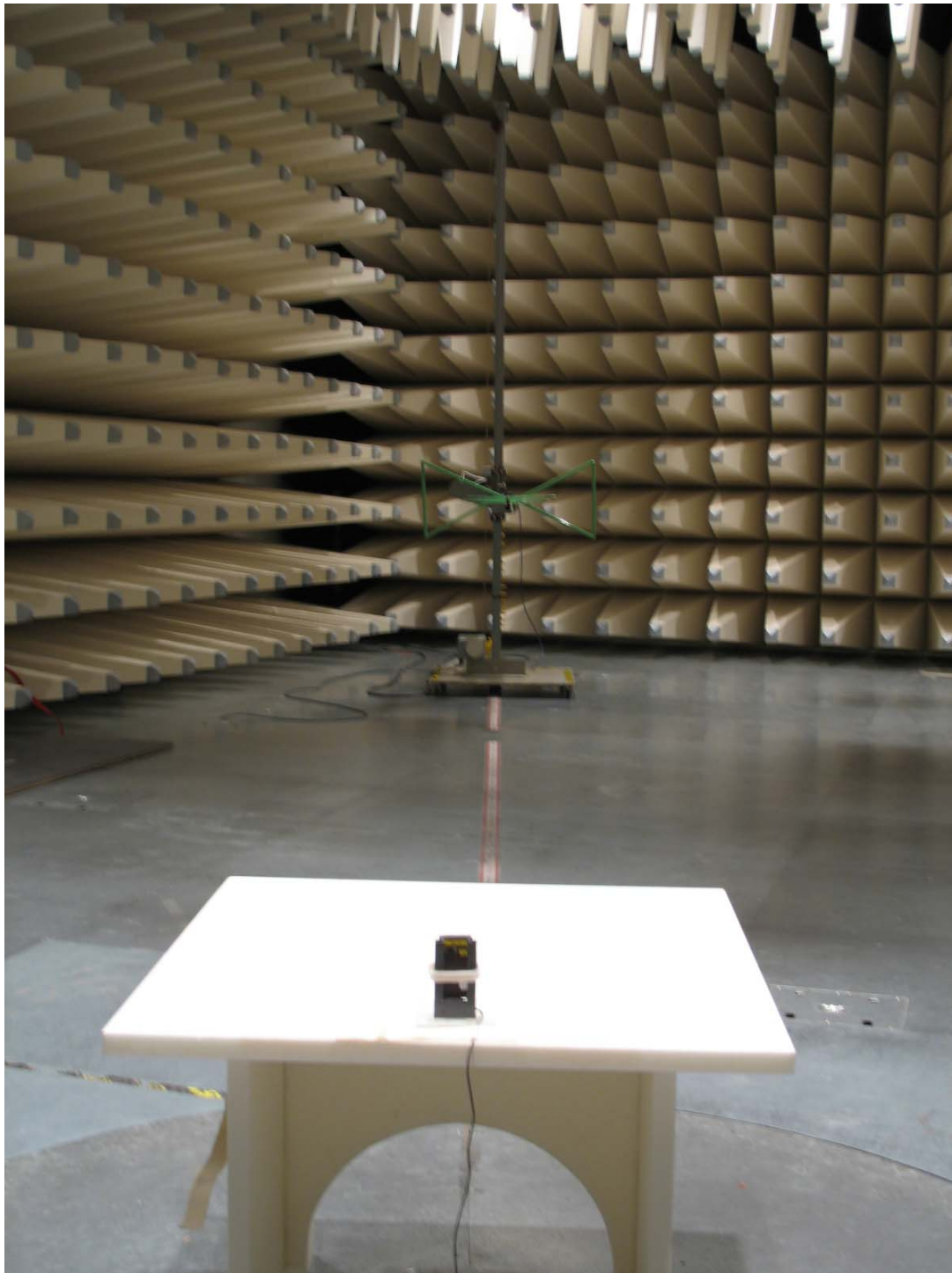
Photo 2 (Radiated Emissions):
