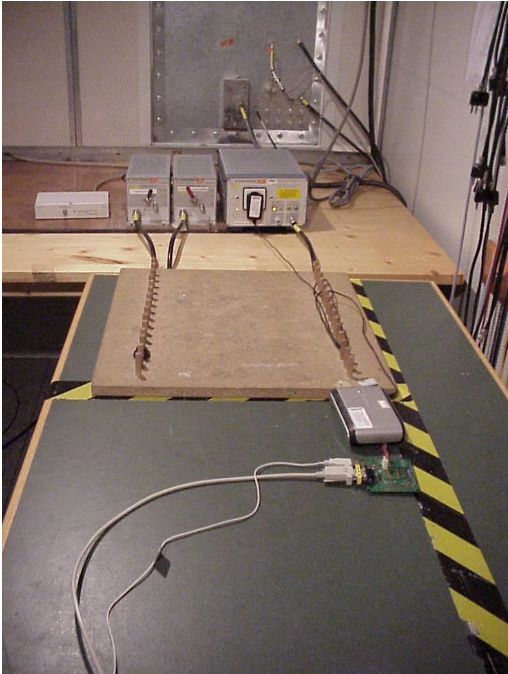
Photo 3: Conducted Emissions
