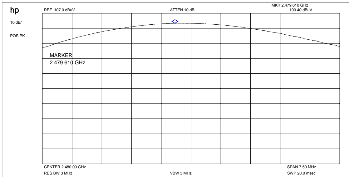
Plot 1 : Max field strength in 3m distance (single frequency)
