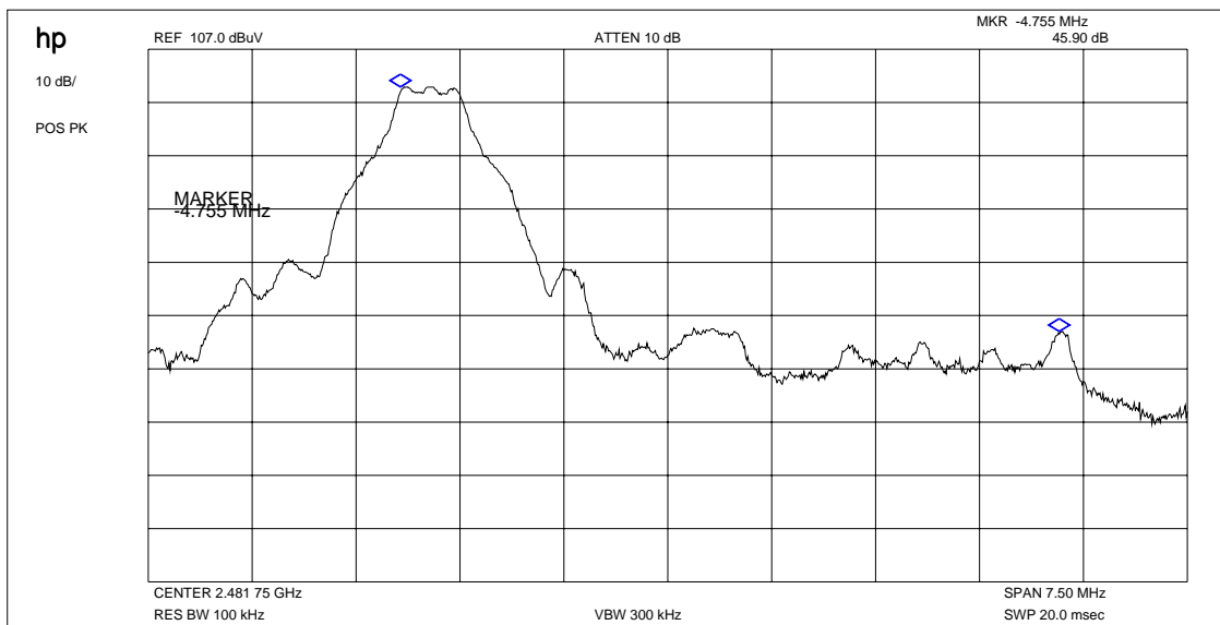
Plot 2: Marker-Delta Method (single carrier)
