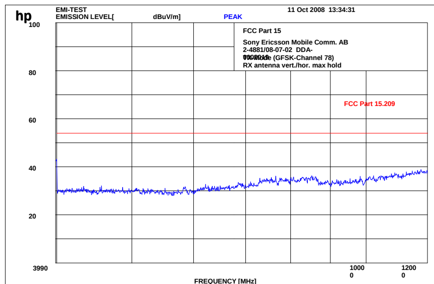
Plot 10: 4 - 12 GHz vertical/horizontal (GFSK - highest channel)
