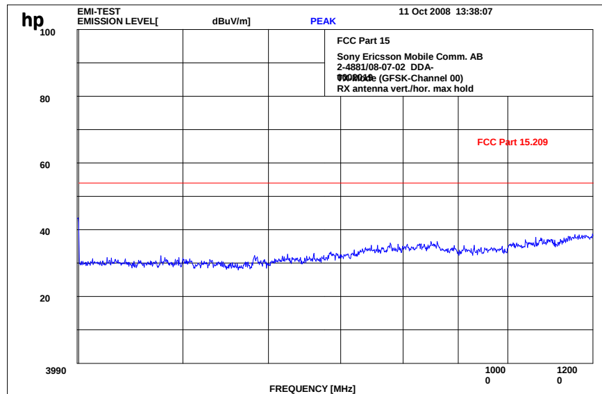
Plot 3: 4 - 12 GHz vertical/horizontal (GFSK - lowest channel)
