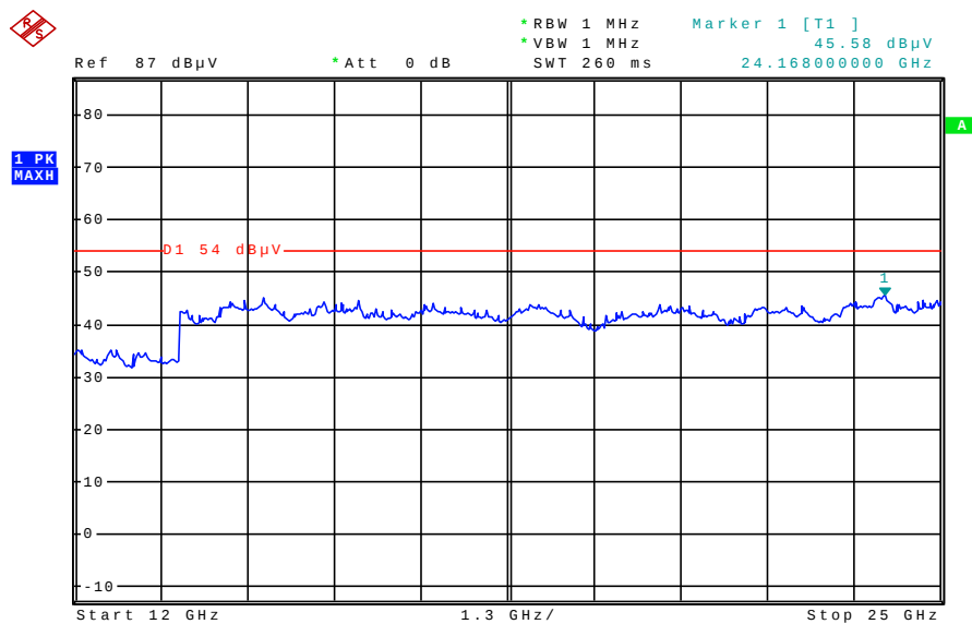
Plot 4: 12 - 25 GHz vertical/horizontal (Pi/4 DQPSK - valid for all channels)
