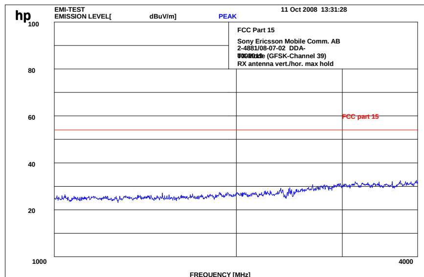
Plot 6: 1 - 4 GHz vertical/horizontal (GFSK - middle channel)
