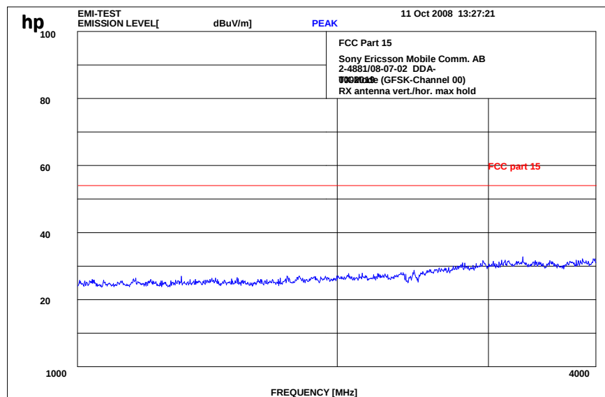
Plot 2: 1 - 4 GHz vertical/horizontal (GFSK - lowest channel)
