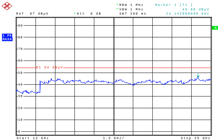
Plot 4: 12 - 25 GHz vertical/horizontal (GFSK - valid for all channels)
