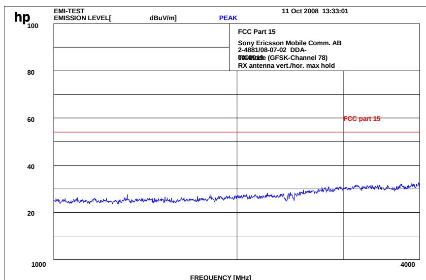
Plot 9: 1 - 4 GHz vertical/horizontal (GFSK - highest channel)
