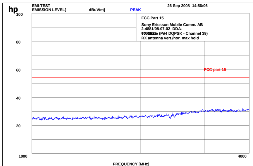
Plot 6: 1 - 4 GHz vertical/horizontal (Pi/4 DQPSK - middle channel)
