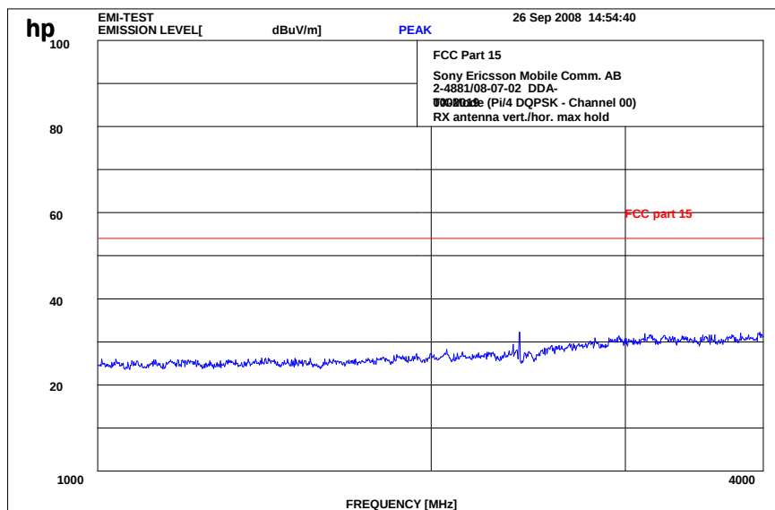
Plot 2: 1 - 4 GHz vertical/horizontal (Pi/4 DQPSK - lowest channel)
