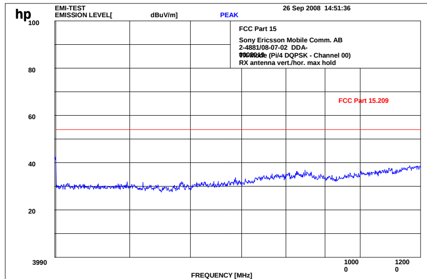
Plot 3: 4 - 12 GHz vertical/horizontal (Pi/4 DQPSK - lowest channel)
