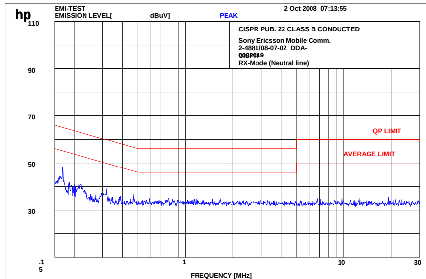
Plot 3: RX-Mode (Neutral line); valid for all modulations
