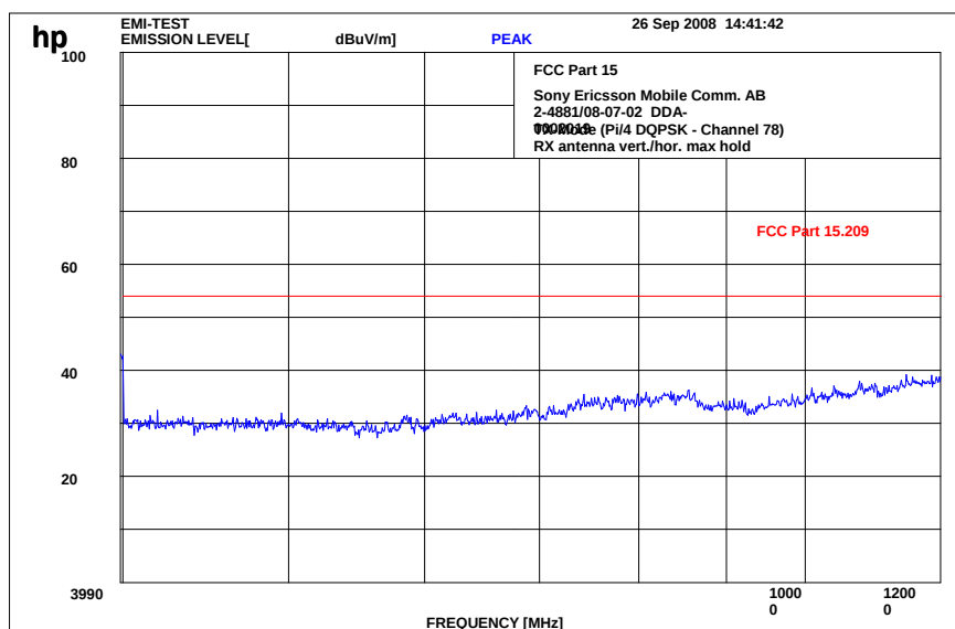
Plot 10: 4 - 12 GHz vertical/horizontal (Pi/4 DQPSK - highest channel)
