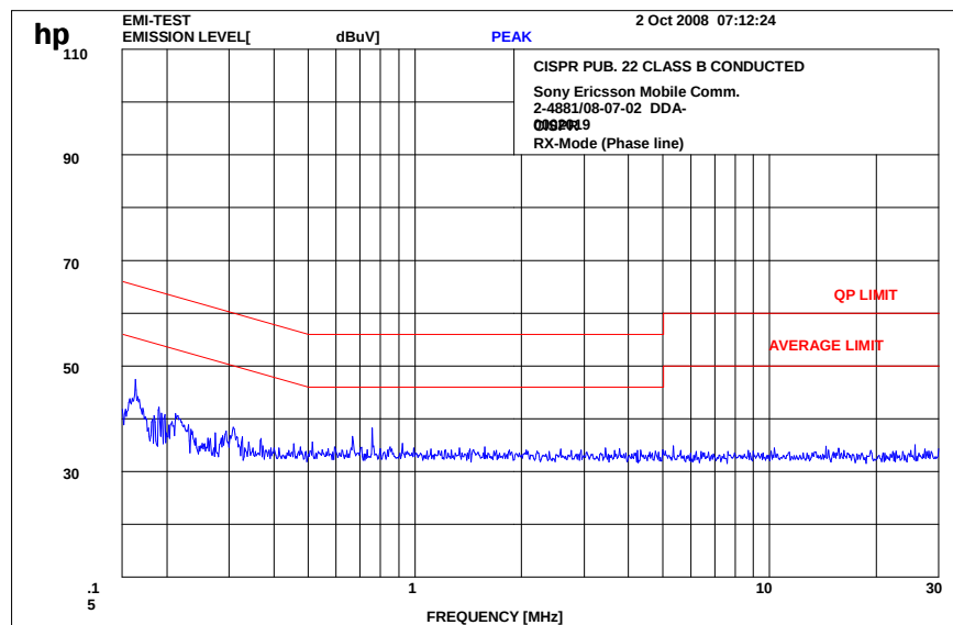
Plot 4: RX-Mode (Phase line); valid for all modulations
