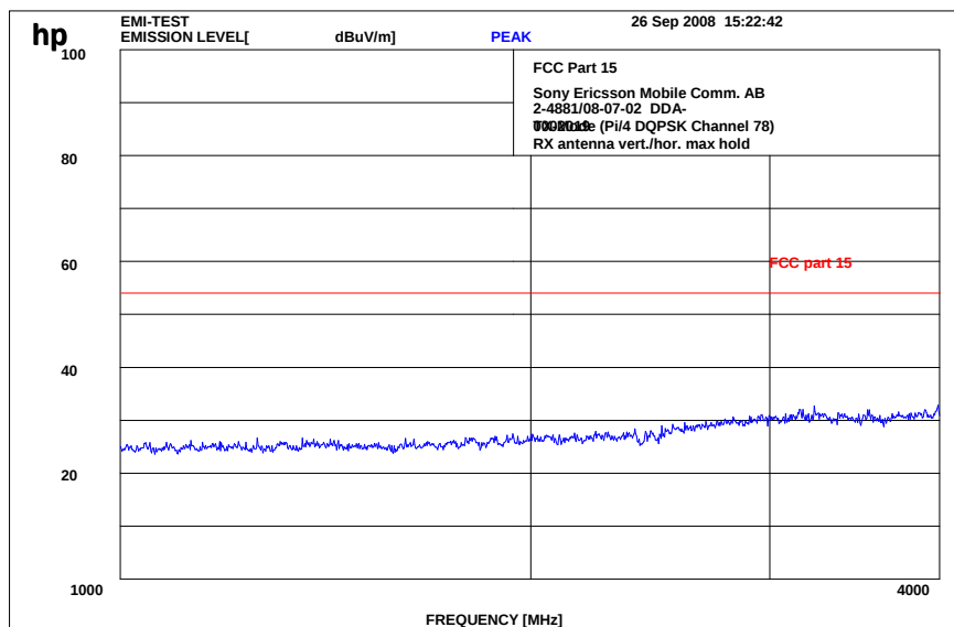
Plot 9: 1 - 4 GHz vertical/horizontal (Pi/4 DQPSK - highest channel)
