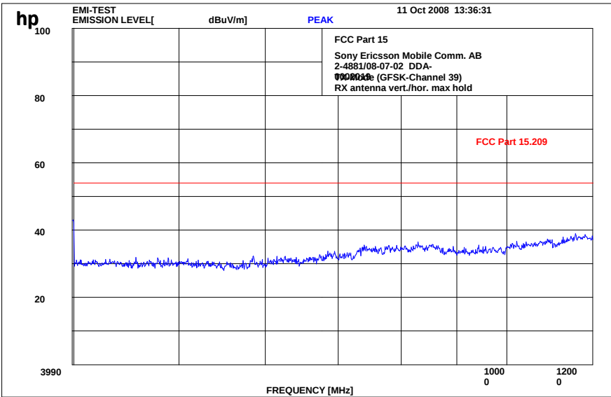
Plot 7: 4 - 12 GHz vertical/horizontal (GFSK - middle channel)
