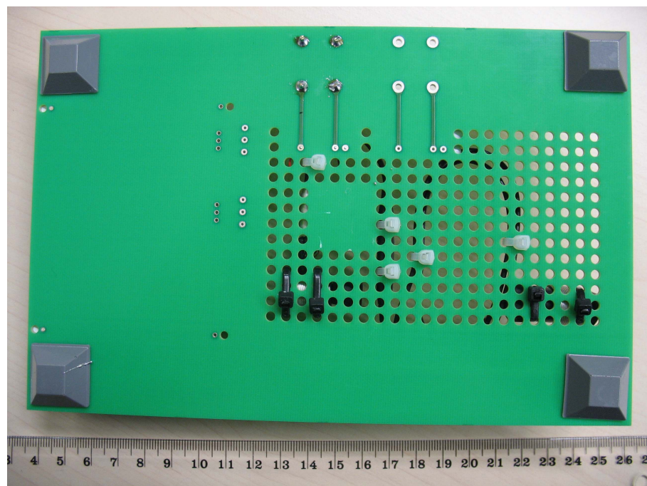
Photo 2: EUT mounted on a test board
