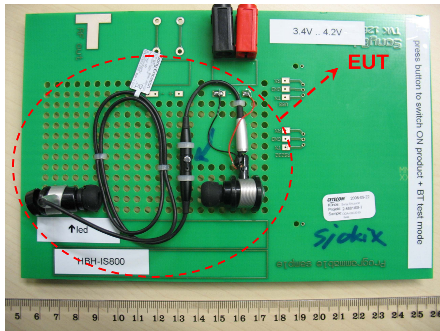
Photo 1: EUT mounted on a test board
