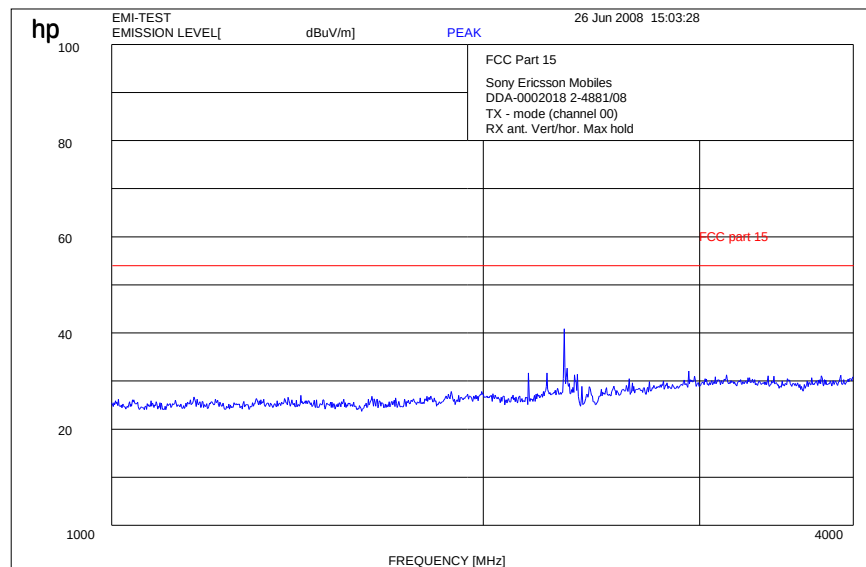
Plot 2: 1 - 4 GHz vertical/horizontal (lowest channel)
