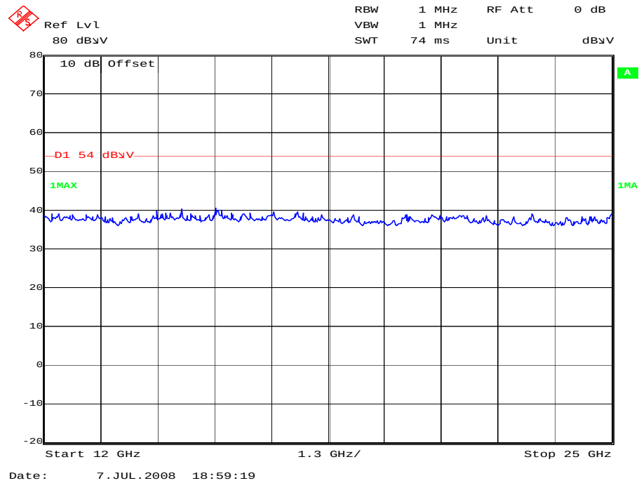
Plot 4: 12 - 25 GHz vertical/horizontal (valid for all channels)
