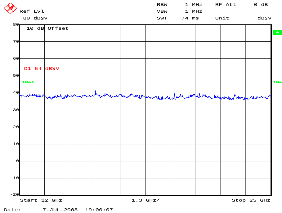
Plot 4: 12 - 25 GHz vertical/horizontal (receiver)
