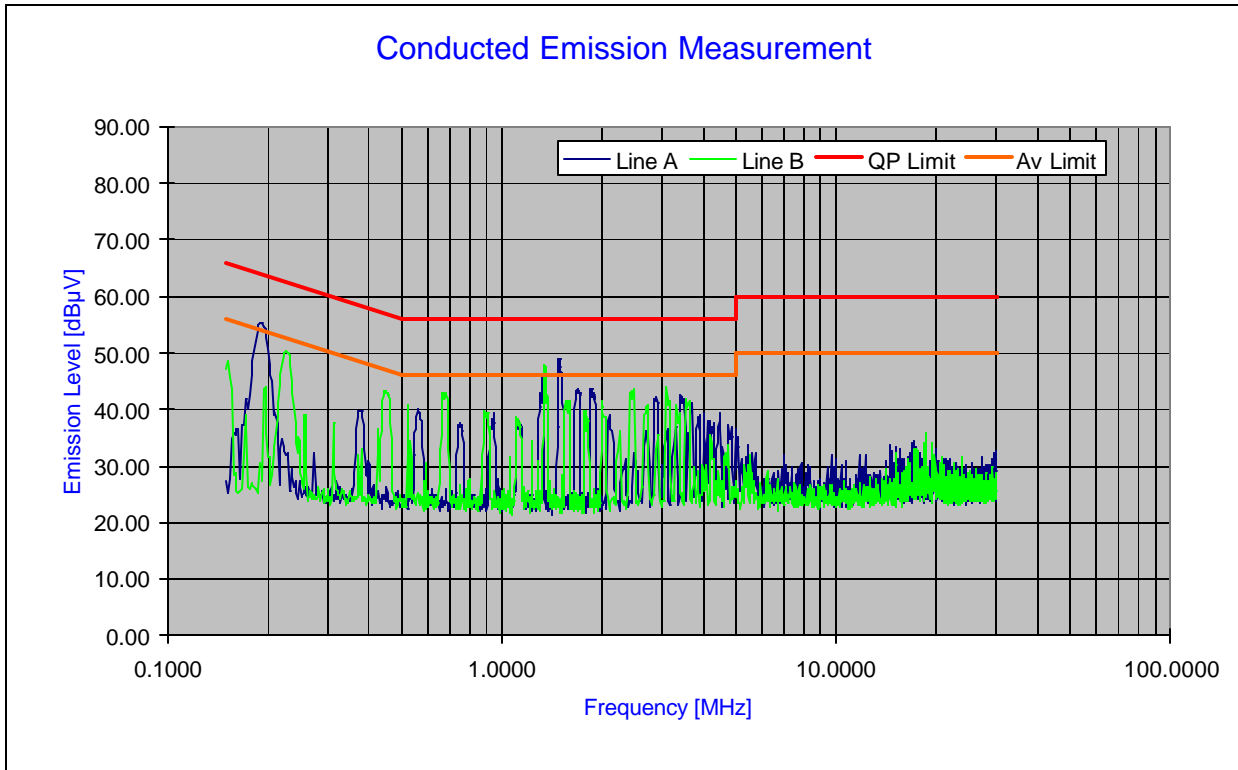
Plot 6-18. Line Conducted Plot with Bluetooth
