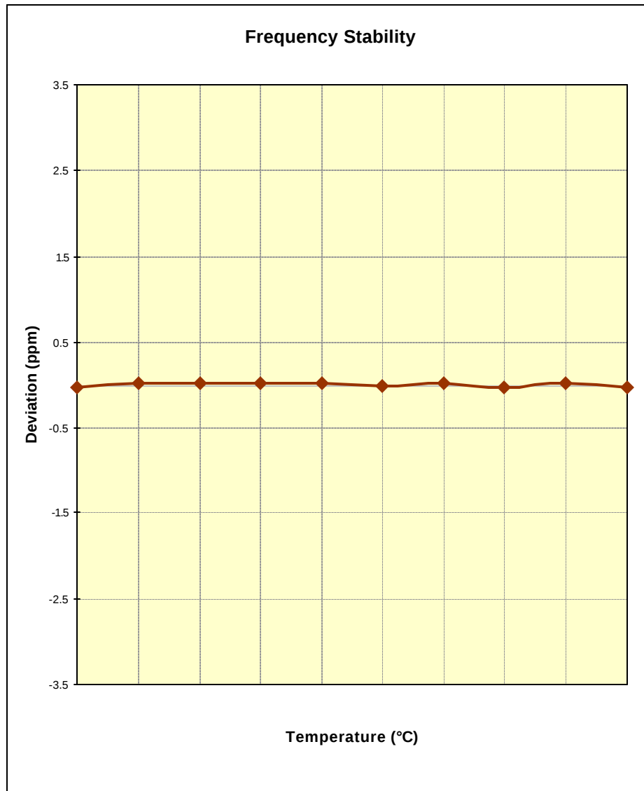
Plot 6-1. Frequency Stability Graph (Cellular CDMA Mode – Ch. 384)
