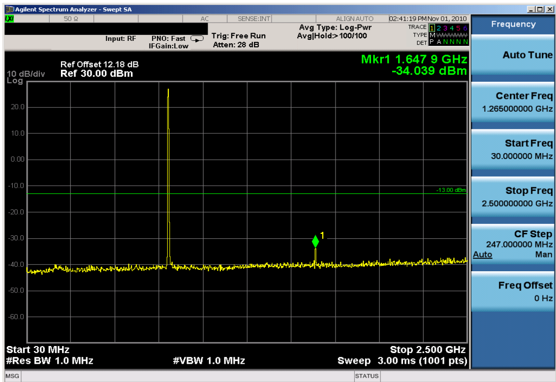
Plot 7-11. Conducted Spurious Plot (Cellular CDMA Mode – Ch. 1013)
