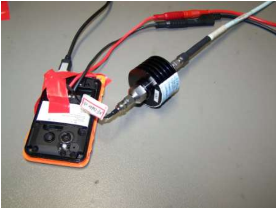
Photograph 1: Conducted test set-up: conducted RF-measurements
