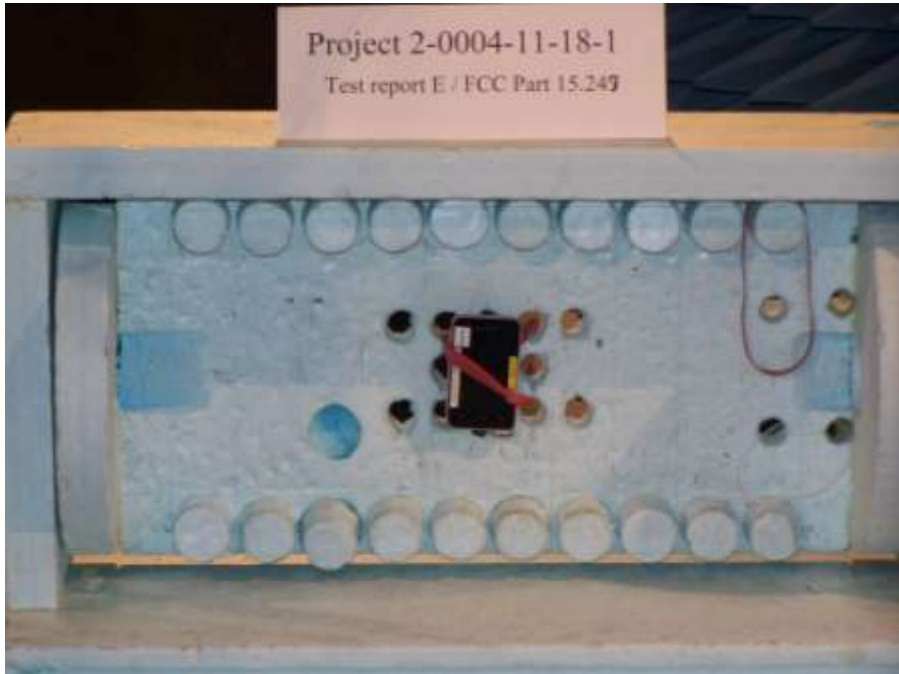
Photograph 2: Radiated test set-up: radiated RF-measurements
