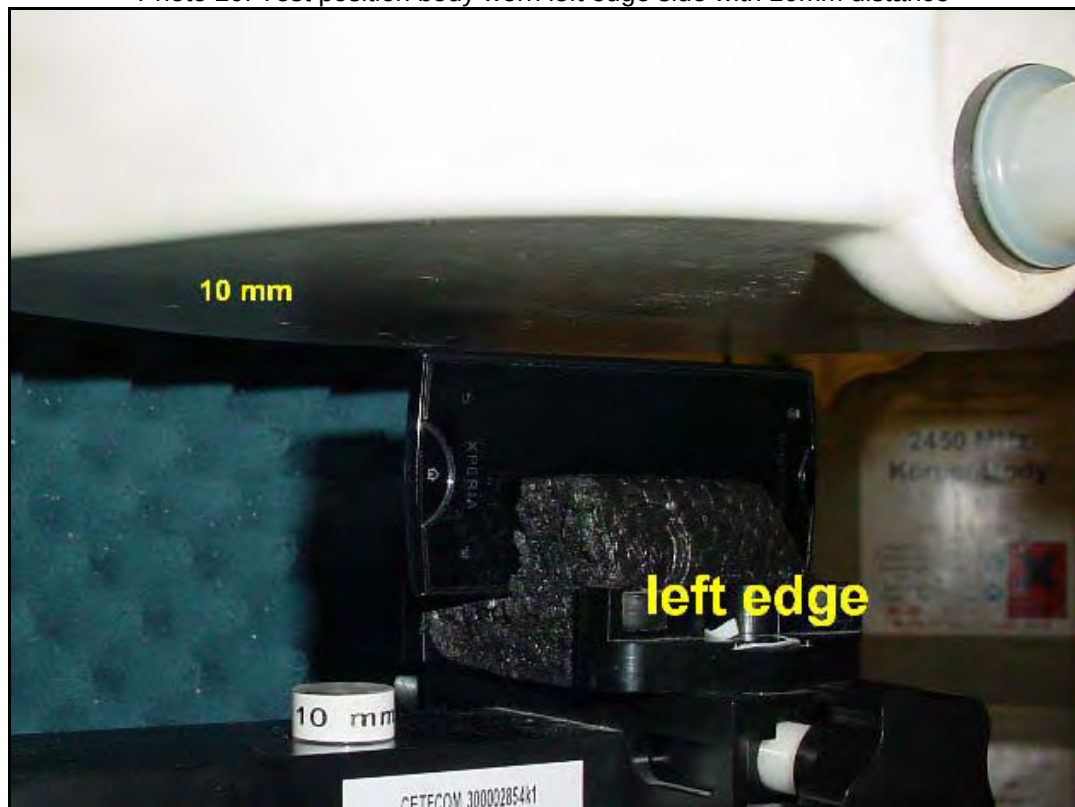
Photo 20: Test position body worn left edge side with 10mm distance
