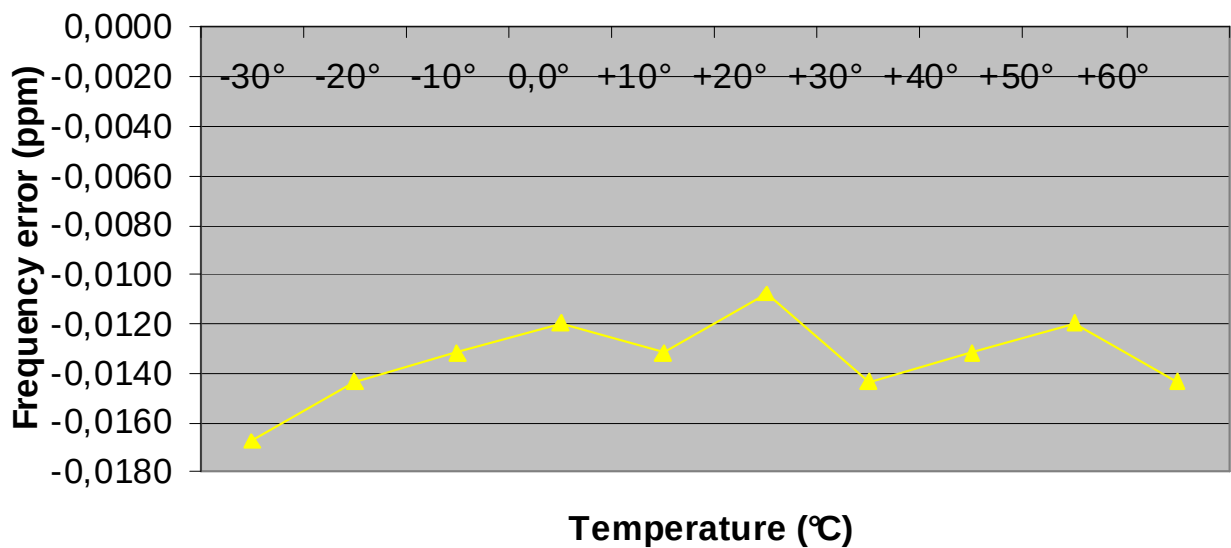
Frequency Error vs. Temperature
