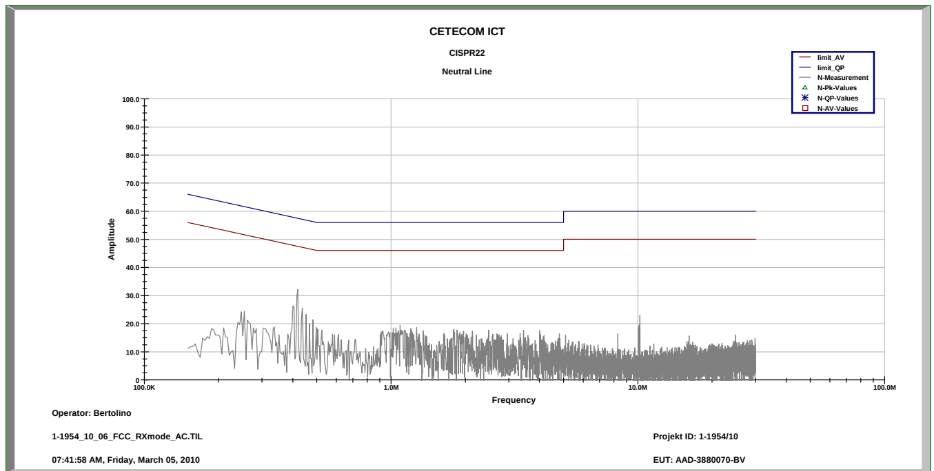
Plot 3: RX mode, neutral line
