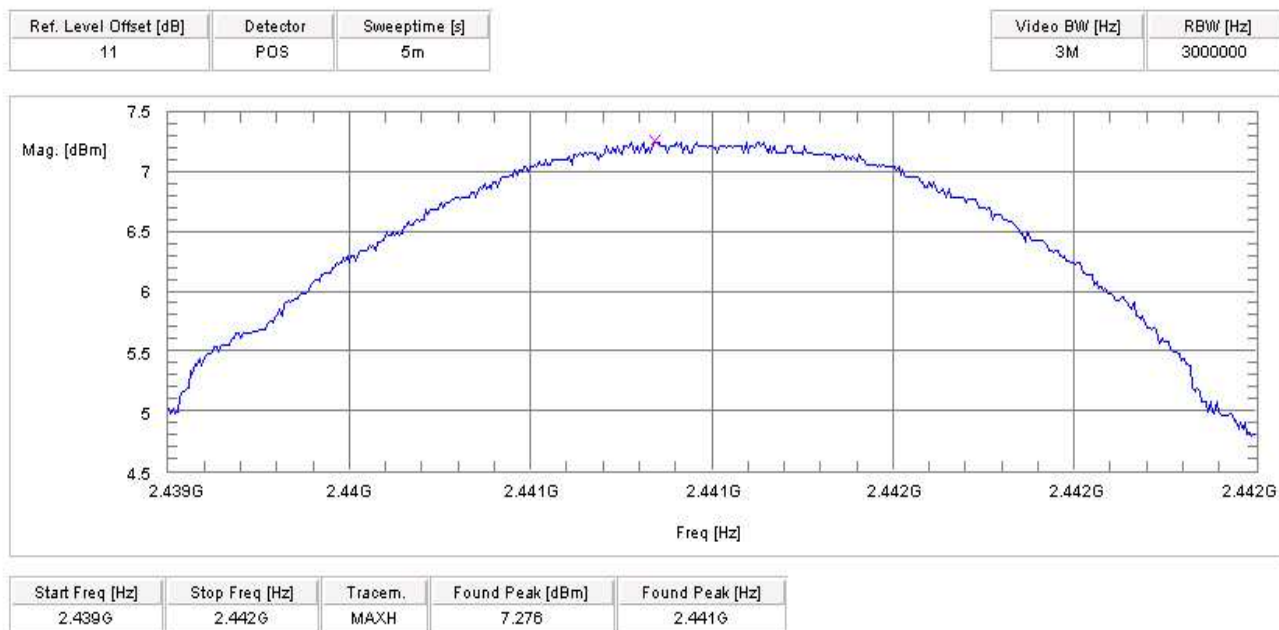
Plot 5: Pi/4 DQPSK, mid channel (39)
