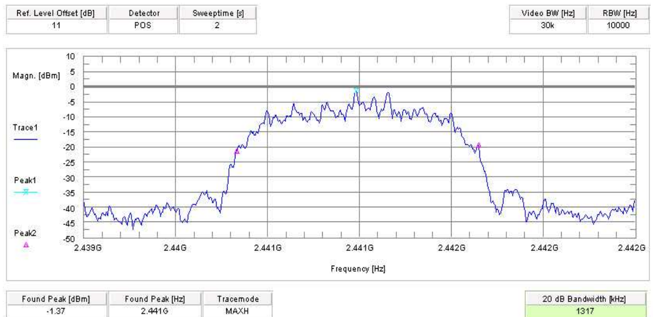
Plot 5: Pi/4 DQPSK, mid channel (39)
