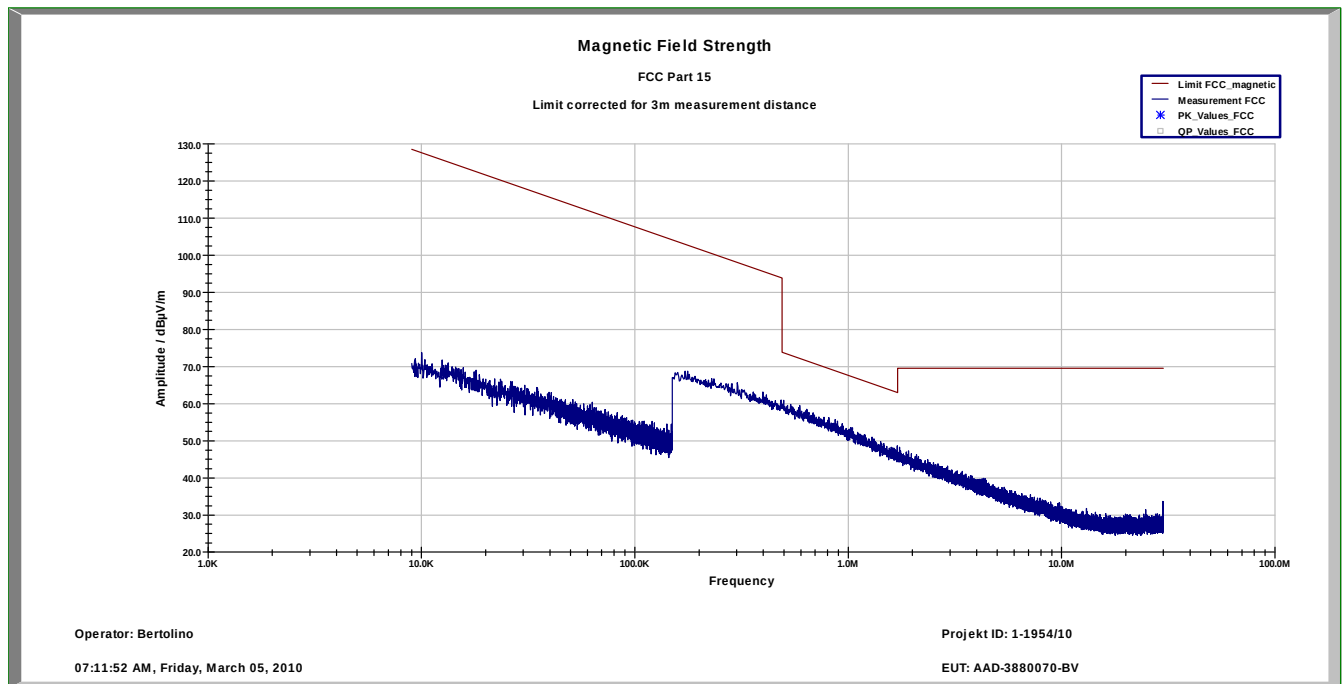
Plot 1: TX mode
