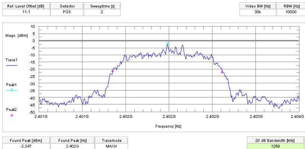
Plot 7: 8DPSK, low channel (00)
