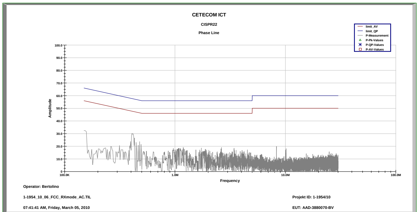
Plot 4: RX mode, phase line
