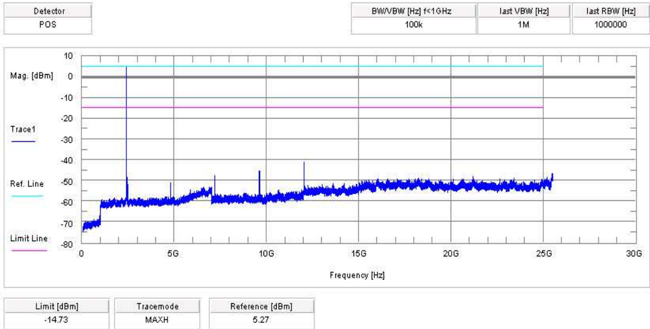
Plot 1 of 3: lowest channel (00)
