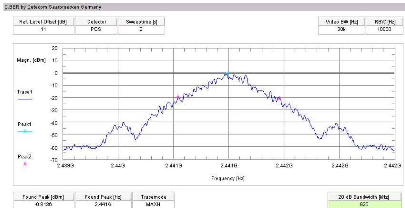
Plot 2: GFSK, mid channel (39)
