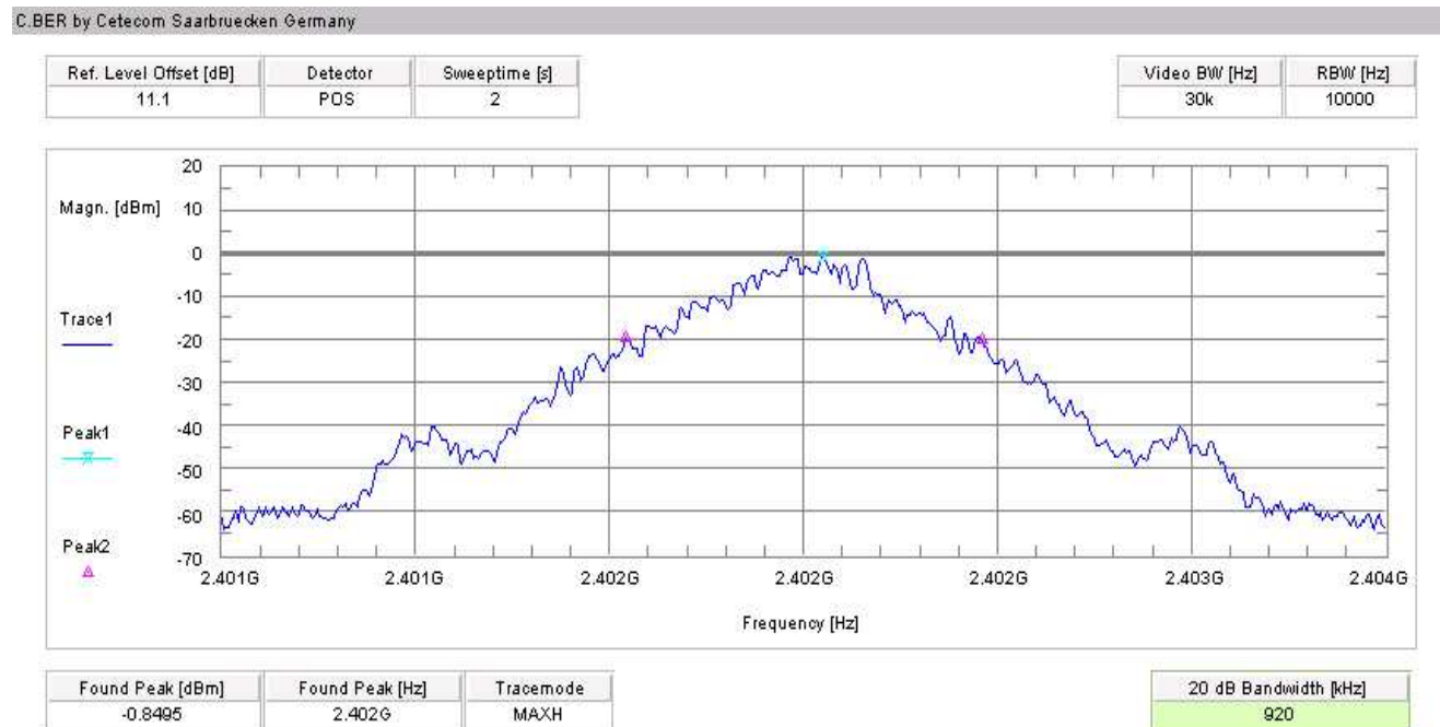
Plot 1: GFSK, low channel (00)
