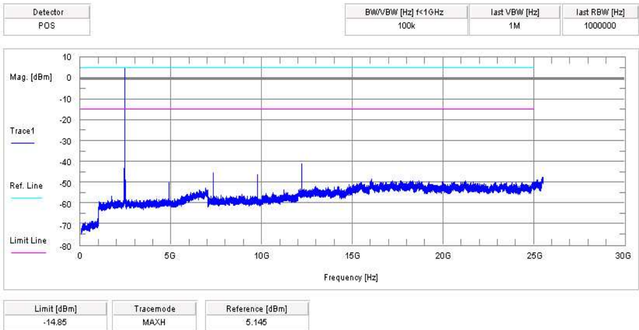
Plot 2 of 3: middle channel (39)
