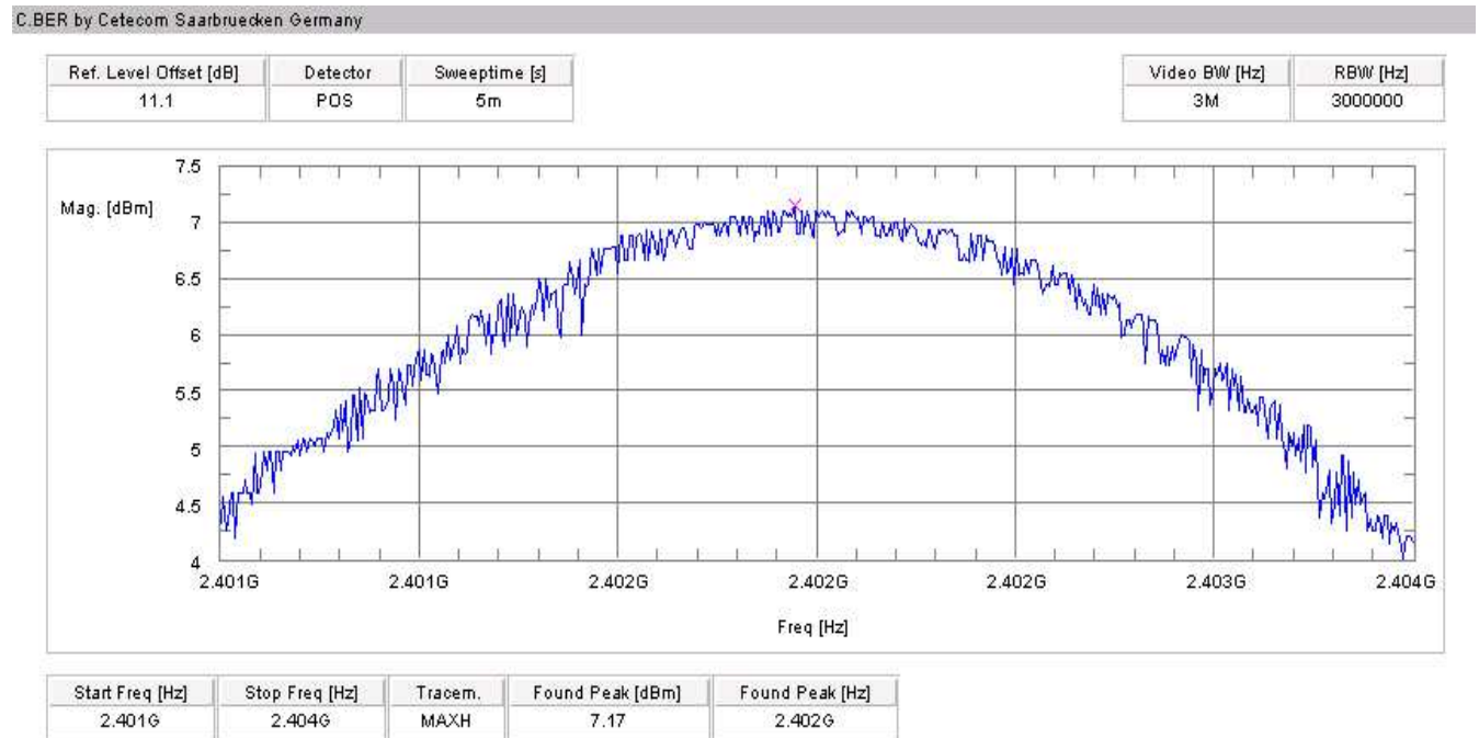
Plot 7: 8DPSK, low channel (00)
