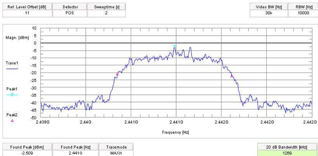
Plot 8: 8DPSK, mid channel (39)
