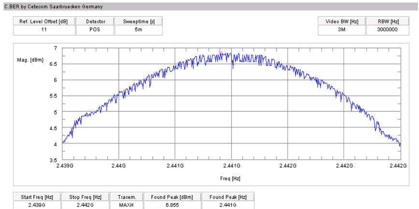
Plot 8: 8DPSK, mid channel (39)
