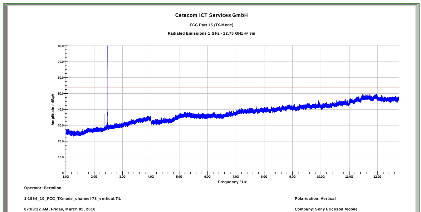
Plot 9: 1 – 12.75 GHz vertical polarization (highest channel)
