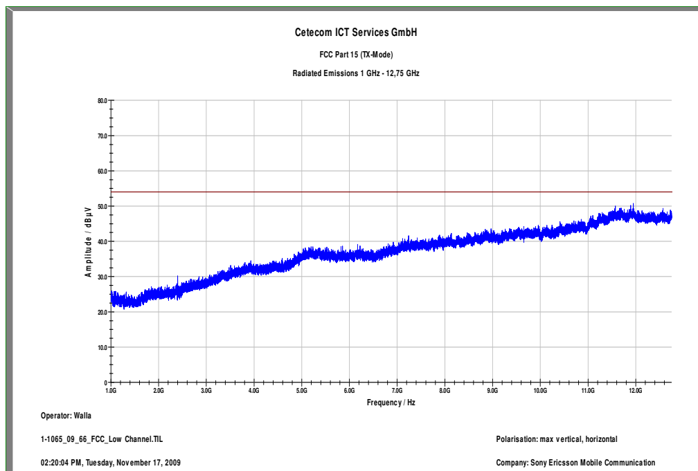
Plot 2: 1 - 12 GHz vertical/horizontal (lowest channel) @ 3 m
