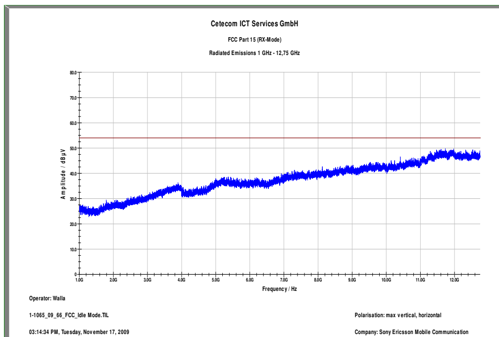
Plot 2: 1 - 12 GHz vertical/horizontal (receiver) @ 3 m
