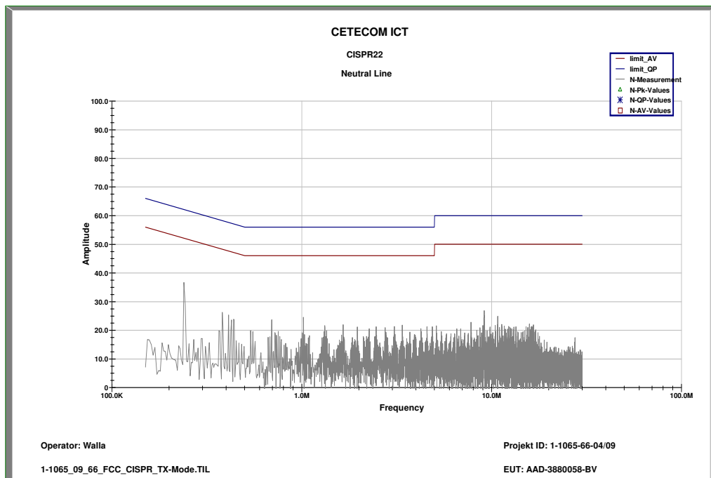
Plot 2: TX-Mode (Neutral Line)
