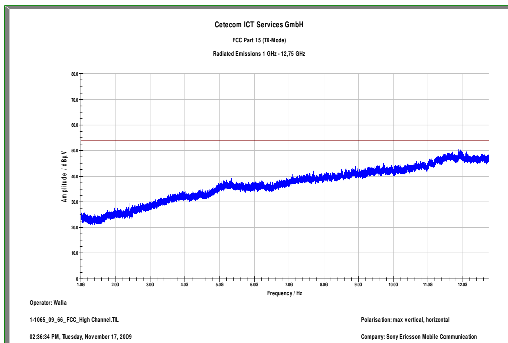
Plot 7: 1 - 12 GHz vertical/horizontal (highest channel) @ 3 m
