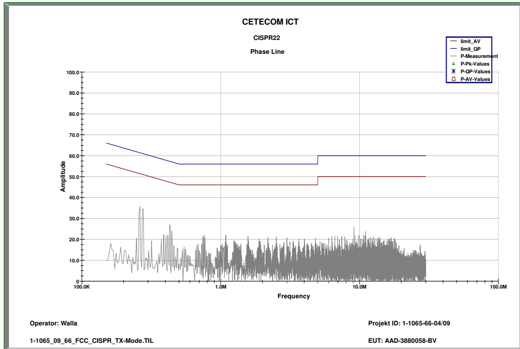
Plot 1: TX-Mode (Phase Line)
