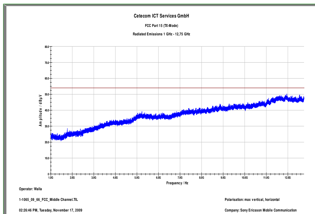
Plot 5: 1 - 12 GHz vertical/horizontal (middle channel) @ 3 m
