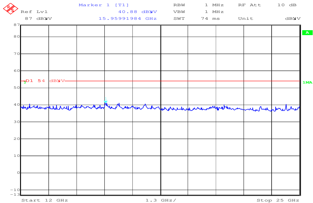
Plot 3: 12 - 25 GHz vertical/horizontal (valid for all channels)
