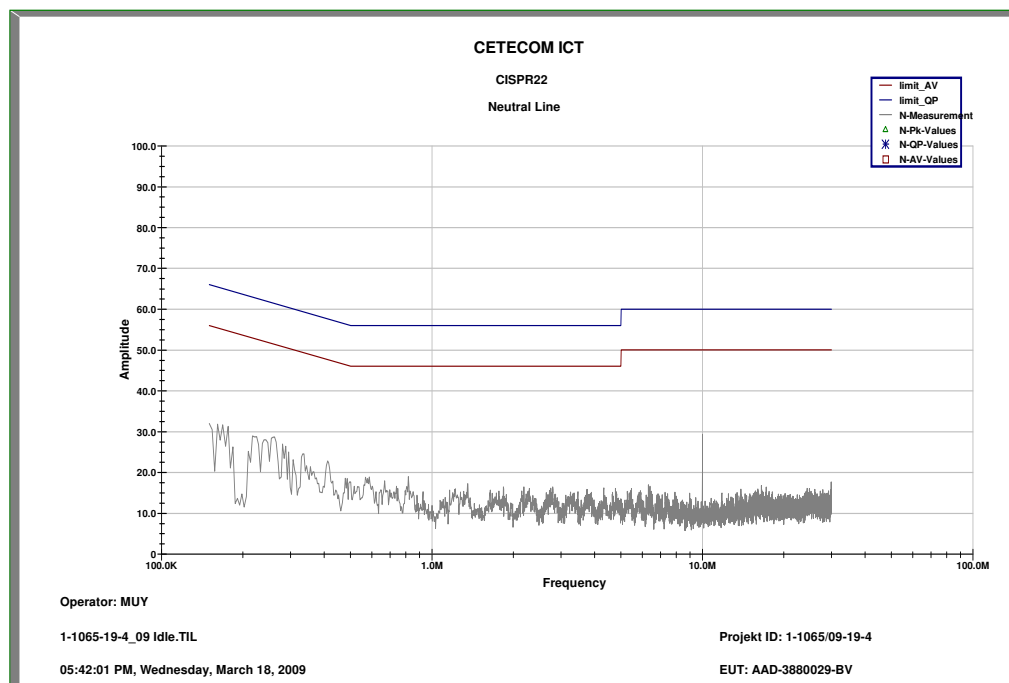
Plot 3: Neutral line, Idle
