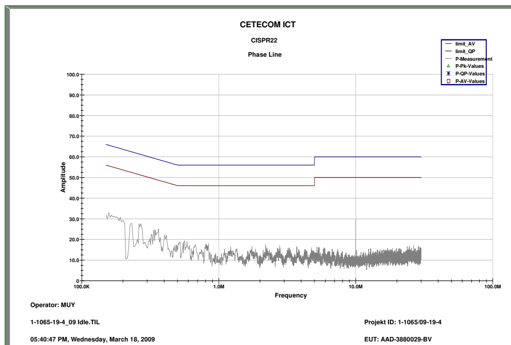
Plot 4: Phase line, Idle
