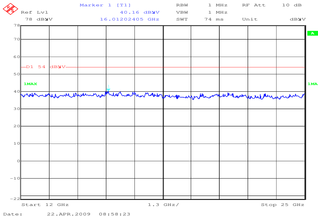
Plot 3: 12 - 25 GHz vertical/horizontal (receiver)
