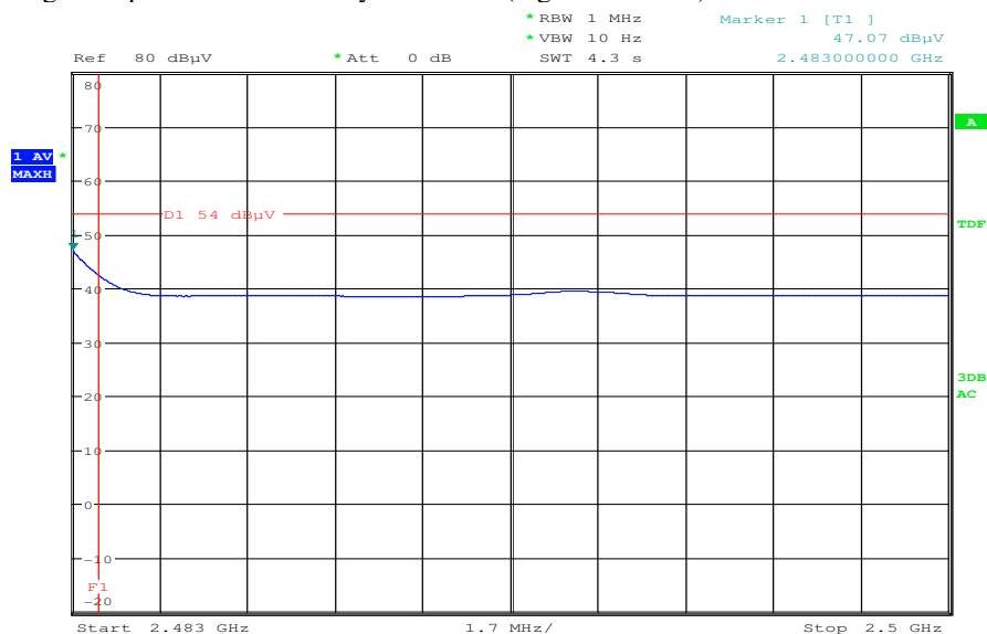
Plot 1: Band-edge compliance and far away emissions (highest channel)
