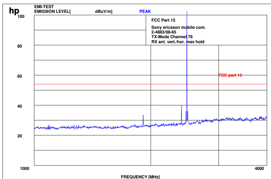
Plot 9: 1 - 4 GHz vertical/horizontal (highest channel)
