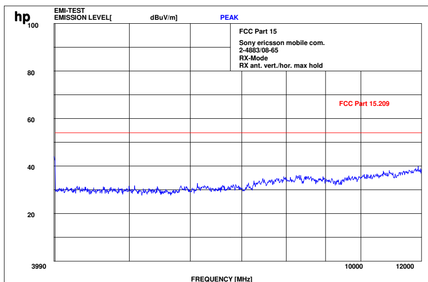
Plot 3: 4 - 12 GHz vertical/horizontal (receiver)
