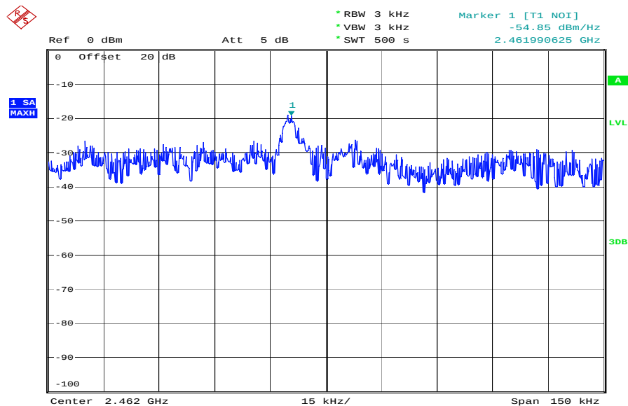
Plot 3: (result calculated by the Signal analyzer FSU from Rohde & Schwarz)
