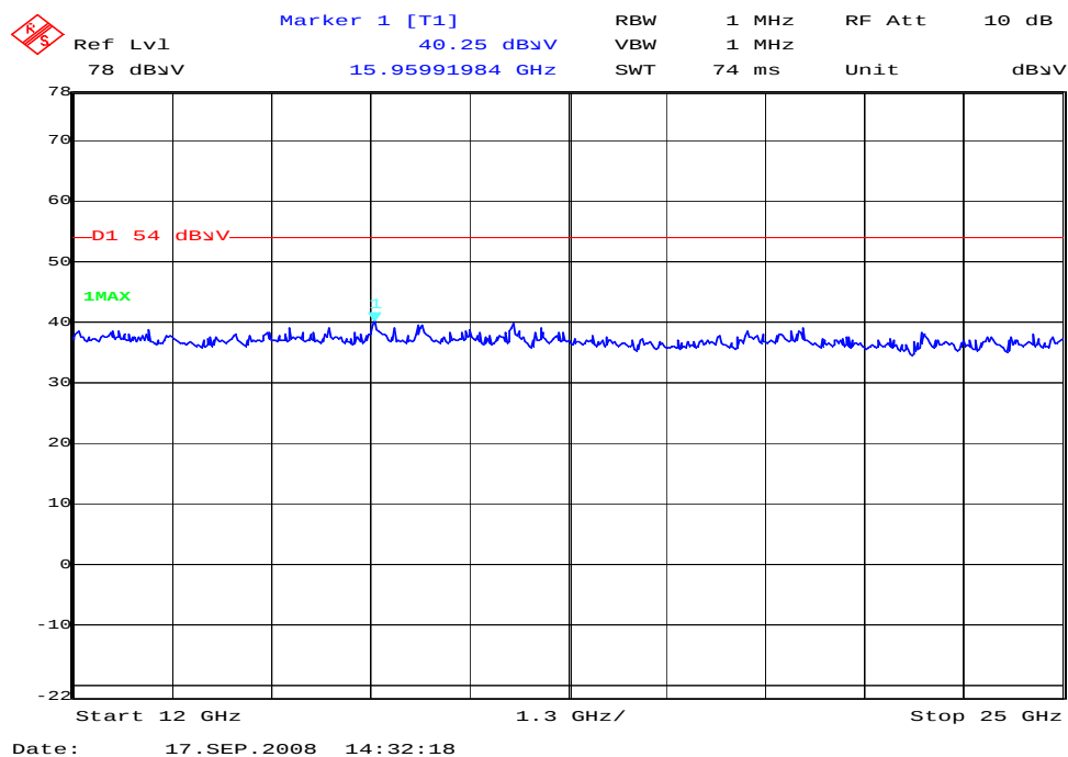
Plot 4: 12- 25 GHz (valid for all channels)
