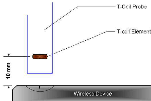
Figure 5-11 Measurement Distance
